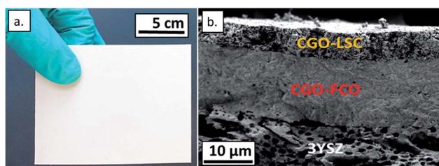
Fig. 12 Post-sintered picture (a) and SEM image of a fractured cross-section (b) of a planar dual-phase membrane component made from \text{Ce}_{0.8}\text{Gd}_{0.2}\text{O}_{2-\delta}-\text{FeCo}_2\text{O}_4 . The post-sintered picture of the membrane was taken on the 3YSZ porous support side.
