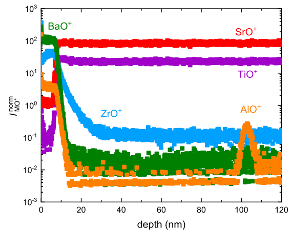
FIG. 5. Secondary ion intensities of \text{MO}^+ normalized to that of \text{O}^+ obtained by ToF-SIMS depth profiling for a \text{BaZrO}_3/\text{SrTiO}_3/\text{SrTiO}_3 sample prior to diffusion annealing (zero-time sample).
