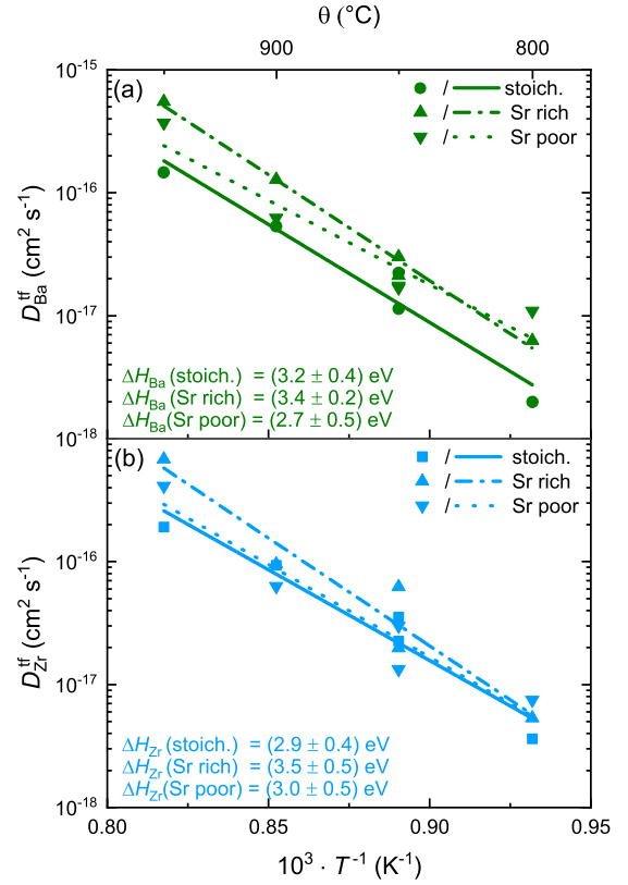
FIG. 8. Diffusion coefficients of Ba and Zr for the faster diffusion process in thin films of \text{SrTiO}_3 with differing Sr/Ti ratios as a function of inverse temperature.
