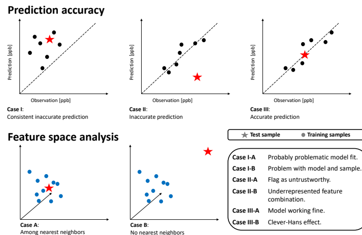
Figure 5. Schematic overview of possible cases. The upper columns show the predictions on k-nearest neighbors training samples and the target test sample with respect to the prediction error. The lower columns depict the k-nearest neighbor analysis in the feature space. Dots represent training samples, while stars depict the test sample.
