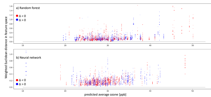
Figure 9. Plots showing inaccurate predictions (absolute values of \Delta > 5 ppb) on the test set by the random forest (a) and neural network (b). The weighted Euclidean distance in the respective feature space is on the y-axis. On the x-axis, the predicted average ozone is shown. The colors indicate the residual: red points mean negative residuals and model overestimation, while blue points show positive residuals and model underestimation. The size of the single dots points to the distance between the test sample and the training sample in the representation space. A larger dot means that the test sample and respective training sample lead to similar activation patterns in the model.
