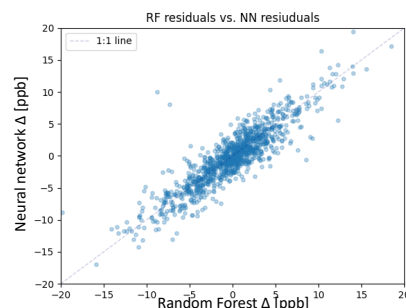
Figure 6. Scatter plot of the residuals \Delta of the random forest on the x-axis and neural network on the y-axis for the test set.
