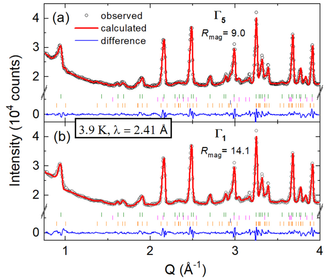
FIG. 8. The fitting results to the higher-resolution NPD patterns of \text{RbEu}(\text{Fe}_{0.95}\text{Ni}_{0.05})_4\text{As}_4 collected at 3.9 K with \lambda = 2.41 Å, adopting the in-plane helical magnetic structure described by (a) \Gamma_5 and the c -axis spin-density-wave-type magnetic structure described by (b) \Gamma_1 , respectively. The circles represent the observed intensities, and the solid lines are the calculated patterns. The differences between the observed and the calculated intensities are shown at the bottom. The vertical bars in olive, magenta, navy, and orange colors indicate the expected nuclear Bragg reflections from the \text{RbEu}(\text{Fe}_{0.95}\text{Ni}_{0.05})_4\text{As}_4 main phase, FeAs impurity, vanadium sample container, and the magnetic Bragg reflections from \text{RbEu}(\text{Fe}_{0.95}\text{Ni}_{0.05})_4\text{As}_4 , respectively.
