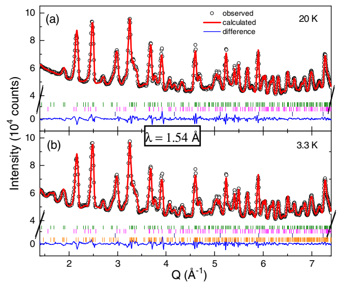
FIG. 4. NPD patterns of \text{RbEu}(\text{Fe}_{0.93}\text{Ni}_{0.07})_4\text{As}_4 at (a) 20 K and (b) 3.3 K collected using the incident neutron wavelength of 1.54 \text{ \AA} and the Rietveld refinements. The pattern in (b) is the refinement result obtained by adopting a magnetic-structure model with the irreducible representation \Gamma_5 as described in the text. The circles represent the observed intensities, and the solid lines are the calculated patterns. The differences between the observed and the calculated intensities are shown at the bottom. The vertical bars in olive, magenta, navy, and orange colors indicate the expected nuclear Bragg reflection from \text{RbEu}(\text{Fe}_{0.93}\text{Ni}_{0.07})_4\text{As}_4 , FeAs impurity, vanadium sample container, and the magnetic Bragg reflection from \text{RbEu}(\text{Fe}_{0.93}\text{Ni}_{0.07})_4\text{As}_4 , respectively.
