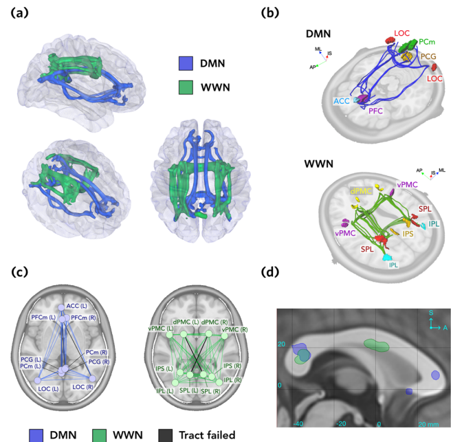
Fig. 3 Tract trajectories for DMN and WWN. a All accepted tracts shown for the DMN (blue) and WWN (green) networks, rendered as isosurfaces thresholded at 0.5 (top, right, and oblique perspectives). b Core polylines representing the trajectories of accepted tracts in the DMN (top) and WWN (bottom) networks. Images are rendered with oblique perspectives next to planar sections of the ICBM nonlinear T1 template image, for reference. See Materials and Methods for names of the ROIs. c Graph representations of the DMN (blue) and WWN (green) networks, with failed edges shown in grey. Graph vertices represent the centre points of each ROI, projected onto the transverse plane. d Sagittal section at midline, showing where contralateral tracts (thresholded at 0.5) for each network traverse the corpus callosum. Coordinates are ICBM152. Axis labels: ML medial-lateral, AP anterior-posterior, IS inferior-superior.
