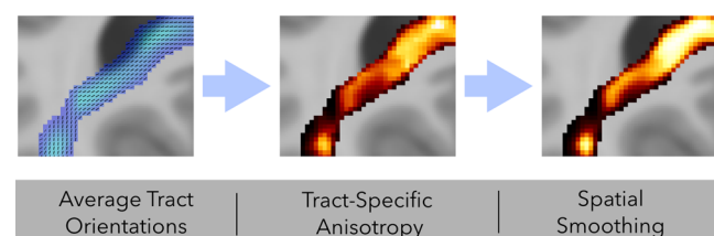
Fig. 1 Schematic of the procedure. Probabilistic tractography: ROIs were obtained from previous meta-analytic studies and used as seed/target regions for diffusion tensor modelling with bedpostx and probabilistic tract tracing performed with probtrackx , across all participants. The resulting probability distributions were averaged across directions for each ROI pair ( P_{ab} ). Tract trajectory estimation: For each ROI pair, a “core” trajectory was estimated from these bidirectional averages, and represented as a 3-dimensional polyline. An uncertainty field ( \Phi_{ab} ) was then generated from this polyline using an anisotropic Gaussian kernel. Finally, a “core” tract estimate ( P_{ab-tract} ) was generated as the element-wise product of P_{ab} and \Phi_{ab} . Tract-specific anisotropy: Average tract orientations were computed for each voxel in a given tract, and these orientations were then regressed against the diffusion evidence for each individual participant. This produced a tract-specific anisotropy (TSA) distribution for each participant, that can be regressed against variables of interest.
