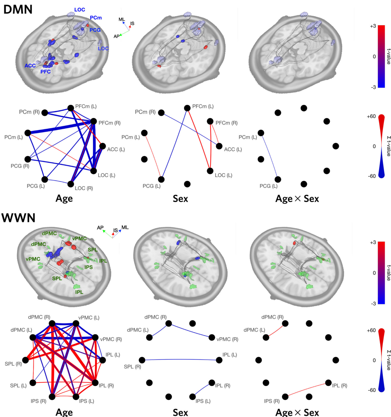
Fig. 5 Age and sex effects for DMN and WWN. Regression results are shown for both networks, for linear models of the form TSA = Age + Sex + Age \times Sex + \epsilon . 3D renderings show the maximal t -values (thresholded using cluster-wise inference, with p < 0.05 and FDR < 0.05 ) at each distance along the core trajectories of each tract in the network. Circular graph representations show the sum of significant positive (red) and negative (blue) t -values for each tract. The thickness of an edge is proportional to its sum, and the absence of an edge indicates that no significant clusters were found for that tract. In all cases, N = 130 . Axis labels: ML medial-lateral, AP anterior-posterior, IS inferior-superior.
