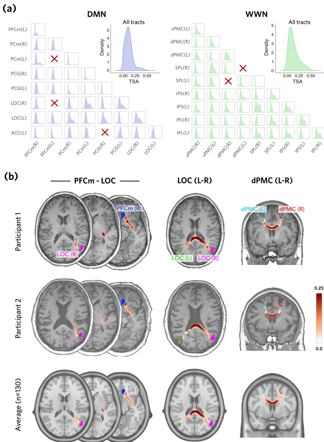
Fig. 4 Tract-specific anisotropy (TSA). a Distributions of TSA across voxels and participants, for each estimated tract (ROI pair), shown as kernel density estimates for DMN (blue) and WWN (green). Insets show the distribution of TSA values over all tracts; x-axis scales are the same for all plots. Red crosses indicate that no tract was generated. b Spatial distributions of TSA values for two exemplar participants and averaged over all participants, and three exemplar tracts, shown in horizontal and coronal section. Anatomical images are the ICBM152 nonlinear template.
