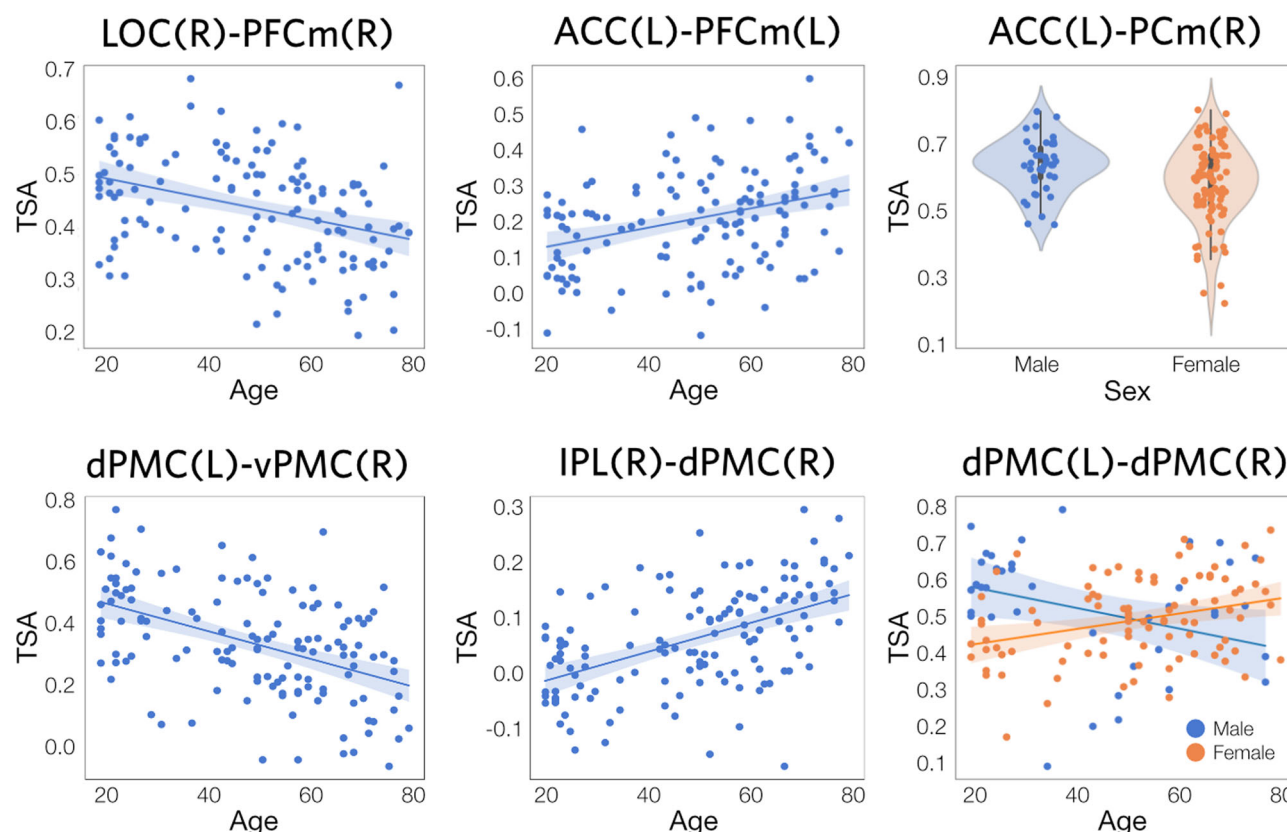
Fig. 6 Scatter and violin plots of age and sex effects. Plots of selected TSA regression results are shown ( N = 130 ). Top row: DMN tracts with (from left to right) negative and positive age effects, and a sex difference (male > female). Bottom row: WVN tracts with negative and positive age effects, and an Age \times Sex interaction. Data points are the mean TSA values within significant clusters (as shown in Fig. 5). Shaded areas on scatterplots represent 95% confidence intervals.
