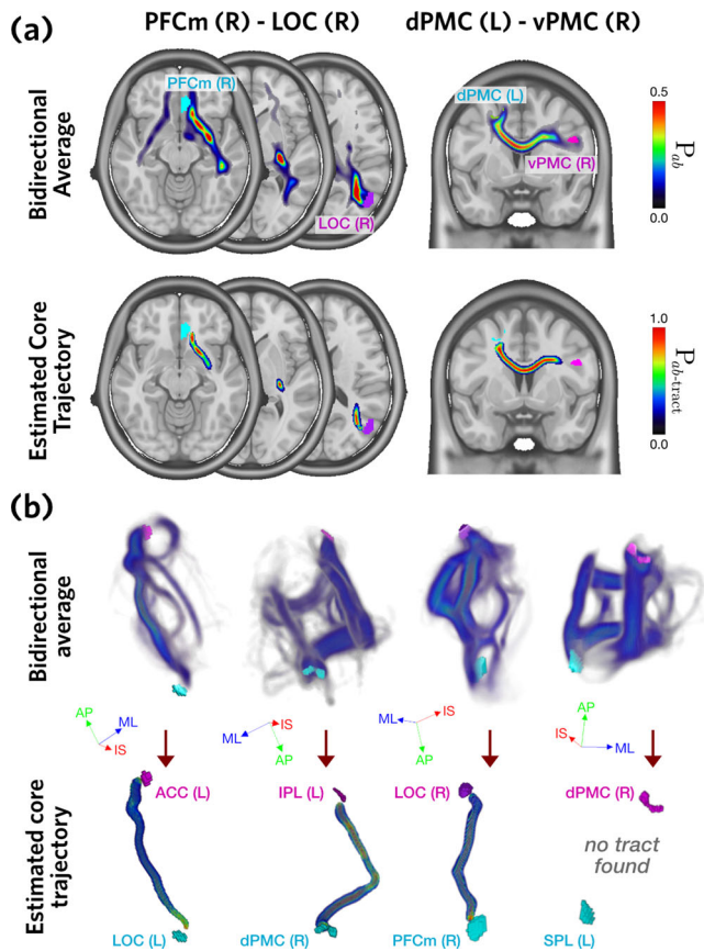
Fig. 2 Tract trajectory estimation. a Core tract trajectory estimation steps, shown for two exemplar tracts. The top row shows the streamline probability determined across all participants ( n = 130 ), averaged in both directions, P_{ab} . The bottom row shows the estimated core trajectory for each ROI pair, P_{ab-tract} . b Three-dimensional distributions of P_{ab} (top) and P_{ab-tract} (bottom), for four exemplar tracts. Axis labels: ML medial-lateral, AP anterior-posterior, IS inferior-superior.
