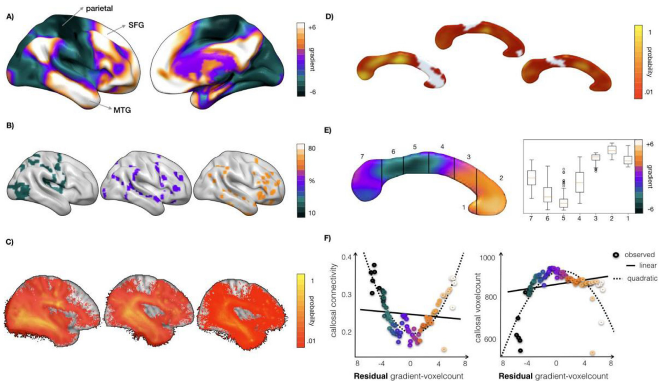
Fig. 2. Mapping the principal gradient on the corpus callosum. A) Visualisation of the principal gradient on the cortical surface. B) Examples for percentage maps (20–40–60%) depicting associated cortical areas. C) Percentage-specific tractograms as derived from the percentage gradients maps shown in B. D) Midsagittal display of callosal connectivity based on the tractograms for the 20th, 40th and 60th gradient percentages. Callosal areas with low probabilities (red) indicate that fewer participants showed connections to the particular gradient percentage in this area. The prevalence across gradient values for 12 exemplary voxels is depicted in supplementary figure S1-A. E) Callosal gradient map (left), which was computed as the weighted average of callosal connectivity across all percentage maps of the gradient with the 7 regions of the Wittelson parcellation superimposed. The distribution of gradient values along the Wittelson parcellation scheme is shown on the right. For a hard-border classification of voxels to gradient values please see supplementary figure S1-B. F) Scatterplots showing the relation between callosal connectivity (left) or number of non-zero connectivity voxels (right) and the residual between the gradient corrected for the number of voxels in the respective gradient percentage map. By callosal connectivity, we mean interindividual probability of connection.
