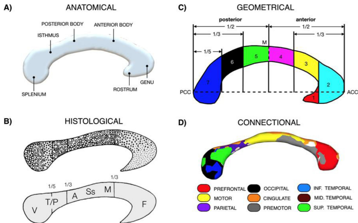
Fig. 1. Parcellations of the corpus callosum along the midsection (right view). A) Anatomical division: depicts the anatomical classification (rostrum, genu, anterior and posterior body, isthmus, splenium) based on gross anatomical features. B) Histological division: the dots in this schematic diagram indicate the range of axonal density and associate them with cortical projections to cortical areas (F: Frontal, M: Motor, SS: Somato-Sensory, A: Auditory, T/P: Temporo-Parietal and V: Visual (from Aboitiz and Montiel, 2003). C) Geometrical division: This parcellation generates seven parcels by equally dividing the midsection (from Wittelson, 1989). ACC: most anterior point of the corpus callosum, PCC: most posterior point of the corpus callosum, M: middle of the corpus callosum. D) Connectional division: Shows the parcellation of the cortex based on diffusion tractography (from Catani and Thiebaut de Schotten, 2012).
