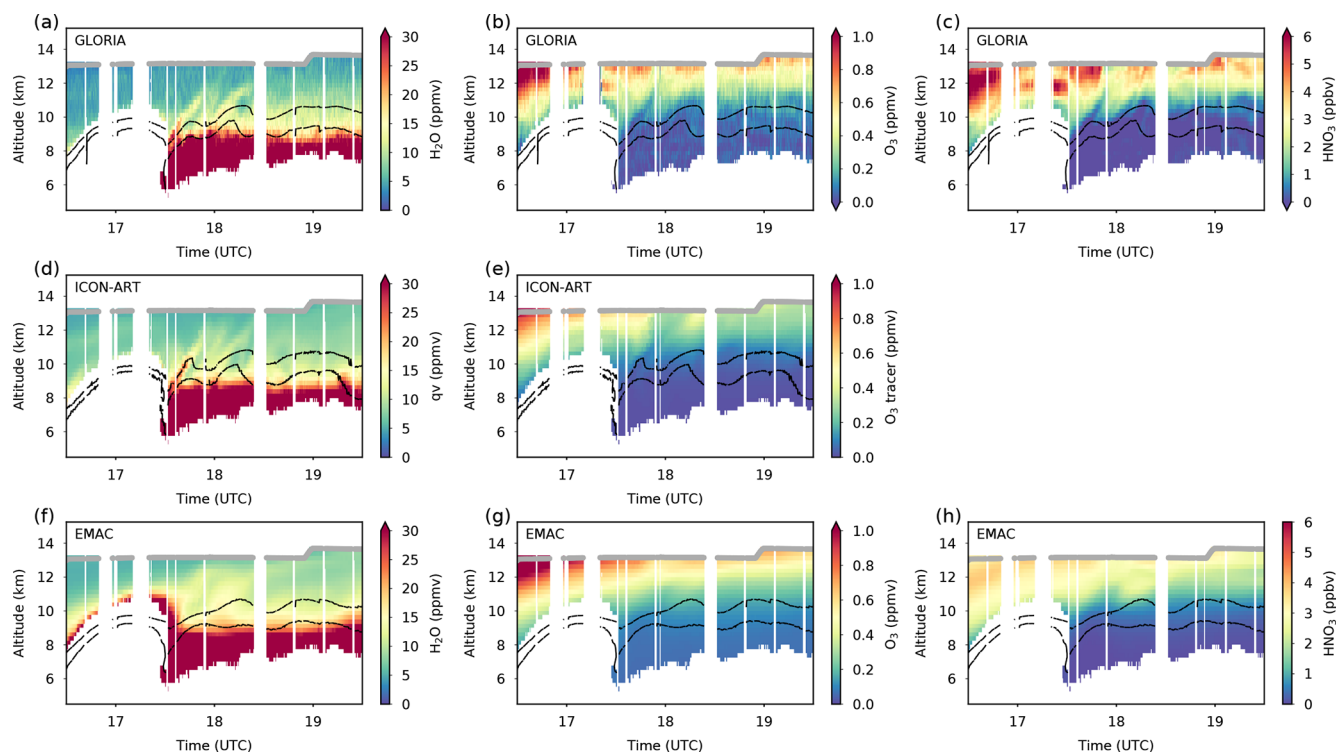
Figure 9. Close-ups of troposphere-to-stratosphere exchange region between 17:30 and 19:30 UTC. In the case of ICON-ART, the nested data are shown. For legend, see Fig. 7.
