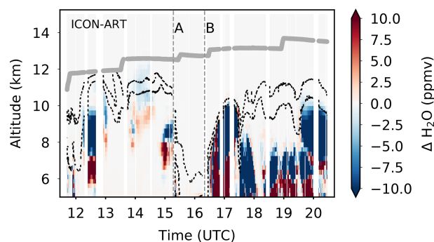
Figure 6. Modelled short-term changes in specific humidity due to cloud processes. Residuals between nested ICON-ART domain of specific humidity and corresponding \text{H}_2\text{O} tracer without cloud microphysics. Dashed black lines: ICON-ART 2 and 4 PVU isolines (lower and higher lines, respectively) as indicators for the dynamical tropopause. Grey lines: HALO flight altitude.
