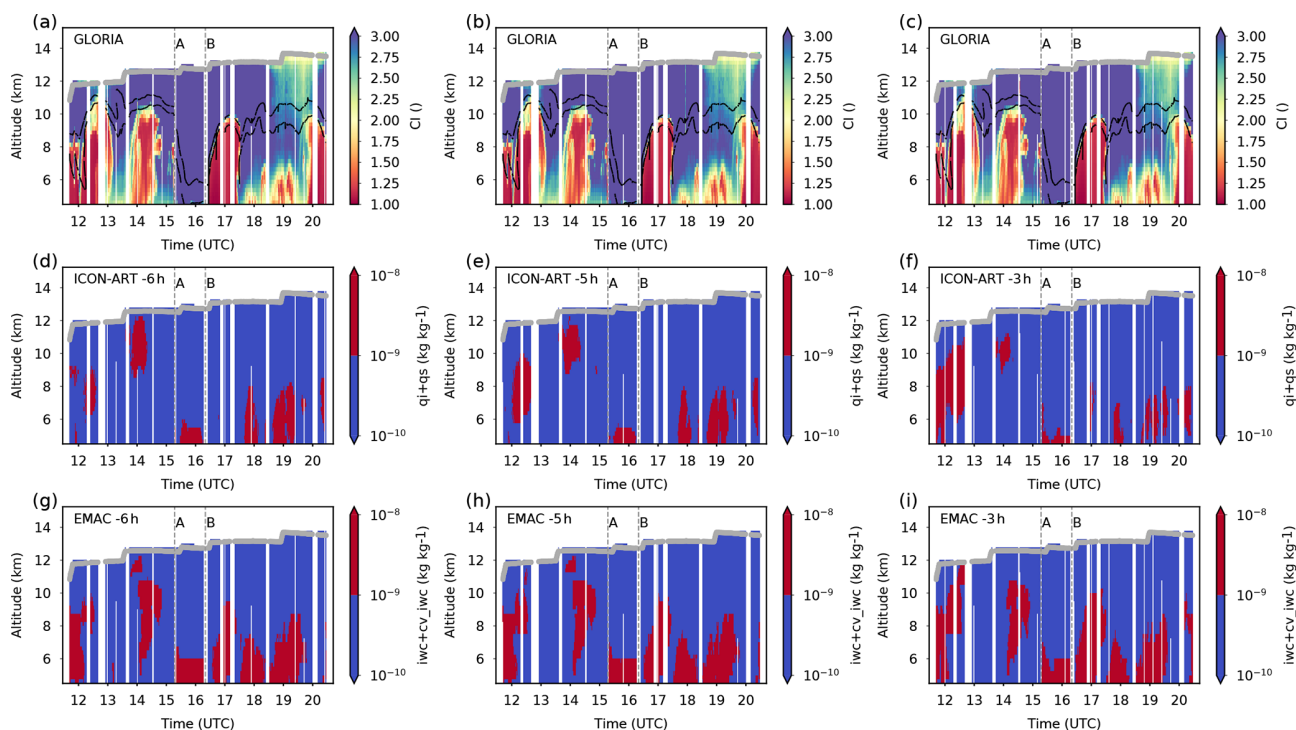
Figure A2. Same as Fig. 5, but model data (ICON-ART and EMAC) have been sampled with a constant time offset of -6 , -5 and -3 h during the interpolation to the GLORIA geolocations along the flight.
