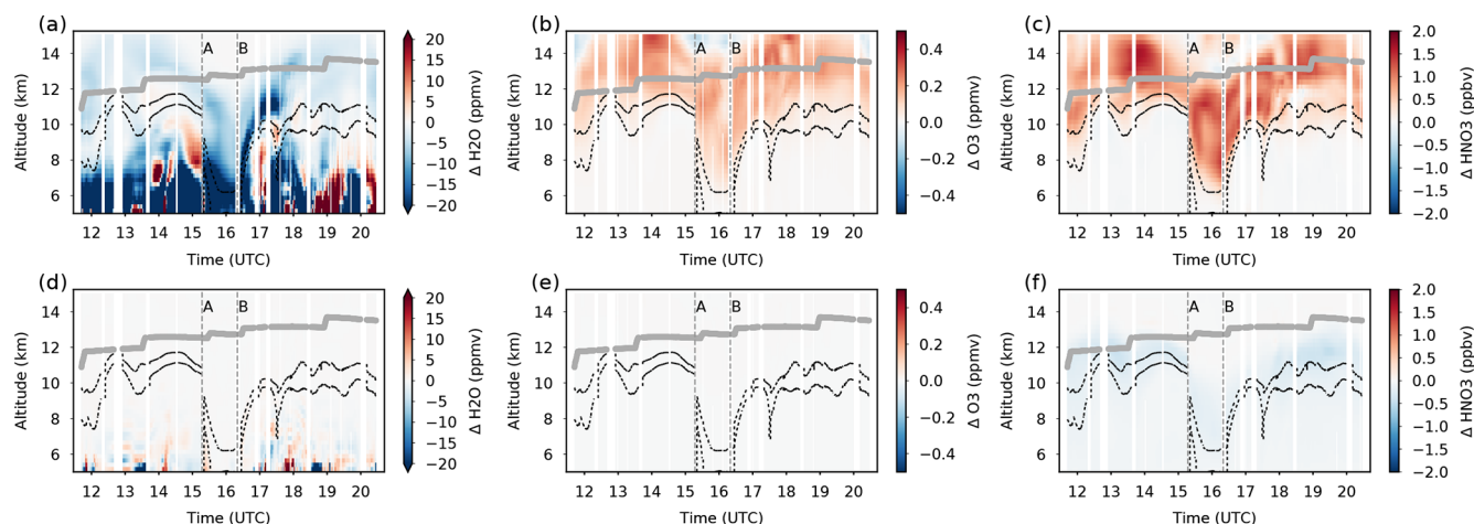
Figure 13. Modelled differences in \text{H}_2\text{O} , \text{O}_3 and \text{HNO}_3 due to lower resolution (a–c; T106 – T42 resolution) and neglecting scavenging processes in clouds (d–f; EMAC-STD – EMAC-NOSCAV). Dashed black lines: EMAC 2 and 4 PVU isolines (lower and higher lines, respectively) as indicators for the dynamical tropopause. Grey lines: HALO flight altitude.
