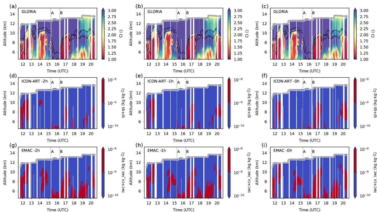
Figure A3. Same as Fig. 5, but model data (ICON-ART and EMAC) have been sampled with a constant time offset of -2 , -1 and 0 h during the interpolation to the GLORIA geolocations along the flight.
