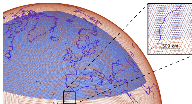
Figure 2. For the POLSTRACC winter, a global ICON-ART simulation with a global R2B6 grid was carried out (red). In the area of the flights, a nest with an R2B7 grid with \sim 20\text{ km} horizontal grid spacing was used to resolve mesoscale processes in more detail (blue).
