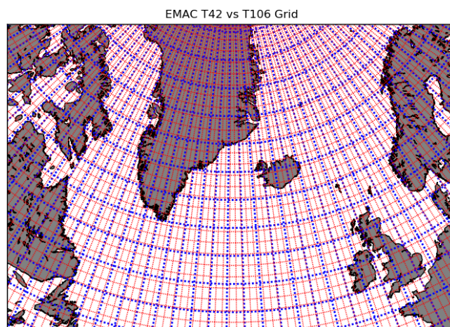
Figure 3. The EMAC standard and sensitivity simulations employed Eulerian grids with 106 (red) and 42 (blue) spectral coefficients. The T106 (T42) grid corresponds to a horizontal resolution of 125 km (310 km) at the Equator. Due to the grid convergence, the zonal grid spacing is reduced towards the poles and amounts to ~40 km (~110 km) at 70° N.
