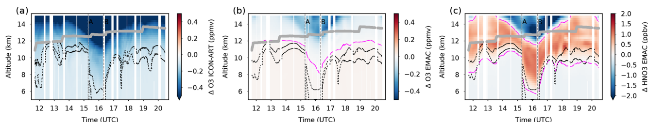
Figure 12. Modelled ozone depletion and changes in nitric acid due to chemical and microphysical processes. Residuals between (a) ICON-ART O 3 tracer and passive O 3 tracer, (b) EMAC O 3 and O 3 passive, and (c) EMAC HNO 3 and HNO 3 passive. Dashed black lines: ICON-ART and EMAC 2 and 4 PVU isolines (lower and higher lines, respectively) as indicators for the dynamical tropopause. Grey lines: HALO flight altitude. Magenta lines indicate the zero contour.
