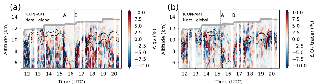
Figure 8. Residuals between the ICON-ART nested R2B7 and global R2B6 domains of q_v (a) and O_3 (b). Black lines: 2 and 4 PVU isolines as indicators for the dynamical tropopause. Grey lines: HALO flight altitude.
