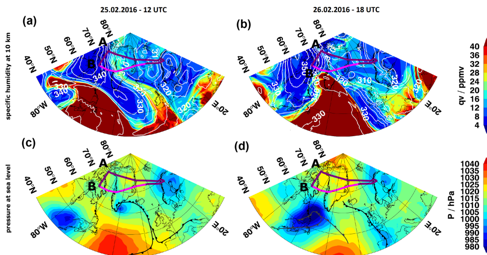
Figure 4. Meteorological conditions in the tropopause region and at sea level on 25 February 2016 ( a , c ) and the flight day, 26 February 2016 ( b , d ), as modelled by ICON-ART. Specific humidity is shown by colour contours, and potential temperature is shown as white contour lines at 10 km altitude ( a , b ). Pressure at sea level is shown with selected warm fronts, cold fronts and occlusions (black and dark-grey overlays) ( c , d ). The HALO flight track on flight day is indicated by a purple line. The section of the flight that covers the filaments observed by GLORIA and analysed in the model data in Sect. 4.2 and 4.3 is highlighted in magenta in all panels.
