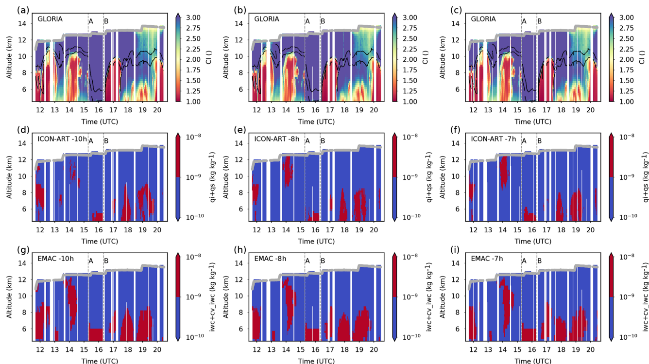
Figure A1. Same as Fig. 5, but model data (ICON-ART and EMAC) have been sampled with a constant time offset of -10 , -8 and -7 h during the interpolation to the GLORIA geolocations along the flight.
