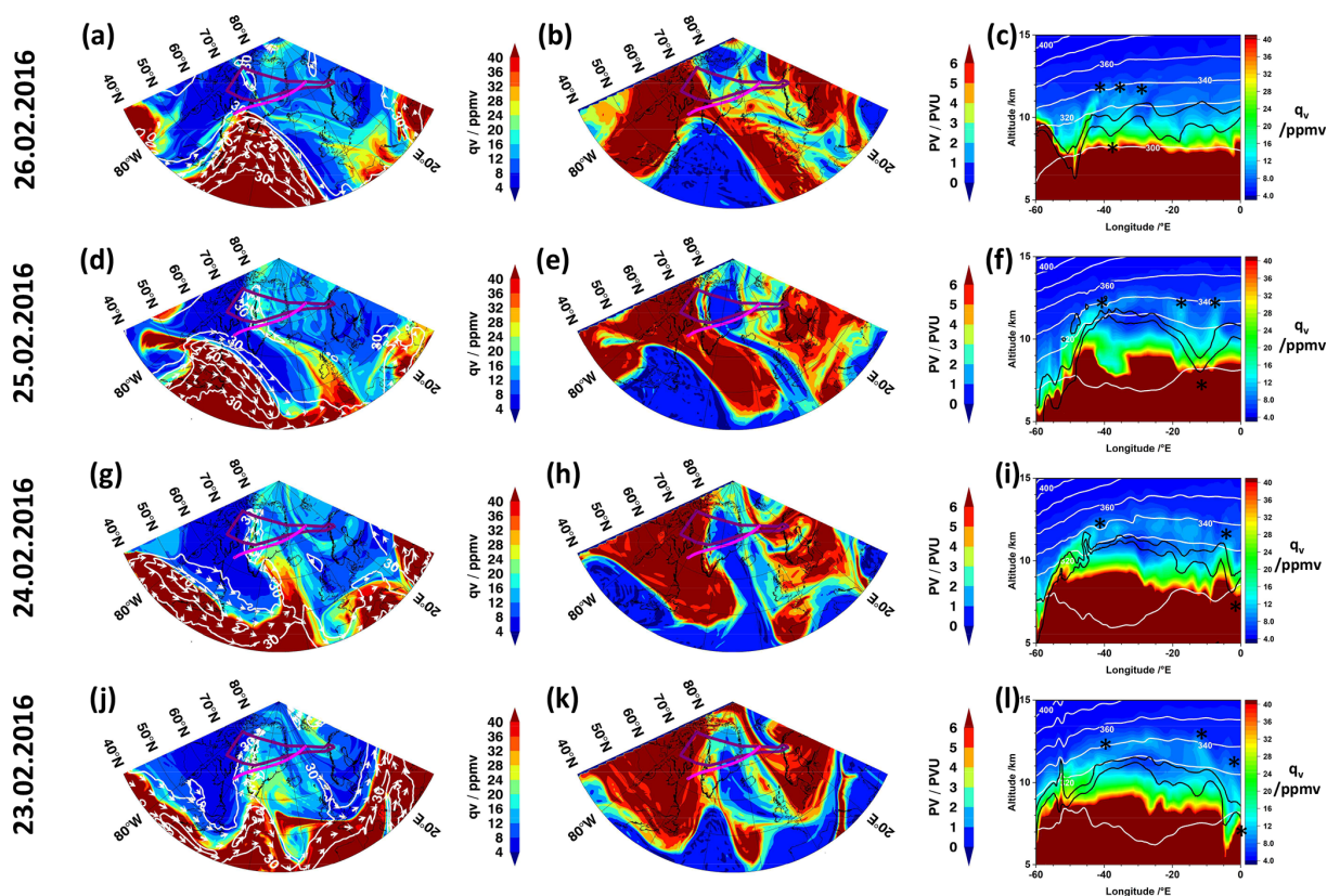
Figure 10. Evolution of filaments in nested ICON-ART domain. (a, d, g, j) Horizontal distribution of q_v (coloured contour) and horizontal wind speed (white contour lines – in intervals of 20 \text{ m s}^{-1} – and arrows) and (b, e, h, k) PV (coloured contour) at 10 km altitude. (c, f, i, l) Vertical distribution of q_v (coloured contour; ppmv), potential temperature (white contour lines; in intervals of 20 K), and 2 and 4 PVU isoline (lower and upper black line) as indicators for the dynamical tropopause. Purple lines in the left and middle column indicate the flight track and magenta lines the location of the vertical cross sections shown in the right column. Stars (c, f, i, l) indicate features in these panels which correspond to features in the other panels out of these. The model data are shown at 12:00 UTC of the dates indicated on the left.
