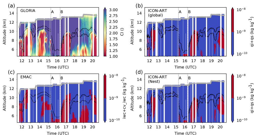
Figure 5. Qualitative comparison of clouds along the flight track observed by GLORIA and cloud masks generated from ICON-ART and EMAC. (a) Vertical cross section of cloud index (CI) derived from GLORIA spectra. (b, d) Cloud mask constructed from global and nested ICON-ART domain of specific cloud ice content plus snow mixing ratio. (c) Cloud mask constructed from EMAC large-scale snow and ice content plus convective cloud snow and ice content. Black lines: 2 and 4 PVU isolines (lower and higher lines, respectively) from ECMWF reanalysis (a) , ICON-ART (b, d) and EMAC (c) as indicators for the dynamical tropopause. Grey lines: HALO flight altitude.
