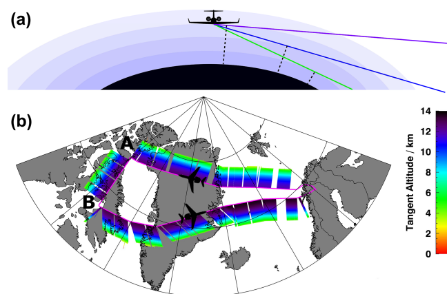
Figure 1. (a) Schematic representation of airborne limb viewing geometry. (b) GLORIA sampling during PGS14 on 26 February 2016. The tangent points of the GLORIA limb views are colour-coded with altitude. Characteristic waypoints are marked “A” and “B”.
