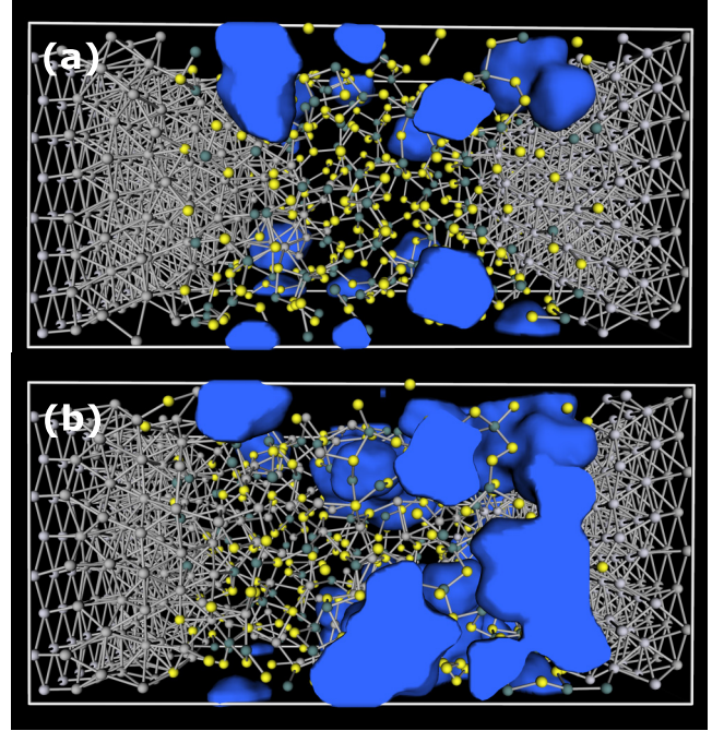
FIG. 6. Cavities at (a) beginning (0 ps) and (b) end (500 ps) of 480 K simulation (cutoff radius 3.2 Å, cavity domains assigned using all atoms [35]). Silver: Ag and Pt atoms.
