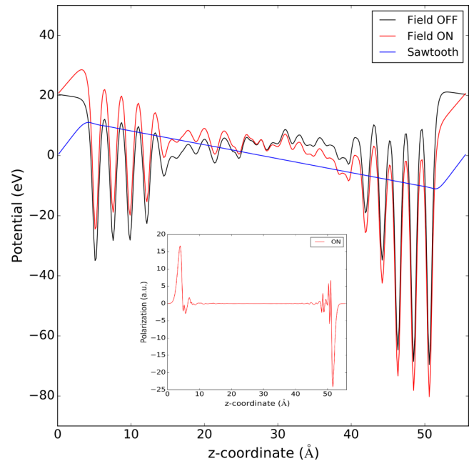
FIG. 8. Laterally averaged electrostatic potential and polarization (inset) as a function of location for a snapshot at the end (500 ps) of the 480 K simulation. The electrostatic potential is calculated with the field ON/OFF ( -0.20 eV/Å). Blue: external sawtooth potential. Polarization dominates in the vacuum-facing layers and the charge transferred is 4.28e (electron accumulation on Ag side).
