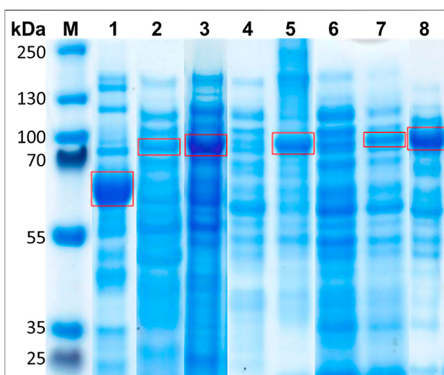
FIGURE 3 | SDS-PAGE analysis of the soluble and insoluble protein content during enzyme production in E. coli after cell disruption. (1) Soluble fraction of ApPDC -EGWH production (61 kDa). (2) Soluble fraction of SOPP- ApPDC -EGWH production (75 kDa). (3) Soluble fraction of SOPP3- ApPDC -EGWH production (74 kDa). (4) Soluble and (5) insoluble fraction of EcFbFP- ApPDC -EGWH production (78 kDa). (6) Soluble and (7) insoluble fraction of Pp2FbFP- ApPDC -EGWH production (79 kDa). (8) Soluble fraction of SuperNova- ApPDC -EGWH production (89 kDa). (M) Marker PageRuler™ Plus Prestained Protein Ladder (Thermo Fisher Scientific, Waltham, MA, United States). Target protein bands are indicated by a red box. 5.5 \mu\text{L} of the appropriately prepared enzyme solution was applied to the gel.
