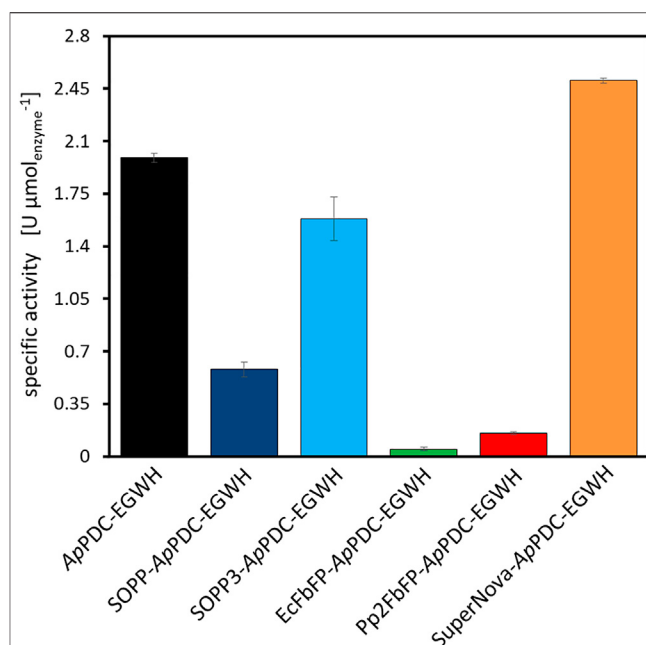
FIGURE 6 | Initial rate of the photosensitizer fusion enzymes in dark conditions compared to the untagged ApPDC -EGWH. For fusions with EcFbFP and Pp2FbFP the activity of the insoluble protein aggregates was determined, apart from this soluble (fusion) enzymes were used. General reaction conditions: 40 mM 3-hydroxybenzaldehyde, 200 mM pyruvate (sodium salt) and 50 mM HEPES buffer (pH 7.5) with 2.5 mM MgSO 4 and 0.1 mM ThDP. Incubation on 1 ml scale at 22°C and 850 rpm in a thermomixer. The displayed enzyme activities in U μmol enzyme -1 correspond to an amount of 1 μmol of each purified and lyophilized fusion enzyme. The error bars describe standard deviation of the technical triplicates.
