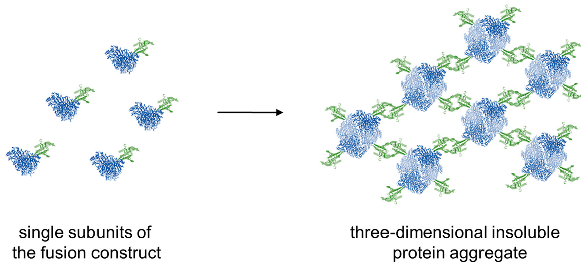
FIGURE 4 | Schematic representation of the formation of insoluble three-dimensional protein aggregates by the combination of a dimeric photosensitizer with a tetrameric enzyme. Green: dimeric photosensitizers (EcFbFP or Pp2FbFP); blue: tetrameric ApPDC-EGWH.
