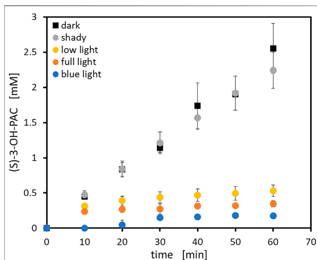
FIGURE 7 | Activity test of SOPP3-ApPDC-EGWH ( 0.5 \text{ mg ml}^{-1} ; purified and lyophilized) at different light conditions (details are given in Table 2 ) and 60 min of exposure time. General reaction conditions: 40 mM 3-hydroxybenzaldehyde, 200 mM pyruvate (sodium salt) and 50 mM HEPES buffer (pH 7.5) with 2.5 mM \text{MgSO}_4 and 0.1 mM ThDP. Incubation on 1 ml scale at 22^\circ\text{C} and 850 rpm in a thermomixer (dark conditions) or in a stirred quartz-glass cuvette (illuminated setups). The error bars describe standard deviation of technical triplicates.
