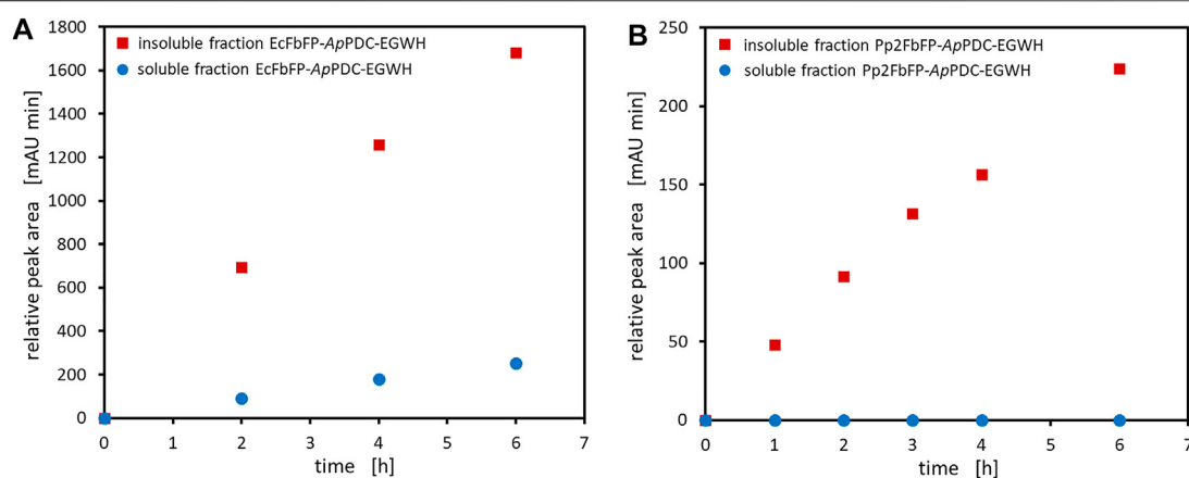
FIGURE 5 | Activity test of the soluble and insoluble protein fraction after cell disruption of samples taken during the production of EcFbFP-ApPDC-EGWH (A) and Pp2FbFP-ApPDC-EGWH (B). General reaction conditions: Incubation on 1 ml scale at 22°C and 850 rpm for 6 h in a thermoshaker using 50 mM HEPES buffer (pH 7.5), 2.5 mM MgSO 4 , 0.1 mM ThDP and 200 mM pyruvate (sodium salt) with (A) 35 mM benzaldehyde and (B) 40 mM 3-hydroxybenzaldehyde. The amount of lyophilized soluble and insoluble protein was equivalent to 500 mg wet cell weight.
