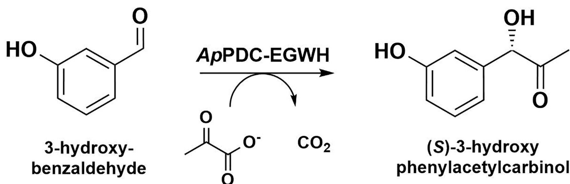
FIGURE 1 | Carboligation of 3-hydroxybenzaldehyde and pyruvate to (S)-3-hydroxyphenylacetylcarbinol ((S)-3-OH-PAC) and CO 2 catalyzed by the pyruvate decarboxylase variant E469G/W543H from Acetobacter pasteurianus (ApPDC-EGWH).
