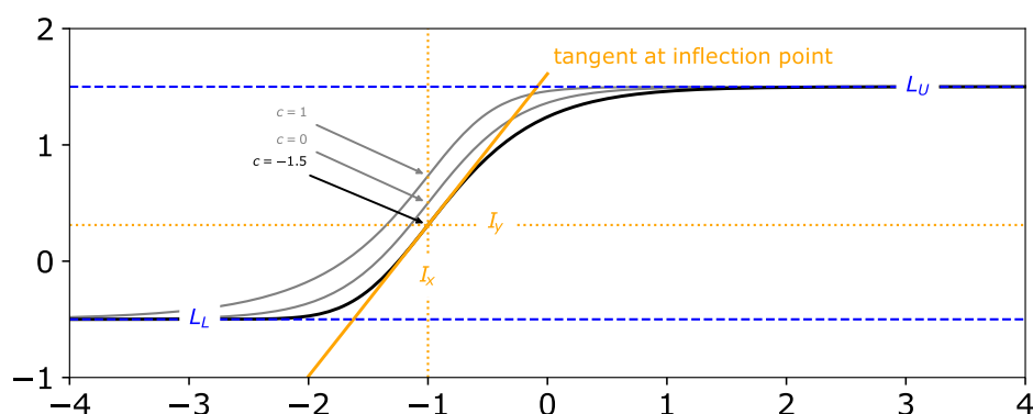
Fig 5. Reparametrized asymmetric logistic function. When parametrized as shown in Eq 11, each of the 5 parameters can be manipulated without influencing the others. Note that, for example, the symmetry parameter c can be changed without affecting the x-coordinate of the inflection point ( I_x ), or the slope S at the inflection point (gray vs. black).
