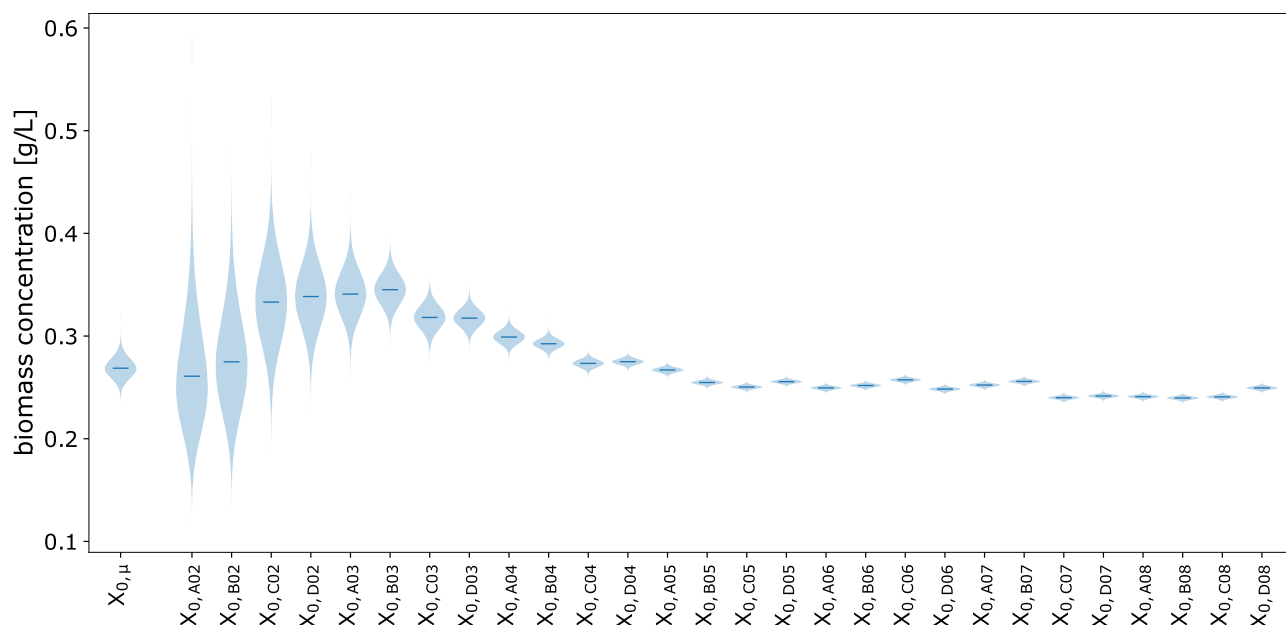
Fig 15. Posterior group mean and well-specific initial biomass concentrations X_0 . Variability between the growth curves in separate wells is described by well-specific initial biomass concentrations X_{0,\text{well}} . Their posterior probability distribution is wide if the well was sacrificed early (left) and narrows down with the number of observed time points (right). Their common hyperprior (a.k.a group mean prior) X_{0,\mu} for the mean of each X_{0,\text{well}} was updated to a posterior with \text{HDI}_{X_{0,\mu}}^{90\%} = [0.250, 0.288] \frac{\text{g}}{\text{L}} .
