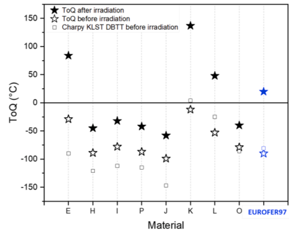
Fig. 9. T_{0Q} measurements by fracture toughness tests with the Master curve approach before and after irradiation at 300°C \pm 30°C, 2.5 dpa. Materials M and N were excluded because of the failing irradiation temperature. Data of EUROFER97 (taken from MPH) are included as reference as well as DBTT measured by Charpy tests on unirradiated KLST samples.
