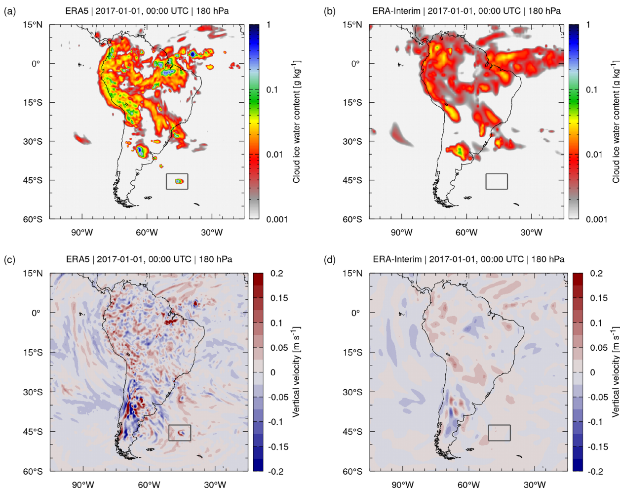
Figure 12. Ice water content ( a , b ) and vertical velocities ( c , d ) of ERA5 ( a , c ) and ERA-Interim ( b , d ) on 1 January 2017, 00:00 UTC, at the 180 hPa pressure level. The gray box near (45° S, 45° W) highlights a convective event in the ERA5 data (see text for details).
