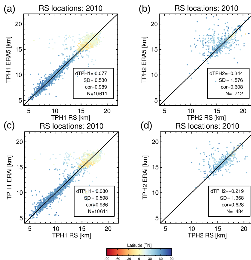
Figure 17. Correlation diagram of HVRRD first (a, c) and second (b, d) tropopause heights versus ERA5 (a, b) and ERA-Interim (c, d) tropopause heights for the 2010 radiosonde (RS) locations, respectively.
