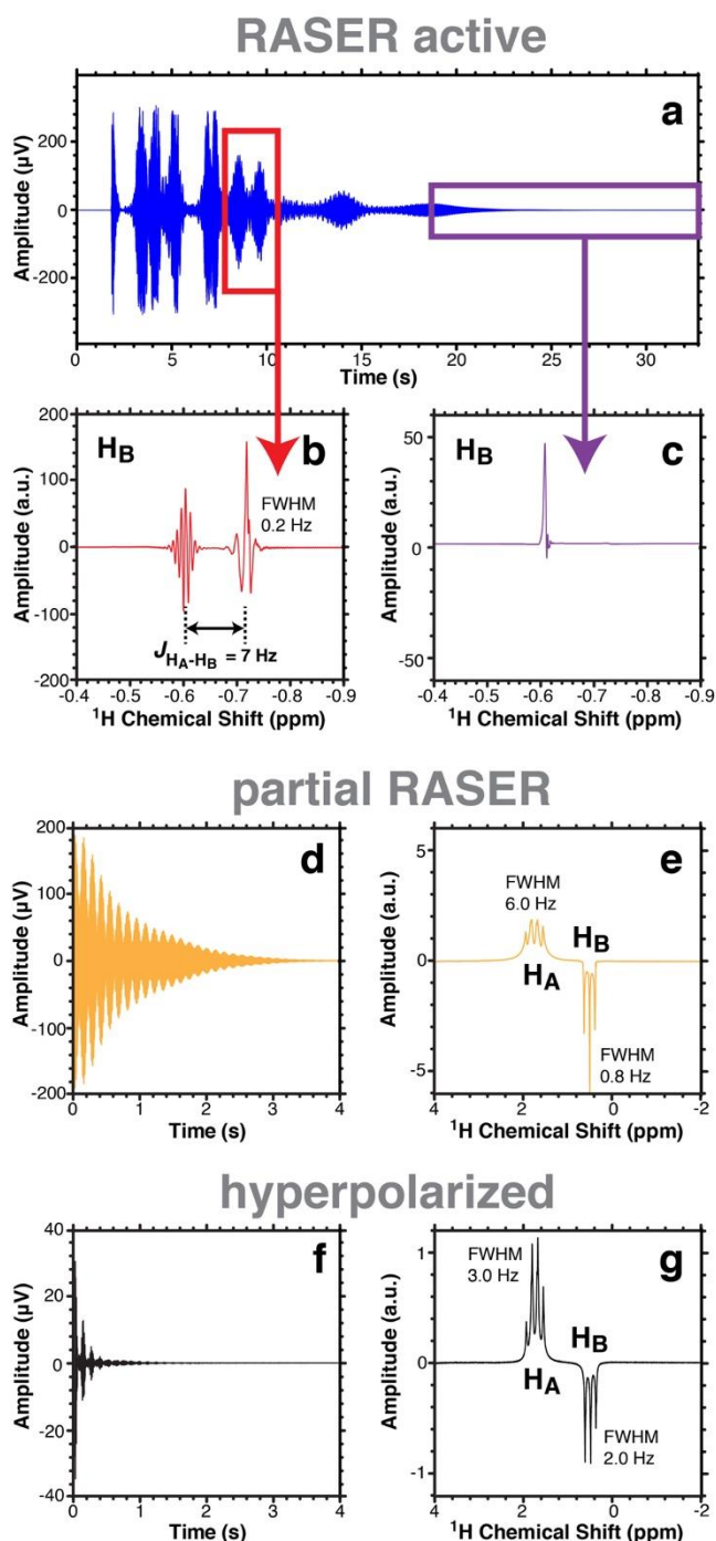
Figure 3. ^1\text{H} NMR spectroscopy of solution-phase PHIP of 0.4 M HP 2-hydroxyethyl propionate (HEP) probed at 1.4 T. a) ALTADENA RASER signal recorded without RF pulse after hydrogenation in the Earth's magnetic field. b,c) Fourier spectra of the regions outlined by red and purple lines in display a), respectively. d,e) Partial ALTADENA RASER signal and Fourier spectrum acquired using \sim 3^\circ RF pulse. f,g) Canonical ALTADENA (non-RASER) FID and Fourier spectrum recorded after further polarization decay ( \sim 30 s). h) PASADENA RASER signal recorded without RF pulse after hydrogenation at 1.4 T. i,j) Fourier spectra of the regions outlined by red and purple lines in display h), respectively. k,l) Partial PASADENA RASER signal and Fourier spectrum acquired using \sim 3^\circ RF pulse. m,n) Canonical PASADENA (non-RASER) FID and Fourier spectrum acquired with \sim 3^\circ RF pulse after further polarization decay ( \sim 30 s).
