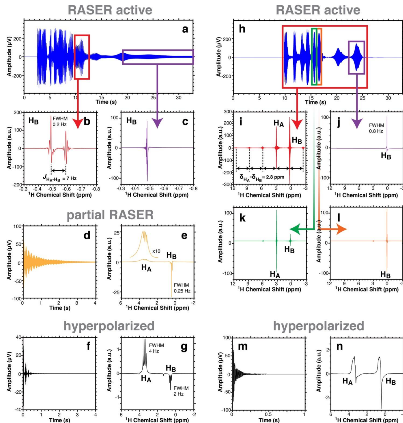
Figure 2. ^1\text{H} NMR spectroscopy of solution-phase PHIP of 0.4 M HP ethyl acetate (EA) probed at 1.4 T. a) ALTADENA RASER signal recorded without RF pulse after hydrogenation in the Earth's magnetic field. b,c) Fourier spectra of the regions outlined by red and purple boxes in display a), respectively. d,e) Partial ALTADENA RASER signal and Fourier spectrum obtained with ~3° RF pulse. f,g) Canonical ALTADENA (non-RASER) FID and Fourier spectrum recorded after further polarization decay. h) PASADENA RASER signal recorded without RF pulse after hydrogenation at 1.4 T. i,j,k,l) Fourier spectra of the regions outlined by red, purple, green and orange boxes in display h), respectively. m,n) Canonical PASADENA (non-RASER) FID and Fourier spectrum acquired with ~3° RF pulse after further polarization decay (~30 s).
