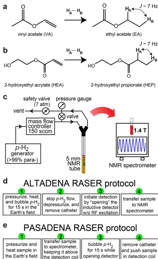
Figure 1. a,b) Reaction schemes for the p\text{-H}_2 pairwise addition to vinyl acetate (VA) yielding to ethyl acetate (EA) and to 2-hydroxyethyl acrylate (HEA) yielding to 2-hydroxyethyl propionate (HEP), respectively. c) Schematic of the experimental setup. d,e) ALTADENA and PASADENA protocols used to evidence parahydrogen-induced RASER activity, respectively.
