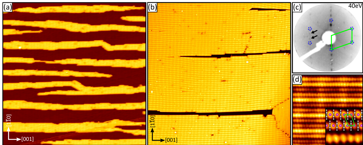
FIG. 6. (a) and (b) STM topographs ( 1500 \times 1500 \text{ \AA}^2 ) of (a) elongated EuCot wire carpet islands and (b) a full layer on Gr/Ir(110) oriented along the [001] direction. (c) 40-eV LEED pattern of the same sample as in (b). The unit cell of the EuCot wire carpet is indicated by the green rhomboid, with the corresponding first-order reflections encircled by dashed blue lines. 3 \times 1 superstructure reflections are highlighted by black arrows. (d) STM topograph ( 100 \times 100 \text{ \AA}^2 ) of EuCot/Gr/Ir(110) with a 3 \times 1 intensity variation along the [1\bar{1}0] direction resulting from the lattice mismatch of the substrate moiré and the wire carpet. Inset: molecular resolution STM topograph ( 25 \times 25 \text{ \AA}^2 ) overlaid with a wire model. Magenta dots, Eu atoms; white and black dots, H atoms and C atoms of Cot. The wire carpet unit cell is indicated as a green rhomboid. STM topographs were taken at 300 K. Tunneling parameters are (a) U_{\text{bias}} = -2.0 \text{ V} and I_t = 0.03 \text{ nA} , (b) U_{\text{bias}} = -1.74 \text{ V} and I_t = 0.08 \text{ nA} , and (d) U_{\text{bias}} = -1.82 \text{ V} and I_t = 0.35 \text{ nA} .
