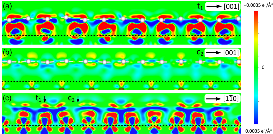
FIG. 3. (a) and (b) Charge density difference plots in the (a) trough and (b) crest locations indicated in Fig. 2(b) as t_1 and c_2 and in Fig. 2(a) by horizontal red lines. (c) Charge density difference average over the entire superstructure unit cell and projected onto a plane along the [1\bar{1}0] direction corresponding to the view of Fig. 2(b). The positions of the cuts along t_1 and c_2 are indicated by arrows. The black dashed lines indicate the position of the top-level Ir atoms. See text. The color scale for all plots ranges from charge accumulation in red ( +0.0035 electrons/ \text{\AA}^3 ) to charge depletion in blue ( -0.0035 electrons/ \text{\AA}^3 ).
