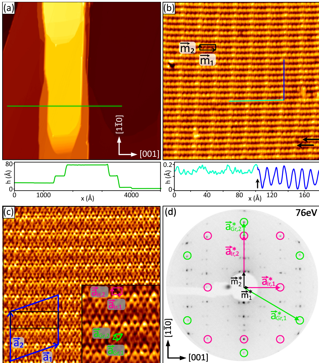
FIG. 1. (a) Large-scale STM topograph ( 7000 \times 7000 \text{ \AA}^2 ) of Gr/Ir(110) grown at T = 1500 \text{ K} . The [001] and [1\bar{1}0] directions specified in the lower right corner are valid also for (b), (c), and (d). The STM height profile along the green line is shown below the topograph. (b) STM topograph ( 300 \times 300 \text{ \AA}^2 ) of flat terrace area. The black rectangle indicates the moiré unit cell. Black arrows highlight the varying appearance of wave crests. The STM height profile along the path of the cyan and blue lines is shown below the topograph. A small black arrow in this height profile plot marks the location where the profile changes from the [001] to [1\bar{1}0] direction. (c) Atomic resolution STM topograph ( 100 \times 100 \text{ \AA}^2 ) with commensurate superstructure cell and primitive translations \vec{a}_1 and \vec{a}_2 indicated by the blue rhomboid. The moiré unit cell is shown with a black rectangle. Inset: magnified view ( 30 \times 30 \text{ \AA}^2 ) with centers of Gr rings visible as dark depressions. Gr and Ir(110) unit cells and primitive translations are indicated. (d) 76-eV LEED pattern of Gr/Ir(110). First-order Ir and Gr reflections are encircled in magenta and green, respectively. Reciprocal moiré, Gr, and Ir primitive translations are indicated. See text. STM imaging temperatures are 300 K in (a) and (b) and 1.7 K in (c). Tunneling parameters are (a) U_{\text{bias}} = -1.33 \text{ V} and I_t = 0.8 \text{ nA} , (b) U_{\text{bias}} = -1.33 \text{ V} and I_t = 1.1 \text{ nA} , and (c) U_{\text{bias}} = -0.05 \text{ V} and I_t = 20.0 \text{ nA} .
