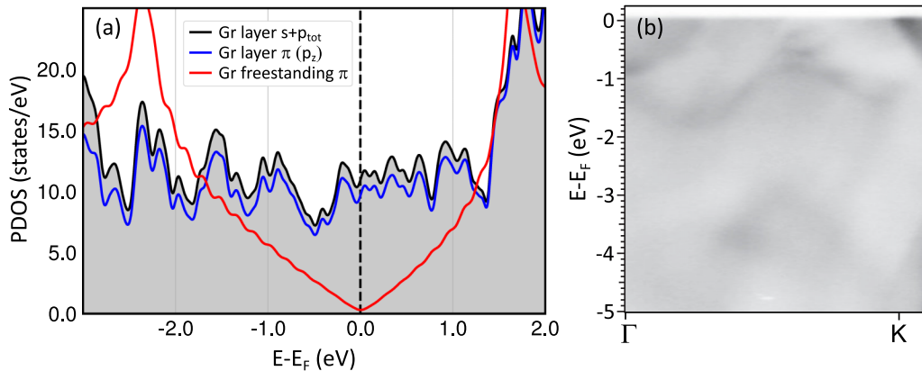
FIG. 4. (a) Red line, density of states (DOS) of freestanding Gr; black line and gray-shaded area, Gr partial DOS (PDOS) when on Ir(110); blue line, Gr partial DOS projected on the Gr \pi system consisting of p_z atomiclike orbitals. See text. (b) Angle-resolved photoemission spectrum along \Gamma - K , recorded at a photon energy of 100 eV and a temperature of T = 35 K. There is no Dirac cone at the K point, and there are no features that could be related to the Gr \pi bands in agreement with the DFT calculations.
