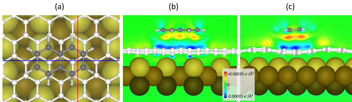
FIG. 5. (a) Top-view ball model for the minimum energy adsorption geometry of C_{10}H_8 in trough t_1 on Gr/Ir(110) (compare Fig. 2). (b) Charge density difference plot along the blue line in (a) of the combined system compared with the sum of the isolated C_{10}H_8 molecule and Gr/Ir(110). (c) Same as (b), but along the red line in (a). The color scale in (b) and (c) is the same as in Fig. 3, but used for one order of magnitude smaller charge density differences ranging from +0.00035 electrons/ \text{\AA}^3 for charge accumulation in red to -0.00035 electrons/ \text{\AA}^3 for charge depletion in blue.
