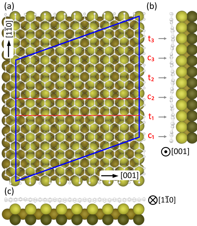
FIG. 2. Ball model representations of relaxed DFT geometries for Gr/Ir(110). Ir atoms, light (top layer) to dark (bottom layer) brown spheres; C atoms, small light gray spheres connected by light gray lines. (a) Top view with DFT supercell indicated by the blue rhomboid. The [1\bar{1}0] and [001] directions are also shown. (b) Side view with the [001] direction out of the drawing plane as indicated. A pattern of crests c_1 – c_3 and troughs t_1 – t_3 in the Gr layer is visible along [1\bar{1}0] with their positions highlighted by arrows. (c) Side view with the [1\bar{1}0] direction into the drawing plane as indicated.
