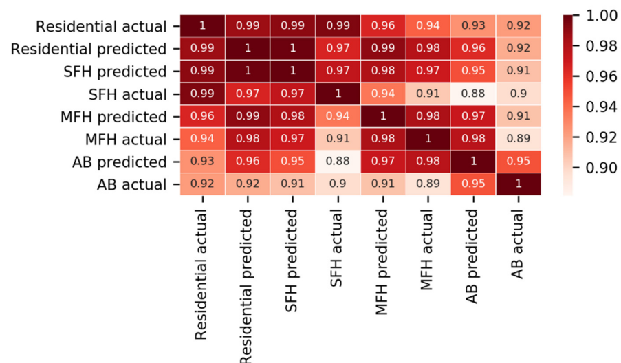
Figure 16. Correlation between different predicted and actual indicators.
