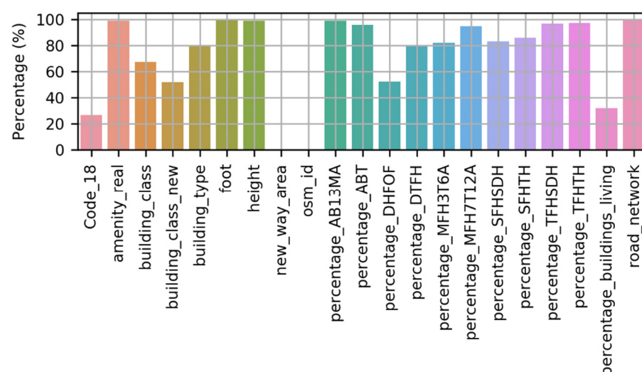
Figure 11. Percentage missingness of data for each feature in the dataset.
