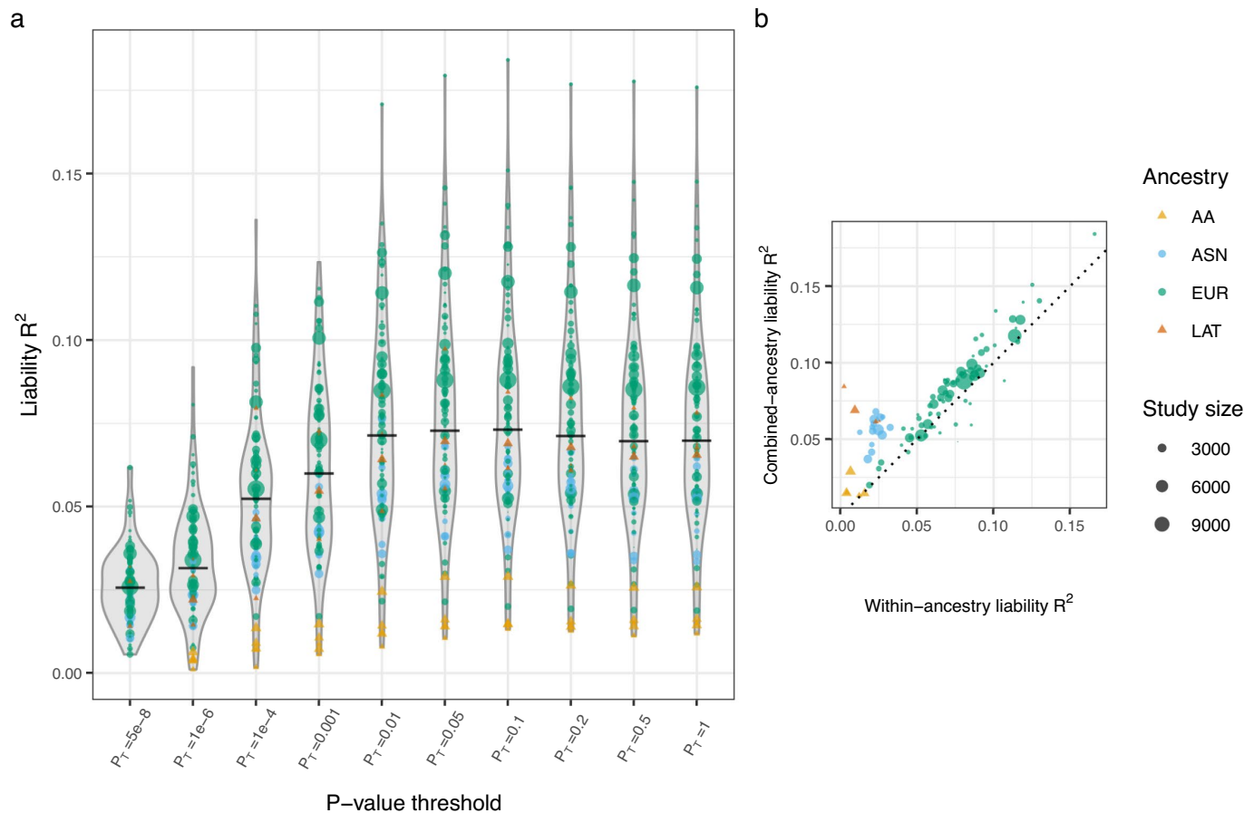
Extended Data Fig. 2 | Polygenic risk prediction. a, Distributions of liability scale R^2 across 98 left-out-cohorts for polygenic risk scores built from SNPs with different p-value thresholds. Distributions of liability R^2 (assuming schizophrenia life-time risk of 1%) are shown for each p-value threshold, with point size representing size of the left-out cohort and colour representing ancestry. The median liability R^2 is represented as a horizontal black line. b, Liability R^2 of predicted and observed phenotypes in left-out cohorts using
