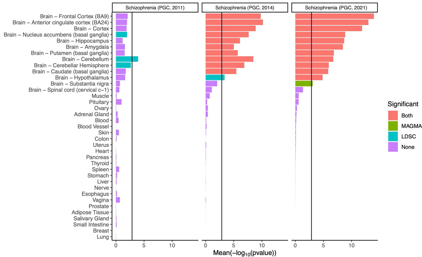
Extended Data Fig. 3 | Association between 37 human tissues and schizophrenia. The mean of the evidence ( -\log_{10}(P) ) obtained from two methods (MAGMA, LDSC) for testing GWAS data for enrichment of association in genes with high expression in each tissue as determined from bulk RNA-seq 14 . The bar colour indicates whether gene expression in the tissue is significantly
