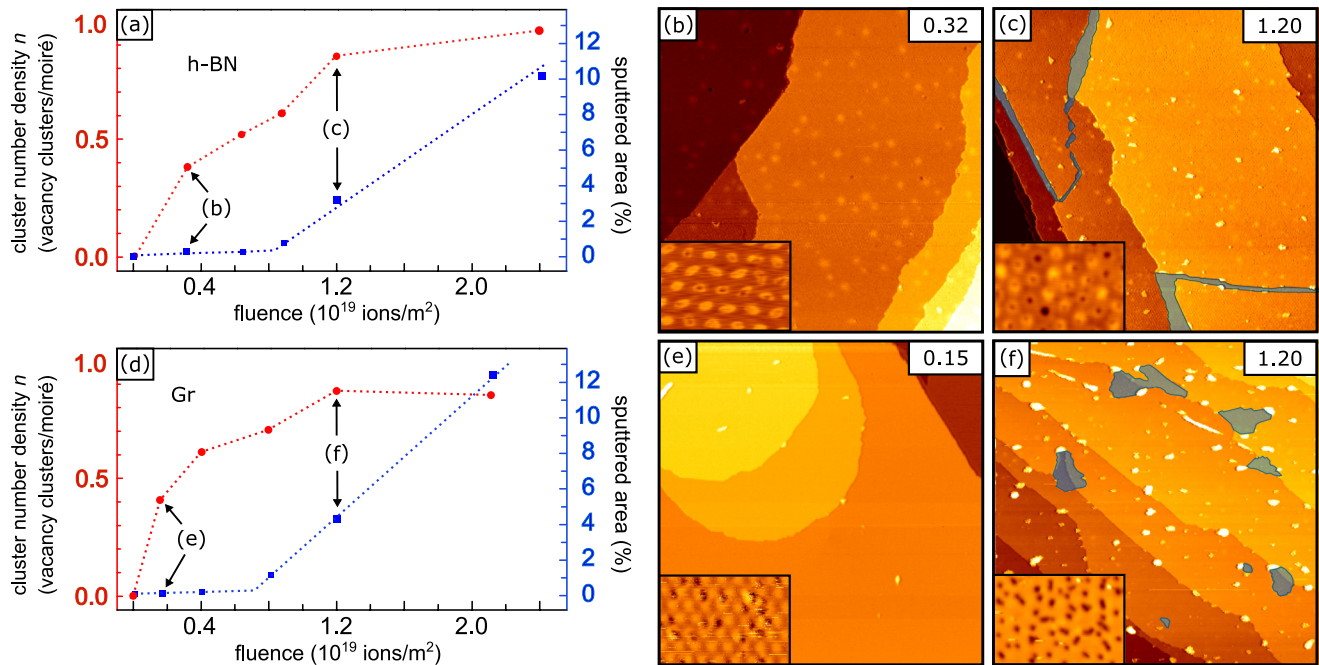
FIG. 4. (a) Dependence of vacancy cluster number density n and sputter removed area in h-BN on Ir(111) on 500 eV He + ion fluence at 1200 K. Full red dots and left axis: n in clusters per moiré cell; full blue squares and right y axis: removed h-BN layer area by sputtering (excluding cluster area). Lines to guide the eye. (b), (c) STM topographs taken after ion fluences as indicated in (a) and in the top right corners in units of 10^{19} ions/m 2 . (d) Same as (a), but for Gr on Ir(111) and at 1150 K irradiation temperature. (e), (f) STM topographs taken after ion fluences as indicated in (d). Insets in STM topographs are magnified views. Removed areas in (c) and (f) are shaded blue. See Figs. S1 and S2 of Ref. [35] for STM topographs of additional fluences and without coloring of sputtered areas. Topograph sizes are 350 nm \times 350 nm, 12 nm \times 17 nm for insets of (b), (c), and 15 nm \times 21 nm for insets of (e), (f). Sample bias is in (b) U_s = -1.4 V and for inset U_s = +1.4 V, in (c) U_s = -1.3 V and for inset U_s = +1.5 V, in (e) U_s = -1.4 V and for inset U_s = -0.8 V, and in (f) U_s = -1.6 V and for inset U_s = -1.8 V.
