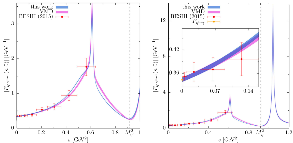
Fig. 2 Determination of the \eta' TFF by means of Eq. (2.3) in comparison to data from BESIII [108] (statistical and systematic errors added in quadrature) scaled with F_{\eta'\gamma\gamma} from Table 1 and the VMD model of Eq. (D.23) with \phi resonance contribution according to Eq. (D.22); for
