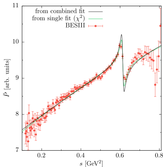
Fig. 1 Fit to the differential decay rate of \eta' \rightarrow \pi^+\pi^-\gamma (individually or combined with the VFF). To highlight differences in the \rho - \omega region, we show the associated function \bar{P} , as defined in Eq. (3.11), compared to the experimental data from BESIII [81]. The function \bar{P} is calculated in units that still contain the event rate
