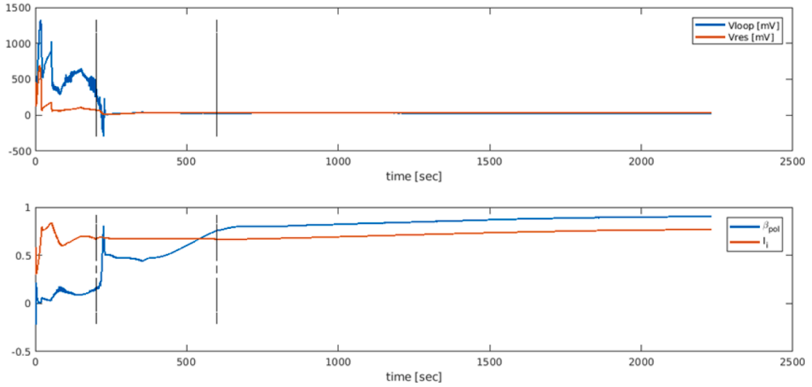
Fig. 2. Loop voltage (top), \beta_{pol} and I_i (bottom) for the ramp-up case shown in Fig. 1. In the top panel, the total loop voltage and its resistive fraction are shown. Black vertical lines identify the end of the current ramp (200 s) and the end of the density ramp (600 s).
