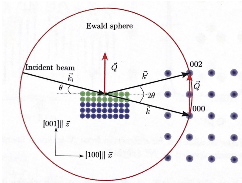
Figure 2.12: Ewald construction for diffraction from a thin film sample. Image taken from [34].
