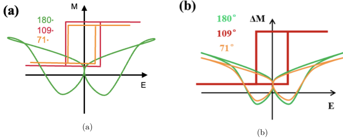
Figure 4.18: Picture of the simulated ME curves for LSMO/PMN-PT(111) and LSMO/PMN-PT(001) related to different domain switching inspired from [25]
