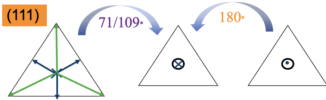
Figure 4.16: Projections of polarizations to the (111) plane before and after 71/109° switching and 180° and corresponding changes of distortion
