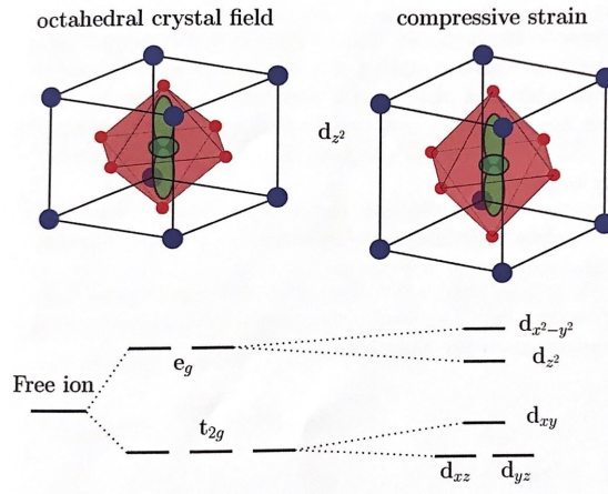
Figure 2.3: Crystal field splitting in octahedral environment and further splitting by compressive strain. The diagram is taken from [34].
