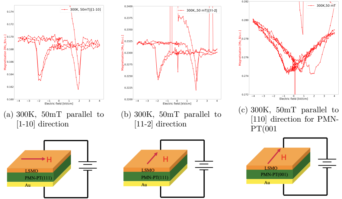
Figure 4.10: Magnetization as a function of electric field at 300K and the schematic of the measurement under different magnetic field direction.
