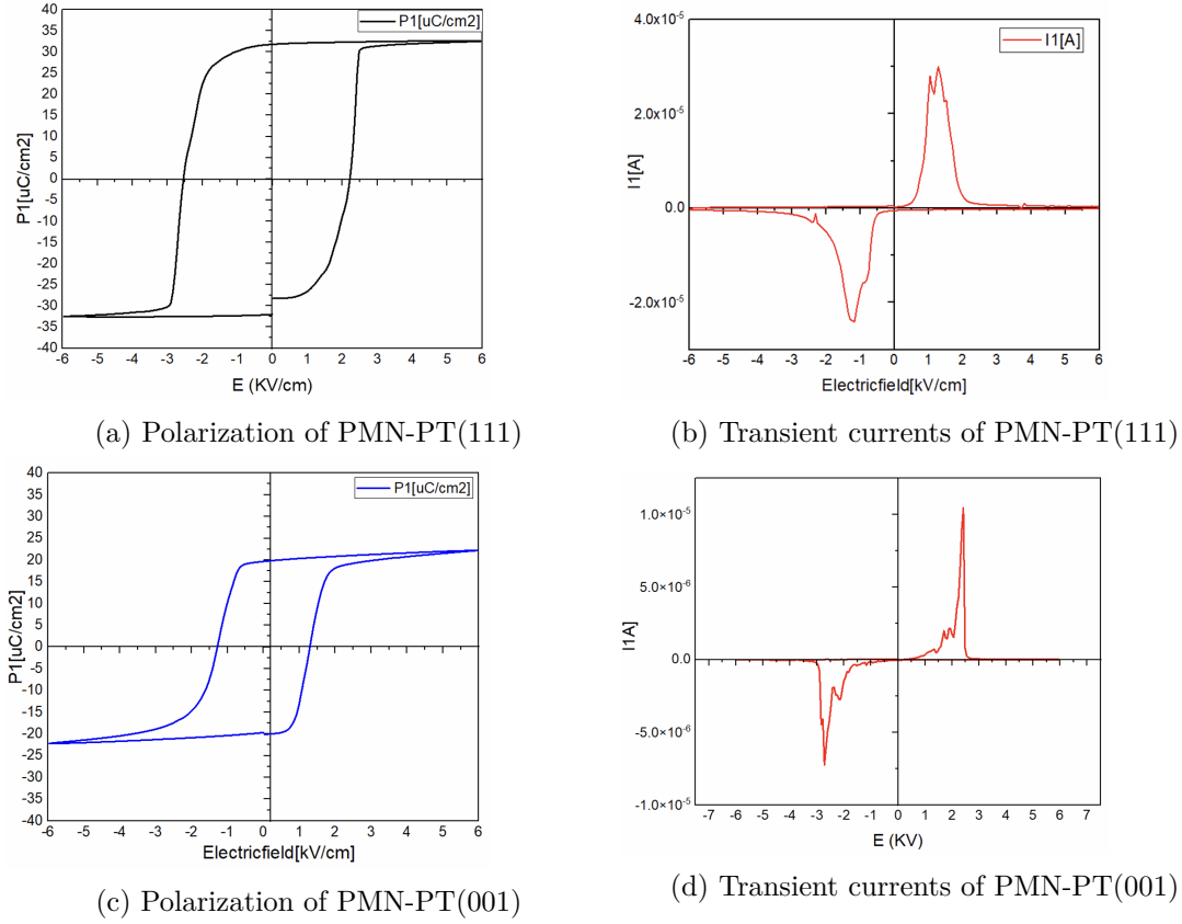
Figure 4.4: (a) Polarization of PMN-PT(111) at 300K with the maximal electric field 6kV/cm. (b) is the transient currents integrated during a triangular field sweep. (c) Polarization of PMN-PT(001) at 300K with the maximal electric field 6kV/cm. (d) is the transient currents integrated during a triangular field sweep.
