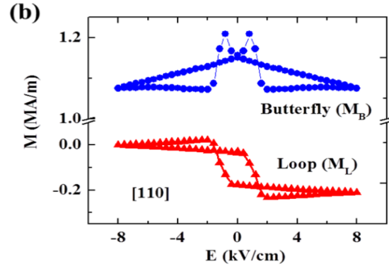
Figure 4.15: The loop-like( M_L , red line) and butterfly-like( M_B , blue line) electric-field control magnetization ME curves reprinted from [25]
