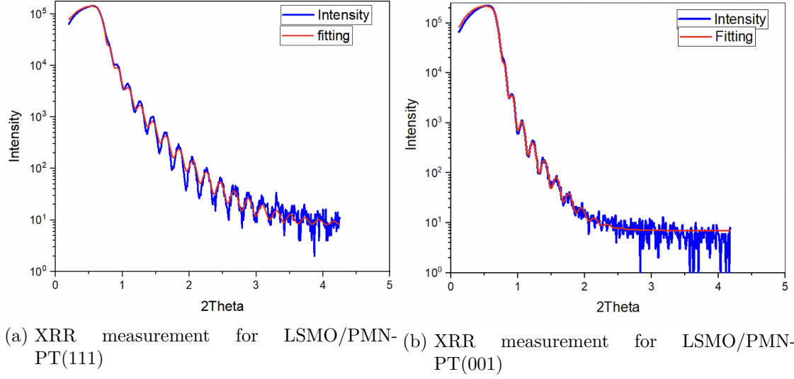
Figure 4.3: XRR measurement and scattering length density profile of sample LSMO/PMN-PT(111) and (001).
