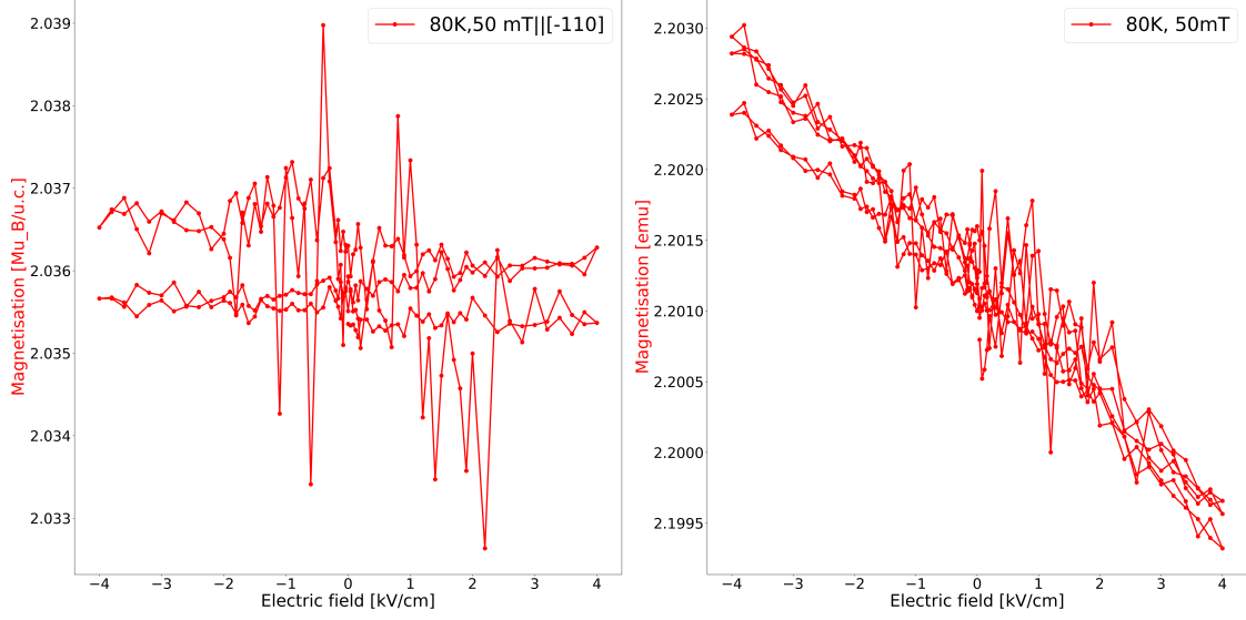
(a) ME curve of LSMO/PMN-PT(111) at 80K under 50mT magnetic field (b) ME curve of LSMO/PMN-PT(001) at 80K under 50mT magnetic field
