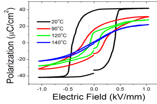
Figure 4.12: Ferroelectric polarization hysteresis at different temperature of PMN-PT taken from [24].
