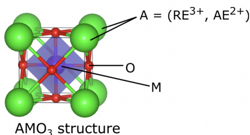
Figure 2.1: Ideal perovskite structure with formula ABO_3 taken from [6]
