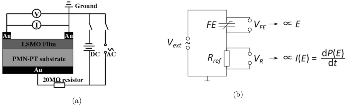
Figure 3.6: (a) is the connect for dynamic hysteresis set-up.(b) is the shunt method to explain the principle.Taken from [31].
