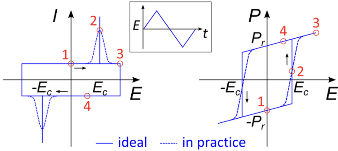
Figure 3.7: Ferroelectric polarization hysteresis (P-E, right) as a result of the transient currents (I-E, left) integrated during a triangular field sweep (inset): (1) linear region around the negative remanent polarization -P_r , (2) switching around the coercive field E_c , (3) saturation region, and (4) linear branch towards the positive remanent polarization P_r . The diagrams are taken from [31].
