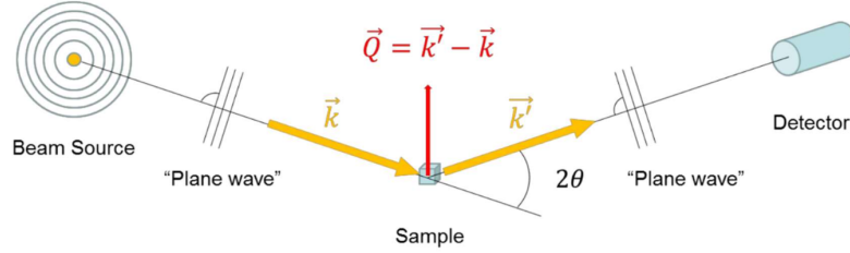
Figure 2.10: Scattering in the Fraunhofer diffraction approximation. Figure taken from ref [10]
