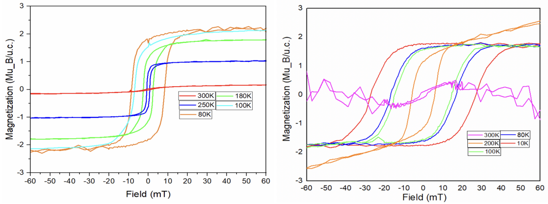
(a) Hysteresis curve of sample LSMO/PMN-PT(111) (b) Hysteresis curve of sample LSMO/PMN-PT(001)
