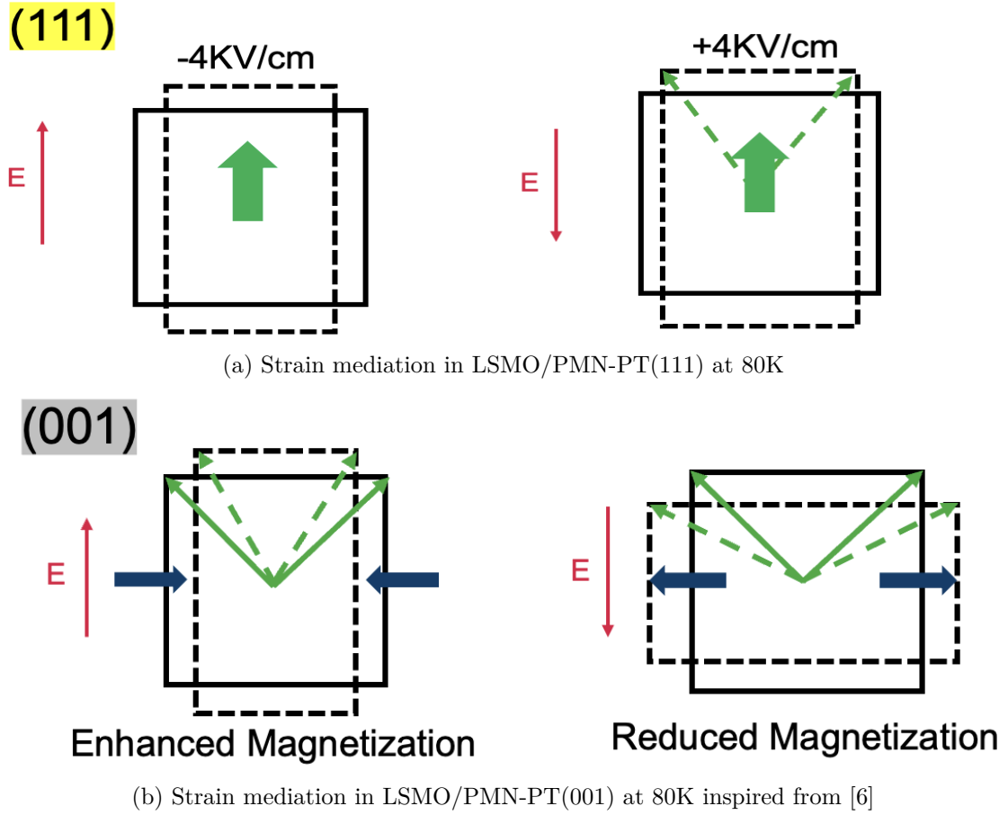
Figure 4.13: Schematic representing the strain-mediation taking place at 80K under positive and negative electric field for LSMO/PMN-PT(111) and (001). The dashed arrows depict the shift of ferroelectric polarizations in PMN-PT.
