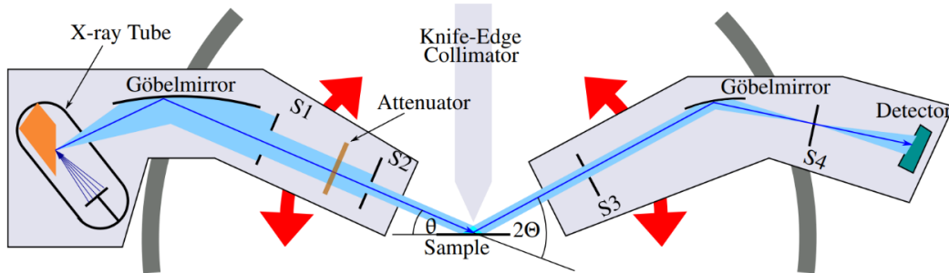
Figure 3.2: Sketch of the Bruker D8 Advance. Taken from [19].
