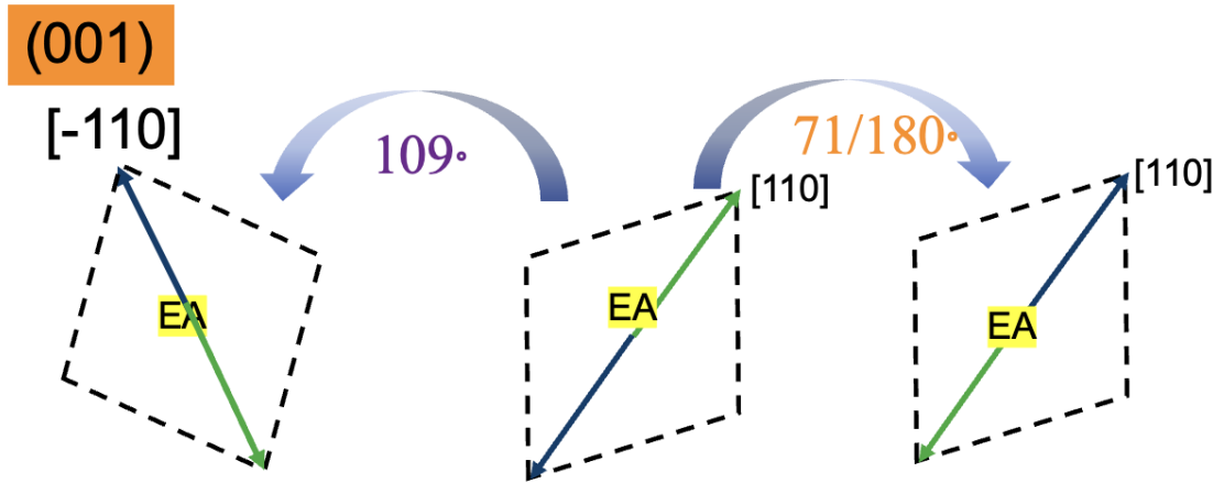
Figure 4.17: Projections of polarizations to the (001) plane before and after 109° switching are perpendicular
