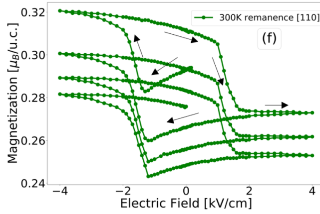
Figure 4.19: ME curve measured with remanent magnetic field along [110]. Taken from [6]
