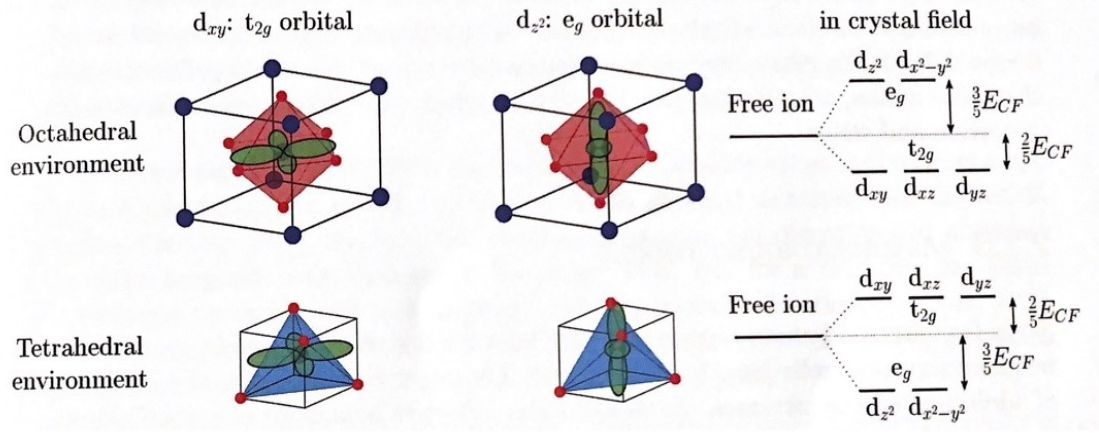
Figure 2.2: Crystal field splitting in octahedral and tetrahedral environment. 3d metal ions are black spheres, the red shaded are oxygen octahedra and cyan shaded the oxygen tetrahedra. The d_{xy} and d_{z^2} orbitals are indicated in green. The diagram is taken from [34].
