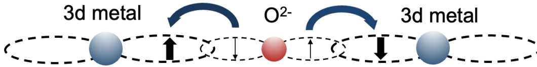
Figure 2.4: Schematic of super-exchange between two 3d metal ions of same valency. The spins of the 3d metal are aligned antiparallel due to a lowering in energy by delocalization.
