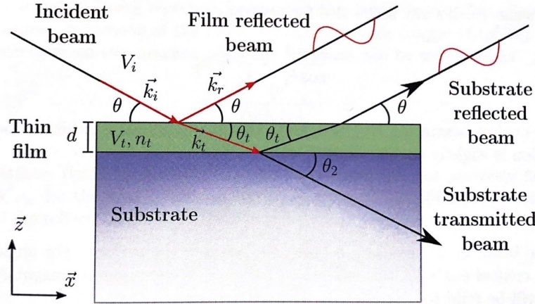
Figure 2.11: Scattering from a thin film sample for a reflection condition. The beam reflected from the film and substrate acquire a phase difference, which results in Kiessig fringes due to constructive and destructive interference for varying incidence angle. Image adapted from [22].
