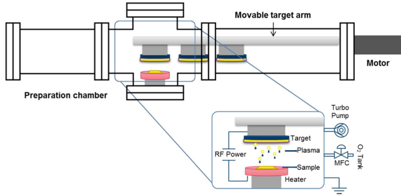
Figure 3.1: Sketch of the HOPSD device. Image taken from [15]. On-axis RF sputtering with a maximum power of 200 W. The target-substrate distance is fixed at 2 cm.
