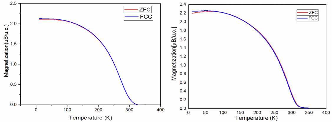
(a) ZFC/FCC curve of sample LSMO/PMN-PT(111) (b) ZFC/FCC curve of sample LSMO/PMN-PT(001)
