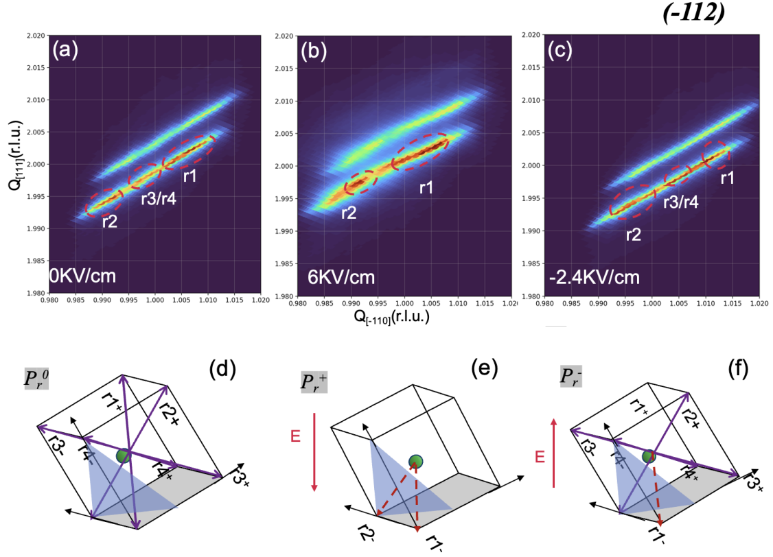
Figure 4.6: Reciprocal lattice map and Schematics of domain structures under different electric field about (-112) reflections of PMN-PT(111). (a),(d) is for unpoled state. (b),(e) is under positive electric field. (c),(f) is applying the coercive field of -2.4 kV/cm. Electric field induced ferroelectric polarization switching is clearly demonstrated in the RSM
