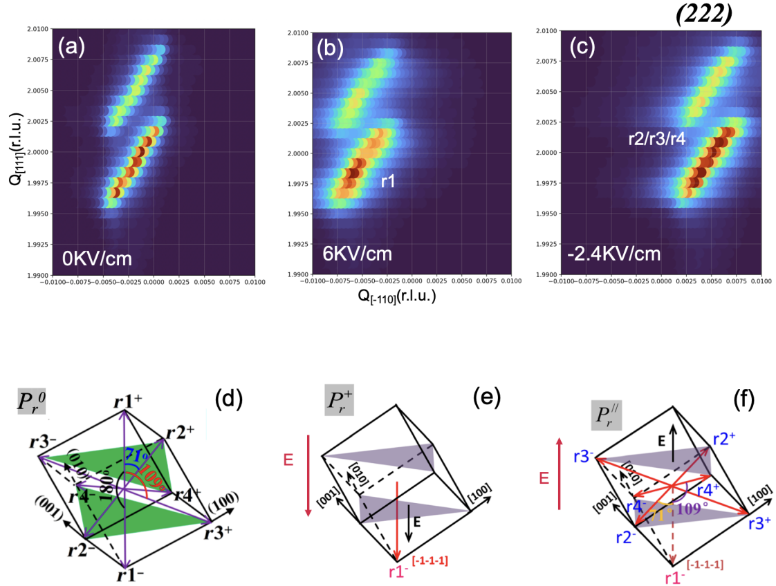
Figure 4.5: Reciprocal lattice map and Schematics of domain structures under different electric field about (222) reflections of PMN-PT(111). (a),(d) is for unpoled state. (b),(e) is under positive electric field with the downwards arrow in (e). (c),(f) is applying the coercive field of -2.4 kV/cm. Electric field induced ferroelectric polarization switching is clearly demonstrated in the RSM
