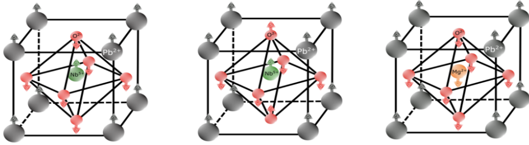
Figure 2.7: Cation-oxygen displacement modes (inspired from [14]).
