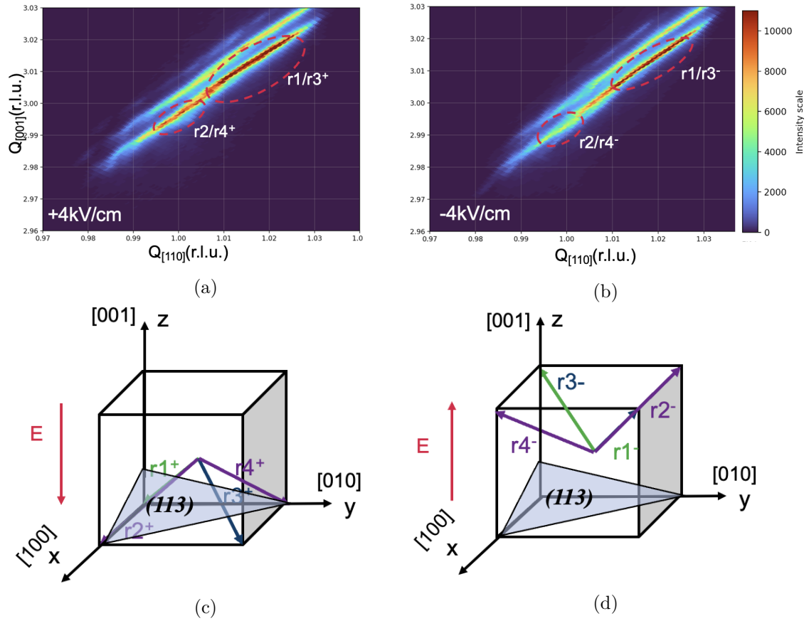
Figure A.1: (a) and (b) are Zoomed reciprocal lattice map in normal scale under positive and negative electric field. Ellipses with different colors in RSMs outline the contours of the deduced spots. (c) and (d) are Configurations of the (113) crystal face and polarisation variants of rhombohedral phase under positive and negative electric fields.
