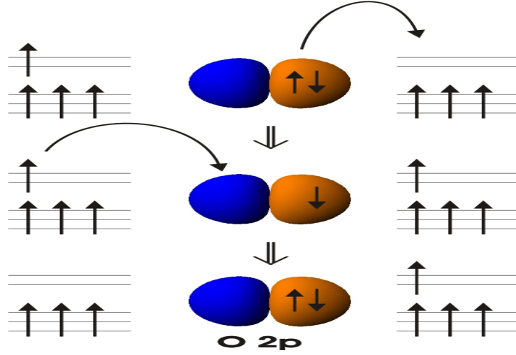
Figure 2.5: Double exchange interaction taking place in Mn-O-Mn bond.
