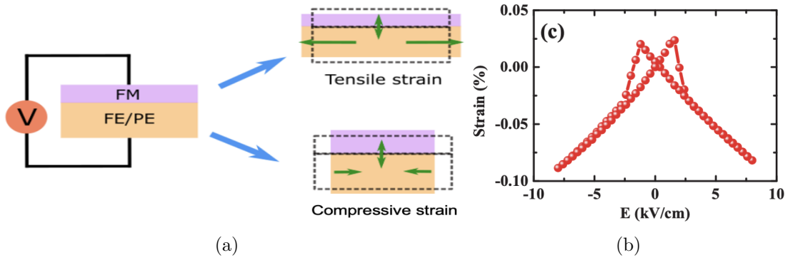
Figure 2.6: (a) Schematic of strain coupling in a FE and FM heterostructure (b) butterfly-shaped curve characteristic of in-plane piezoelectric strain vs electric field taken from [43]
