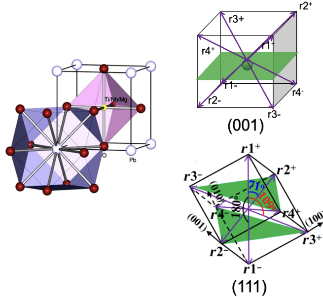
Figure 2.8: PMN-PT structure in (001) and (111) plane(inspired from [14]).
