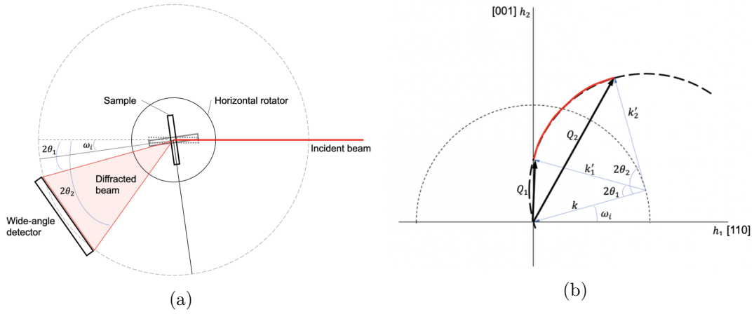
Figure 3.4: (a) is the schematic geometry of the WAXS. (b) is the calculation of the reciprocal data from the WAXS data.
