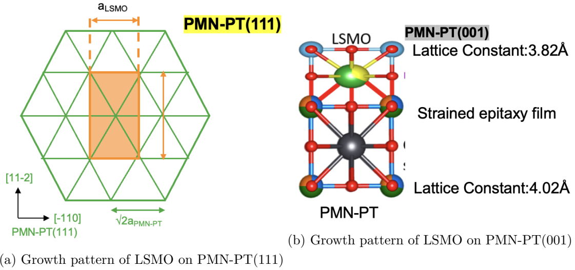
Figure 4.1: Schematic growth method for LSMO thin film on PMN-PT(111) plane and (001) plane inspired from [6].
