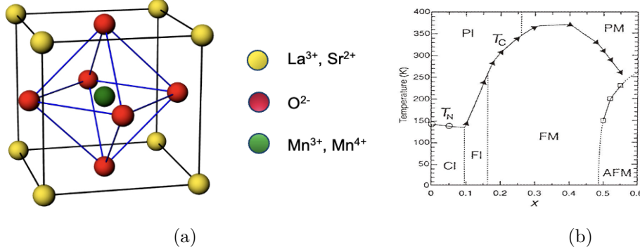
Figure 2.9: (a) La_xSr_{1-x}MnO_3 structure (b) La_xSr_{1-x}MnO_3 phase diagram reproduces from [20].
