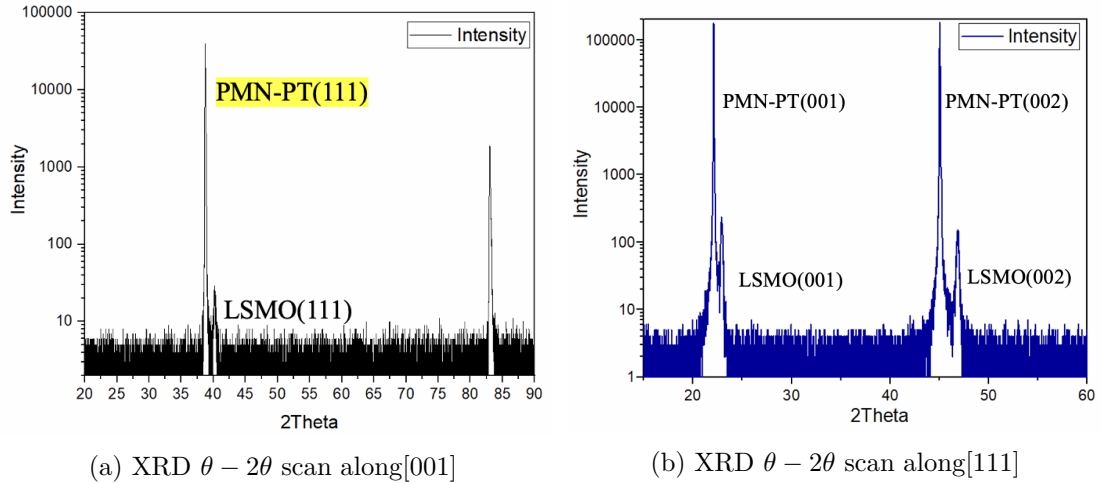
Figure 4.2: XRD measurement of sample LSMO/PMN-PT(111) and (001).
