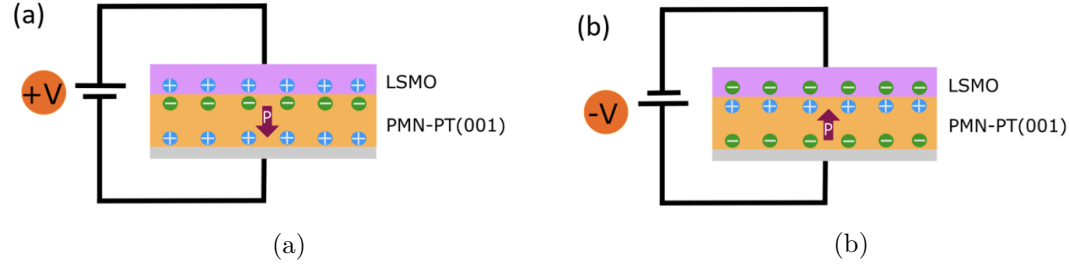
Figure 4.11: (a)Schematics of the interface charge distribution with applied positive voltage.(b)applied negative voltage in the LSMO/PMN-PT(001) heterostructure. Draw adapted from [6].
