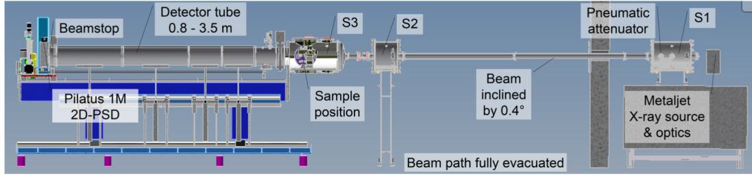
Figure 3.3: Schematic drawing of GALAXI with its main components. The beam direction is from right to left. Image taken from [23].
