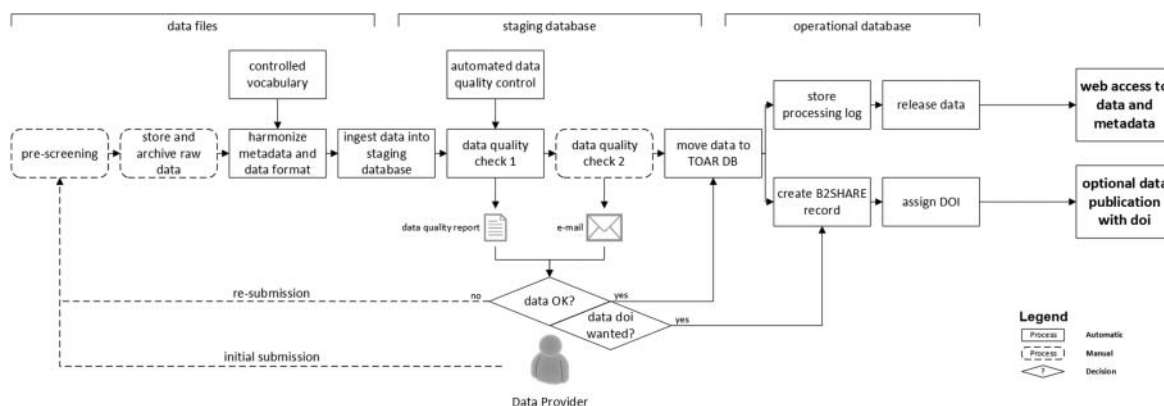
Figure 1. TOAR-II data ingestion workflow.
