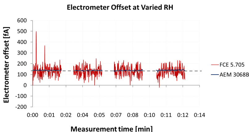
Fig. 28: Electrometer offset current for the FCE 5.705 and AEM 3068B electrometers over 3-minute intervals at varied RH. The dotted line represents the average noise value.
