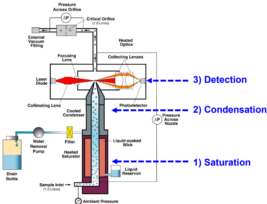
Fig. 4: Operating principle of a typical laminar flow, butanol CPC (Schematic courtesy of TSI Incorporated, Model 3790 EECPC Operation and Service Manual).
