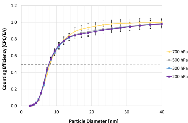
Fig. 43: Measured counting efficiency curves of the Sky-CPC 5.411 for ammonium sulfate at reduced pressures from 700 to 200 hPa.
