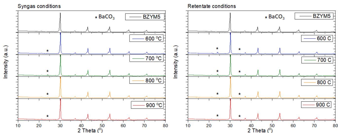
Fig. 14. XRD patterns of BZYM5 powder specimens, before (black pattern) and after exposure to simulated Syngas and Retentate WGSMR conditions at temperatures from 600 °C to 900 °C.
