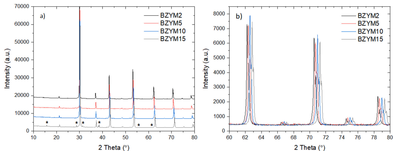
Fig. 3. XRD patterns of a) polished specimens of the series \text{BaZr}_{0.8}\text{Y}_{0.2-x}\text{Mn}_x\text{O}_{3-\delta} where x = 0.02; 0.05; 0.1 and 0.15 (BZYM2, BZYM5, BZYM10 and BZYM15, respectively) sintered at 1700^\circ\text{C} for 10 h; b) Magnified XRD spectra excerpt in the 2\theta range of 60\text{--}80^\circ : peaks shift to the higher 2\theta values with increasing the Mn content. Secondary phases are marked with an asterisk.
