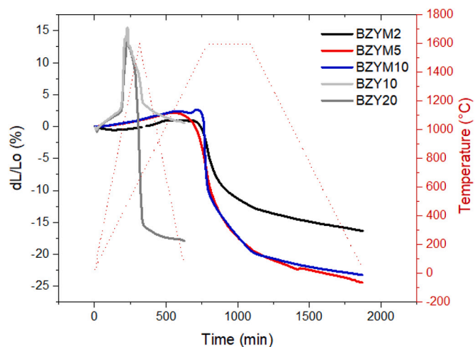
Fig. 5. Shrinkage rate dL/L_0 plotted as a function of the time and the temperature for \text{BaZr}_{0.8}\text{Y}_{0.2-x}\text{Mn}_x\text{O}_{3-\delta} with x = 0.02; 0.05 and 0.1 (BZYM x ). Reference compounds: \text{BaZr}_{0.9}\text{Y}_{0.1}\text{O}_{3-\delta} (BZY10) and \text{BaZr}_{0.8}\text{Y}_{0.2}\text{O}_{3-\delta} (BZY20).
