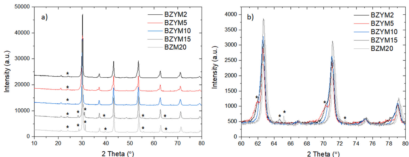
Fig. 2. XRD patterns of a) powder specimens of the series \text{BaZr}_{0.8}\text{Y}_{0.2-x}\text{Mn}_x\text{O}_{3-\delta} where x = 0.02; 0.05; 0.1; 0.15 and 0.20 (BZYM2, BZYM5, BZYM10, BZYM15, BZM20 respectively) after conventional solid state synthesis at 1400^\circ\text{C} for 6 h; b) Magnified XRD spectra excerpt in the 2\theta range of 60\text{--}80^\circ . Secondary phases are marked with an asterisk.
