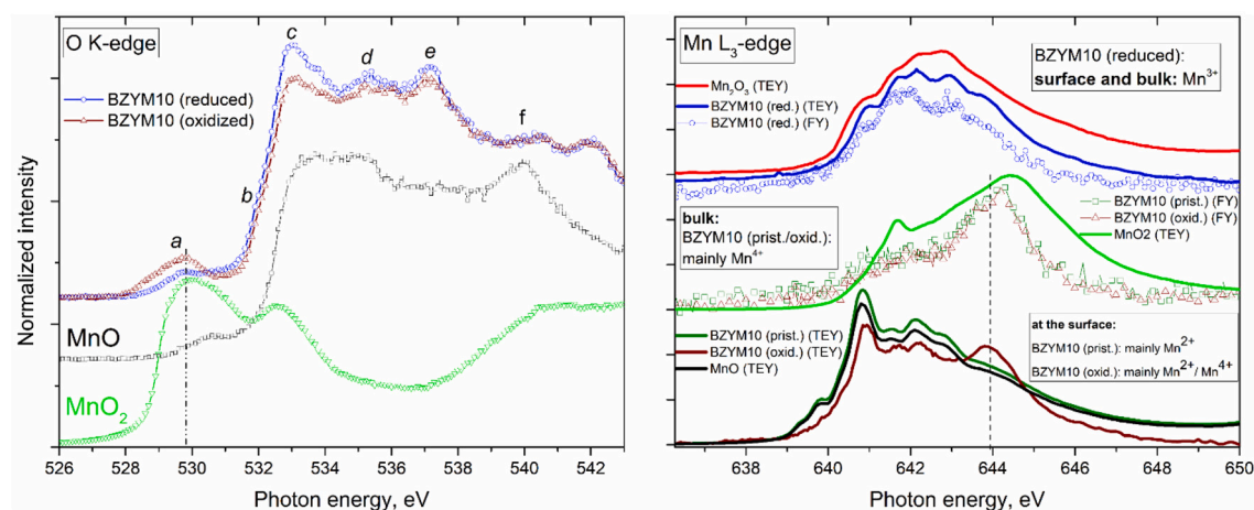
Fig. 13. Comparison of the NEXAFS spectra at O K-edge (left) and Mn L_{3\text{-edge}} (right) of the studied compounds and some reference powders recorded in the TEY (solid line) and FY (symbols) modes.
