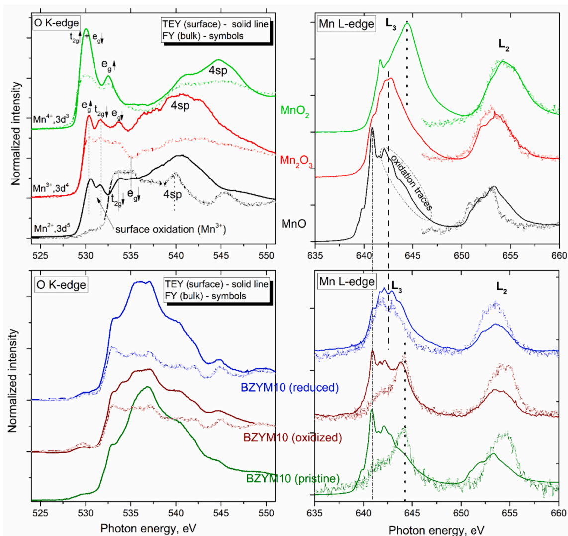
Fig. 12. Experimental NEXAFS spectra of the reference Mn oxide powders (top): MnO, \text{Mn}_2\text{O}_3 , \text{MnO}_2 , and the studied samples (bottom): BZYM10 pristine, BZYM10 oxidized, BZYM10 reduced. The spectra in solid line were recorded in the total electron yield (TEY) mode (surface-sensitive). The spectra acquired in the fluorescence yield (FY) mode (bulk-sensitive) are presented in symbols.
