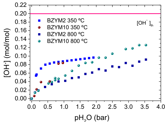
Fig. 10. a) Proton content registered for BZYM2 and BZYM10 as a function of p_{\text{H}_2\text{O}} at 350 ^{\circ}\text{C} and 800 ^{\circ}\text{C} ; (pink line indicates the theoretical proton content according to the nominal stoichiometry). (For interpretation of the references to colour in this figure legend, the reader is referred to the web version of this article.)
