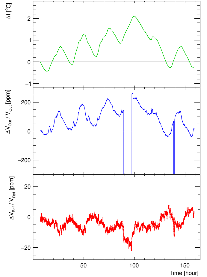
Figure 11: Voltage stability as function of time. The output voltage of one of the power supply modules is shown (middle) together with the reference voltage (bottom) in parallel with the ambient temperature recording (top). Note that the drops in the output voltage are caused by turning the power supply modules off. The reference voltage source remains turned on all the time.
