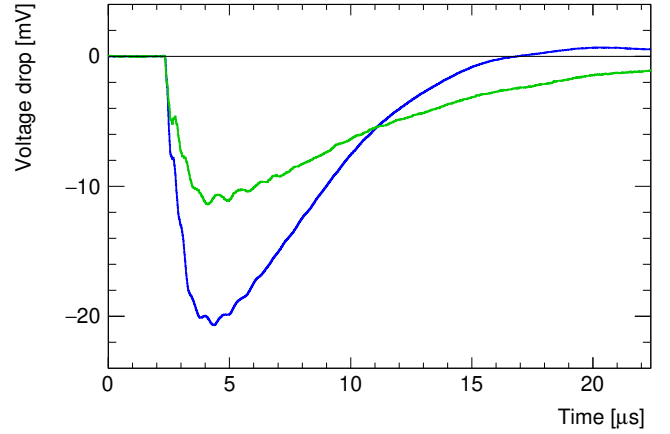
Figure 7: Voltage drop at the SiPM board (SiPM side): blue curve - voltage drop on the first prototype of the SiPM board with 8 \mu F total capacitance, green curve - voltage drop on an improved board with the capacitance increased up to 40 \mu F.
