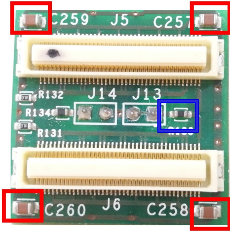
Figure 5: SiPM original board with LC filter. Red squares indicate the buffer capacitors while the blue square shows the filtering inductance, which was present in the original design of the board and was removed in later versions.
