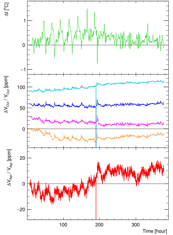
Figure 13: Voltage stability of the upgraded power supply. The output voltages of four typical power supply modules are shown (middle) together with the reference voltage (bottom) and the ambient temperature recording (top). Note that the whole power supply was off during some period of time. This is indicated by a drop in the output voltages at around 190 hours.
