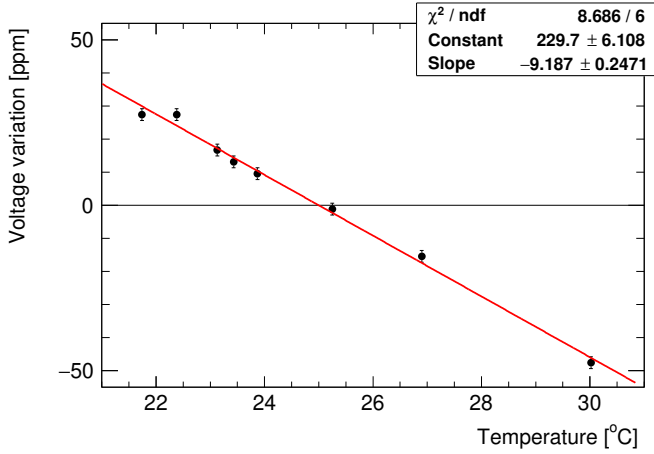
Figure 12: Temperature dependency of the power supply module after the upgrade.
