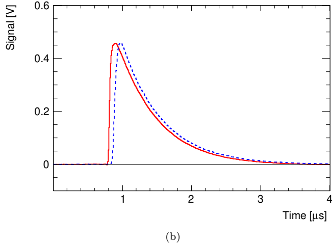
Figure 6: (a) Laboratory setup for a SiPM load simulation test and (b) comparison of the shapes of the Red Pitaya-generated voltage signal (solid red) versus the simulated sink current, converted back to voltage (dashed blue). The simulator consists of Red Pitaya signal generator, providing the exact copy of the SiPM signal and the fast voltage to current transformer loading the output of the power supply module. The voltage drop is measured at the output of the SiPM holder board and is fed back into the Red Pitaya oscilloscope.
