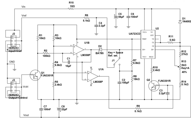
Figure 3: The schematics of a single module of the power supply
