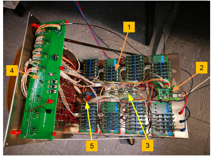
Figure 9: Assembled power supply: 1 - Power supply modules, 2 - Raspberry Pi, 3 - Port expander, 4 - Voltage monitoring board, 5 - Reference voltage board
