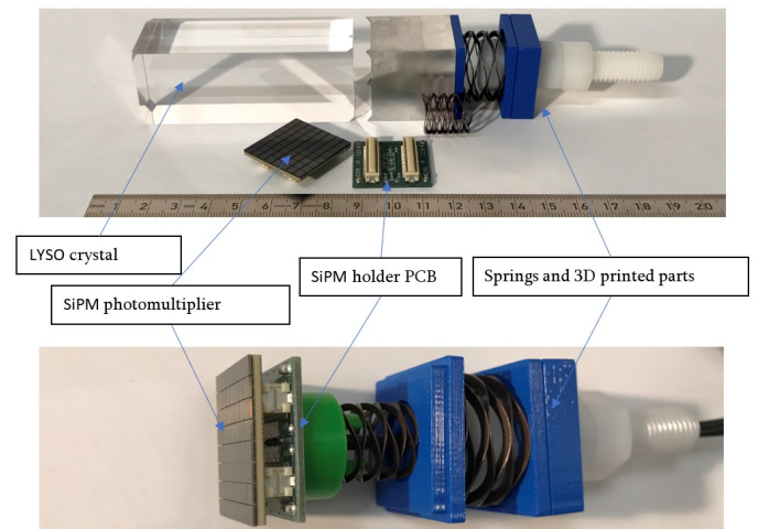
Figure 1: A single calorimeter module before assembly.
