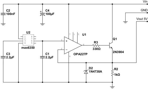
Figure 4: The schematics of a reference voltage source
