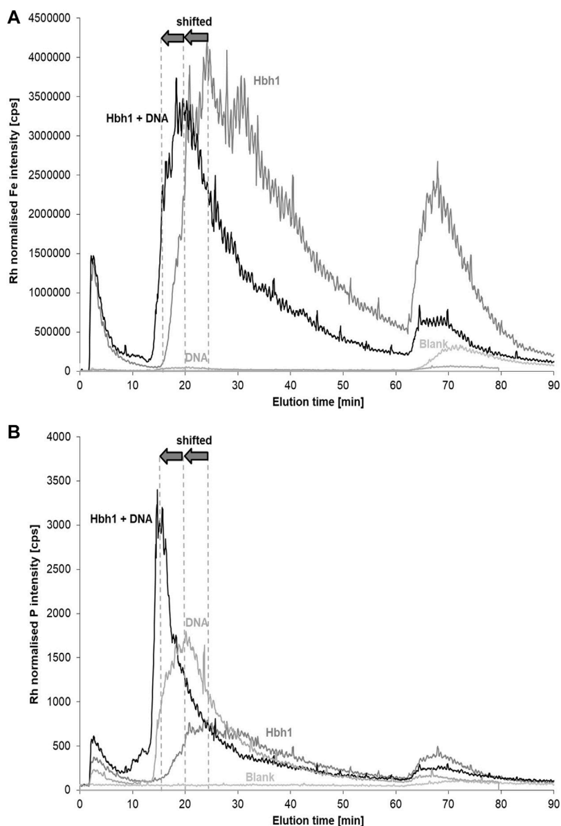
FIGURE 4 | Fractograms of a surface-water sample (Hbh1), calf-thymus DNA in deionized water, the surface-water sample spiked with CT DNA, and a deionized water blank monitoring Fe (A) and P (B). The carrier was 25 \mu\text{mol L}^{-1} NaCl and the membrane 1 kDa PES.
