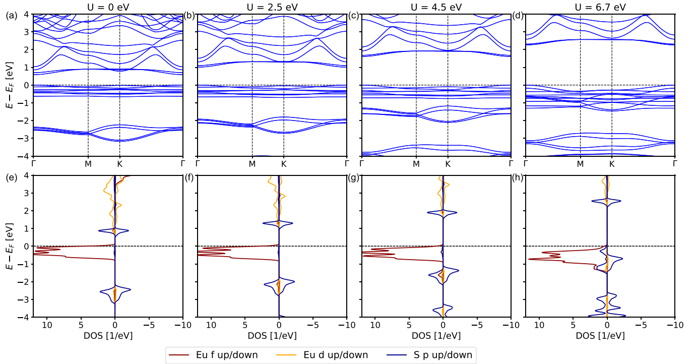
FIG. 2. Electronic structure of the H -phase \text{EuS}_2 monolayer as a function of Coulomb repulsion strength U . In (a)–(d) the band structures are shown for U = 0, 2.5, 4.5 , and 6.7 eV, respectively. In (e)–(h) the corresponding evolution of the spin-resolved density of states is shown. In (e)–(h) the left and right parts of the plots correspond to the majority and minority spins, respectively, while the densities of states of Eu f , Eu d , and S p states are shown with dark red, orange, and blue thin lines, respectively. While the dominance of the majority Eu f states at the Fermi level is evident, increasing U drives the hybridization of Eu f states with S p states. This has a drastic influence on the transport properties of the system, as discussed in the text.
