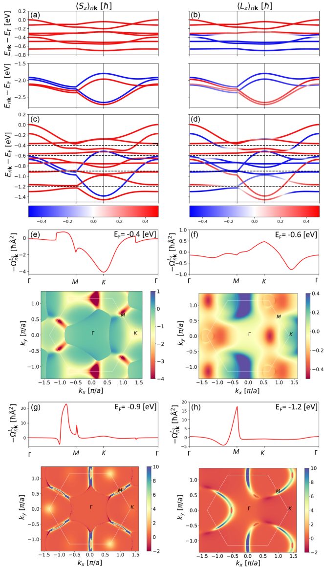
FIG. 4. Evolution of (a) and (c) the out-of-plane spin \langle S_z \rangle_{nk} and (b) and (d) orbital polarization \langle L_z \rangle_{nk} of occupied states in \text{EuS}_2 . (a) The occupied spin-up f states of Eu above -0.8 eV (top) and S p states in the region between -3 and -1.5 eV (bottom) for the case of U = 2.5 eV. Note that both groups of displayed states are isolated in energy from other states. (c) The hybridized group of occupied f and p states for the case of U = 6.7 eV which reside above -1.5 eV. (b) and (d) are analogous to (a) and (c). The value scales are indicated by the color bars at the bottom in units of \hbar . Horizontal dashed lines in (c) and (d) are guides to the eye marking the position of energy at -1.2 , -0.9 , -0.6 , and -0.4 eV. (e), (f), (g) and (h) Distribution of the orbital Berry curvature along high-symmetry lines for the indicated position of the Fermi energy, shown together with the distribution of the corresponding orbital Berry curvature in the Brillouin zone.
