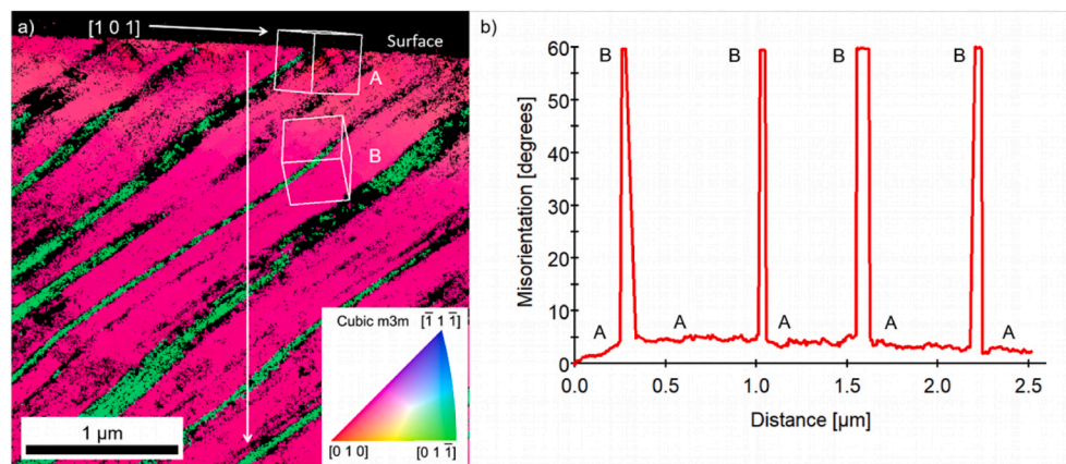
Fig. 3. a) TKD-IPF map of TEM foil cut along the wear direction shown by a white arrow above the surface of the TEM foil. The IPF references the surface normal direction during wear; this direction is the same as in Fig. 2 b) Point to origin misorientation plot along the white arrow pointing downwards in a). The crystal orientations are shown for A: parent grain, B: twinned region.
