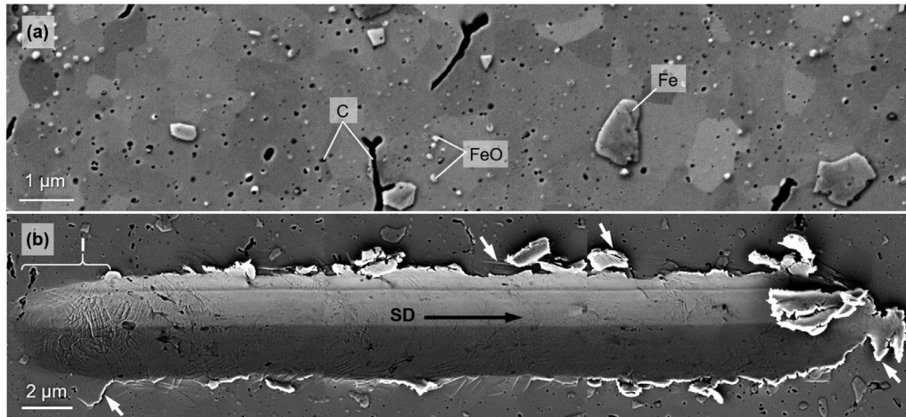
Fig. 1. SEM images of the cementite surface (a) before and (b) after the single-pass wear experiment. (a) Initial sample microstructure with iron, iron oxide, and graphite inclusions that remain after spark plasma sintering. (b) Combined (of three images at the different wear track regions) image of the single-pass wear track with a black arrow showing the sliding direction (SD). White arrows mark wear features: a single crack event, plastic slip traces, wear debris, and pile-up at the wear track end. The white bracket denotes the indentation region “I”.
