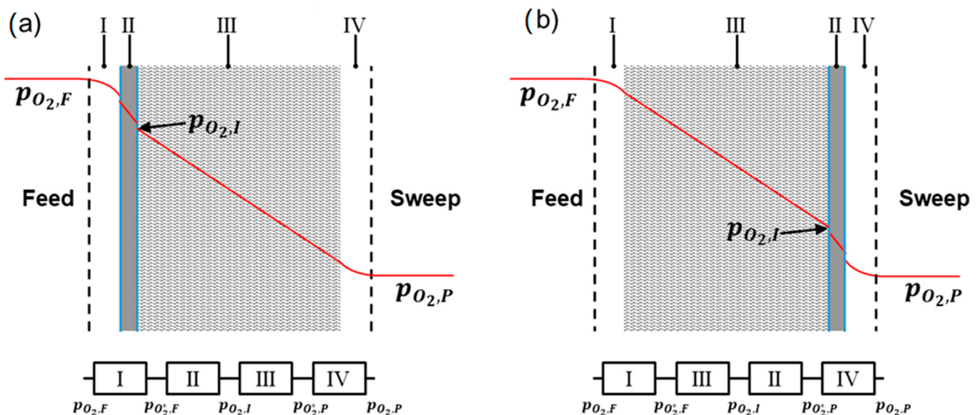
Figure 1. Partial pressure of O_2 (red line) in a cross section of an asymmetric membrane; (a) membrane operated with support on the permeate side (SP); (b) membrane operated with support on the feed side (SF); the flow resistance can also be expressed as linear connection of resistors. (adapted from [15]).
