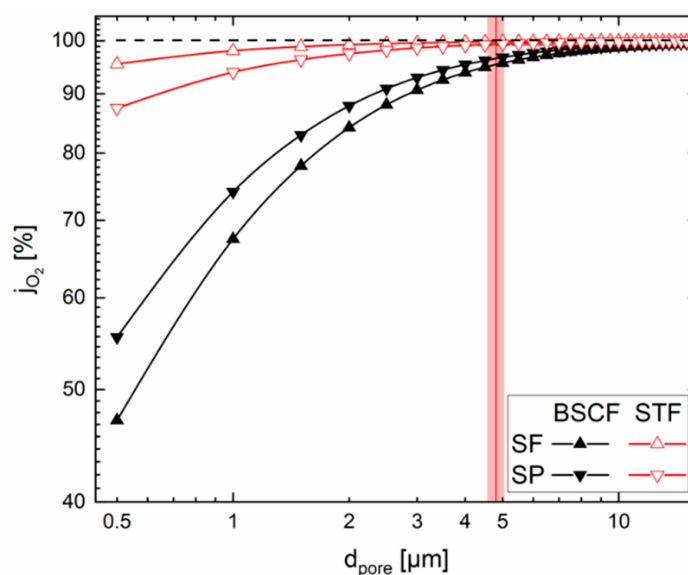
Figure 4. Influence of the pore diameter; vertical red line and the red area show the value used in this work and the \pm 5\% deviation of the sensitivity analysis.
