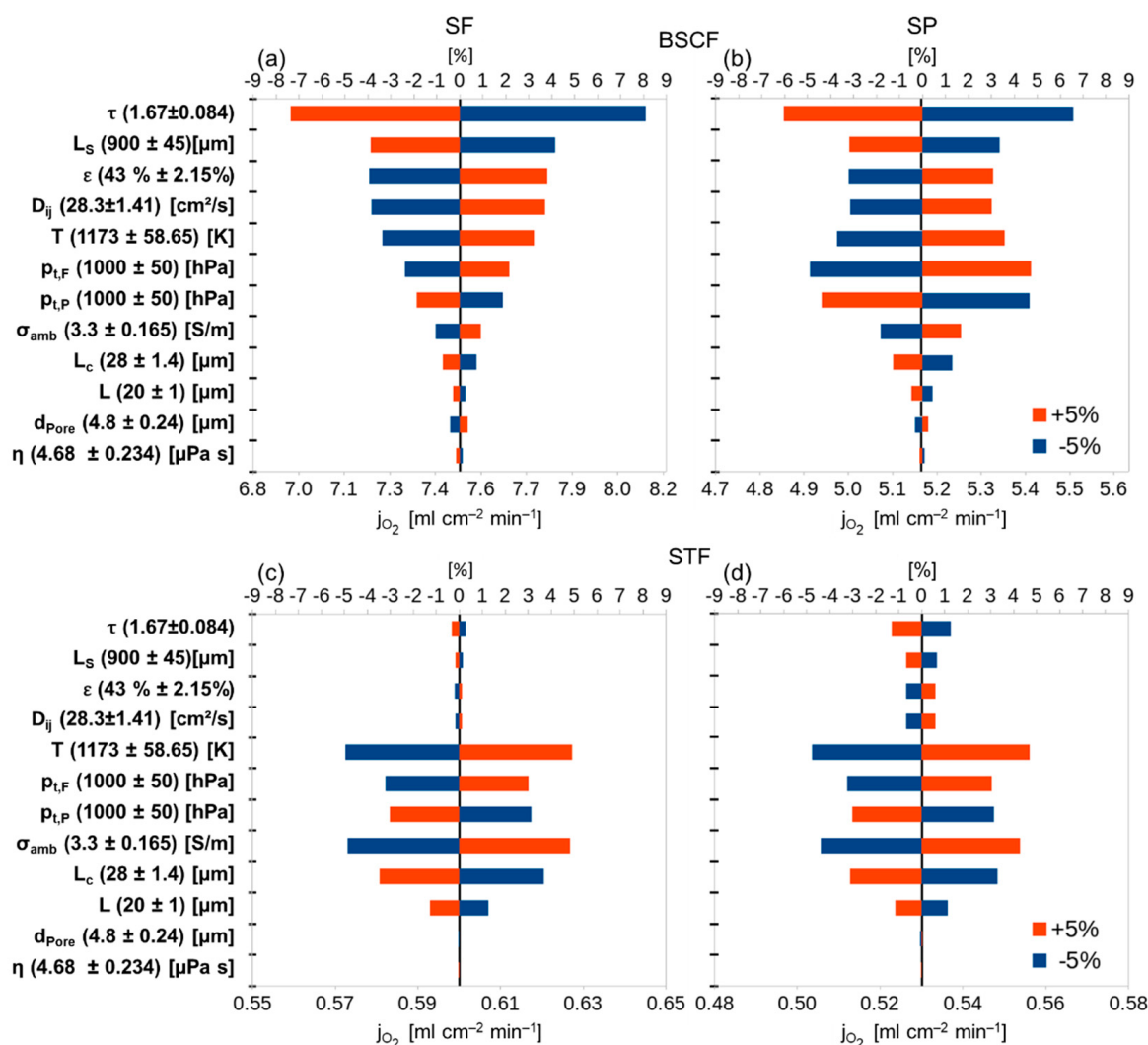
Figure 3. Sensitivity analysis: effect of varying single parameters by \pm 5\% of their original value on the total result of the calculated result. Upper scale: percentage deviation of the original flux. Lower scale: fluxes calculated with the given values from Table 1. (a) BSCF support on feed side (SF), (b) BSCF support on permeate side (SP), (c) STF SF, (d) STF SP.
