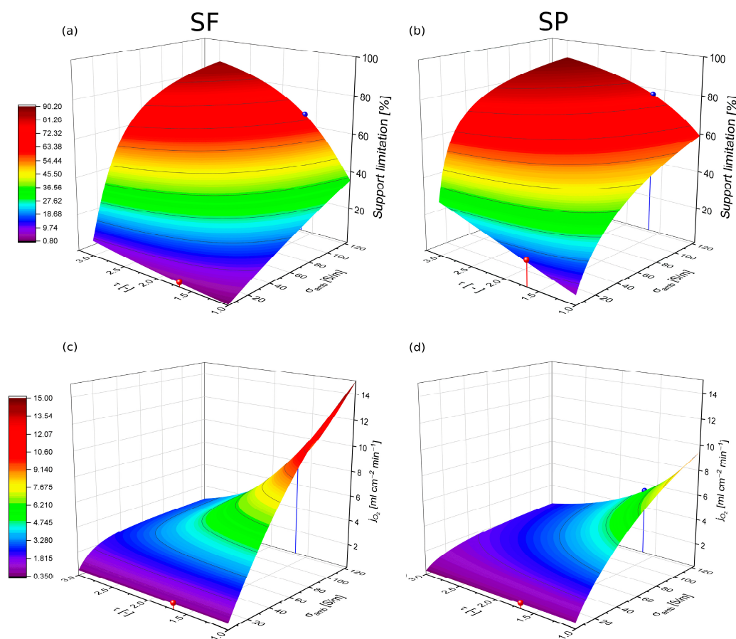
Figure 6. Influence of tortuosity and ambipolar conductivity on the support limitation (a,b) and the flux (c,d). The red and the blue dots represent the parameter sets investigated in the sensitivity analysis.
