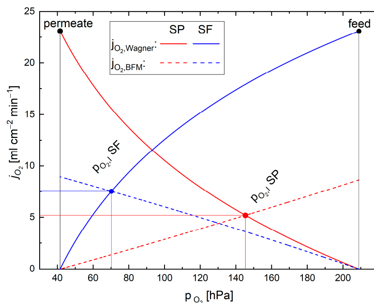
Figure 2. Flux vs. partial pressure curve and resulting flow in membrane and support for support on feed side (SF) and support on permeate side (SP) modes for the example of BSCF. The resultant flux through the entire system as well as the partial pressure at the interface can be seen at the intersection of the respective curves. For the calculation of the fluxes, one pressure is kept constant while the other is varied towards the feed or permeate pressure depending on the operation mode (Wagner or BFM).
