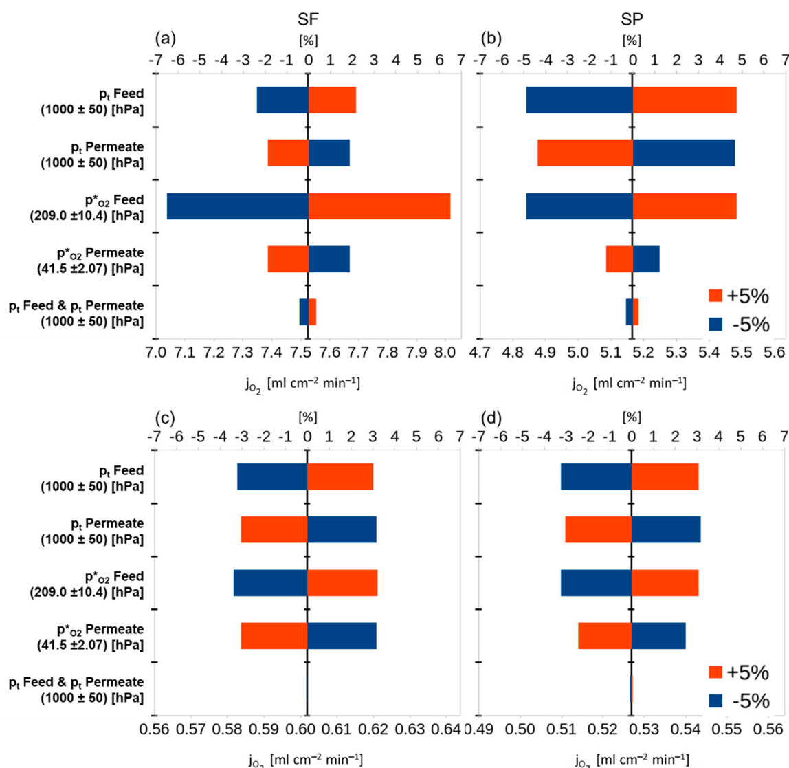
Figure 5. Detailed sensitivity study of the effect of total and partial pressures on the feed and permeate sides for BSCF (a,b) and STF (c,d).
