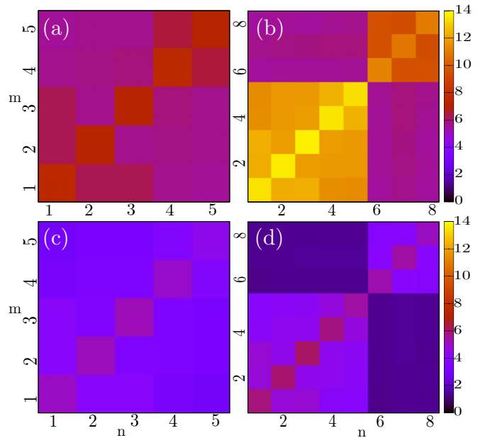
FIG. 5. Effective U_{mn} Coulomb matrix elements (in eV) in the isolated \text{MnO}_2 chain including (a) only \text{Mn}(d) electrons and (b) \text{Mn}(d) and \text{O}(p) electrons in the correlated subspace. Panels [(c), (d)]: same quantities for the supported \text{MnO}_2 chain. [Note, \text{O}(s) electrons, which belong to the correlated space in panel (d), are not shown.]
