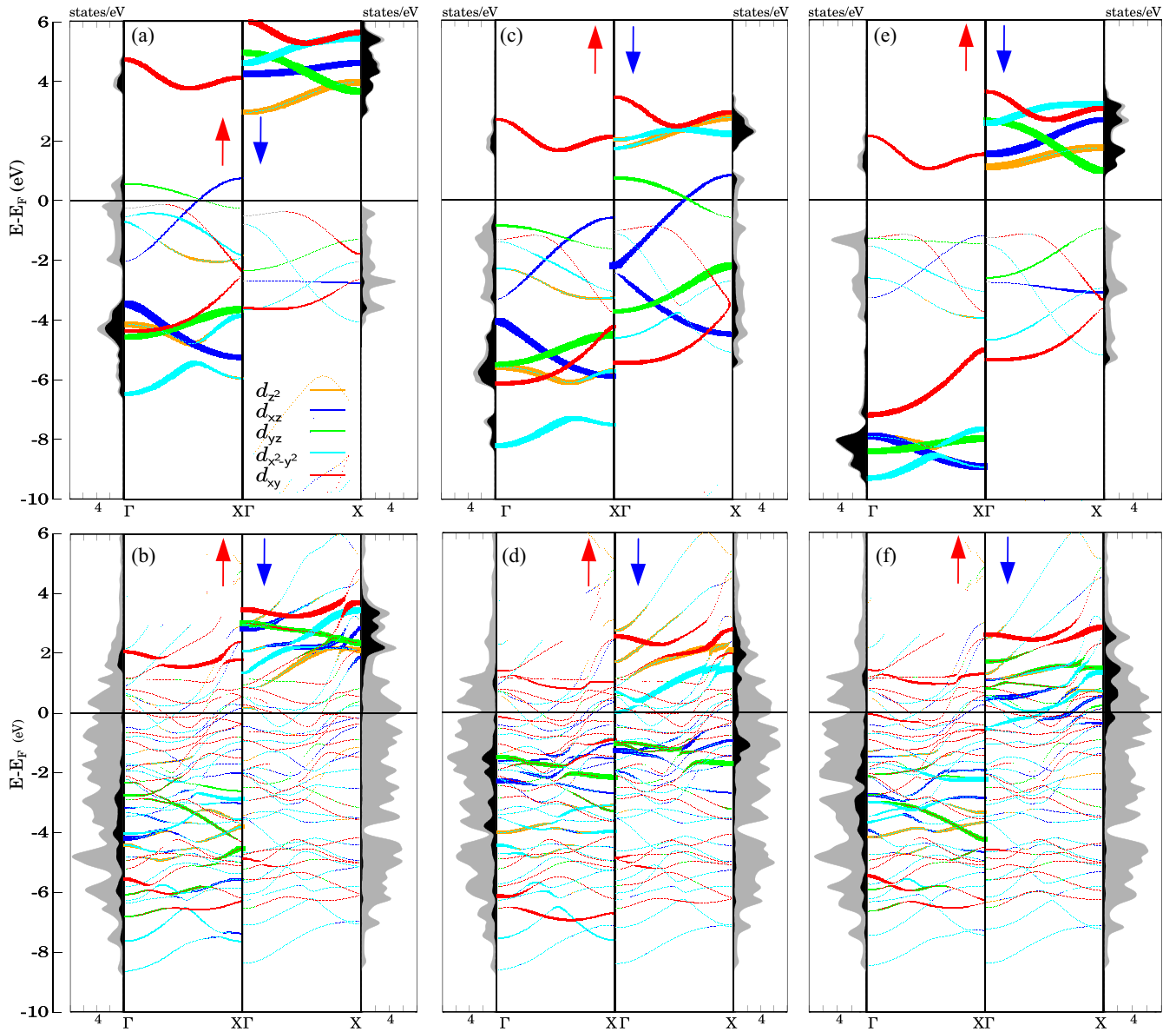
FIG. 4. The same information as in Fig. 2 is provided here for free-standing planar (top panels) and supported (bottom panels) \text{XO}_2 chains with \text{X} = \text{Mn} [(a), (b)], \text{Co} [(c), (d)], and \text{Fe} [(e), (f)].
