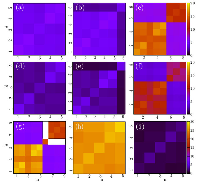
FIG. 3. Screened Coulomb matrix elements U_{mn} ( \uparrow\uparrow spin channel) in eV for the \text{NiO}_2 chain for selected orbitals screened by the remaining electrons. For the free-standing C1 configuration, the selection is: (a) d (indices ordered as 1 – d_z^2 , 2 – d_{xz} , 3 – d_{yz} , 4 – d_{x^2-y^2} , and 5 – d_{xy} ), (b) d and O( s ) (index 6), and (c) d and O( p ) orbitals (indices ordered as 6 – p_z , 7 – p_x and 8 – p_y ). [(d)–(f)] shows the same information as [(a)–(c)] but for the free-standing C2 configuration. In the bottom row, bare Coulomb matrix elements of (g) free-standing C1 and (h) Ir-supported \text{NiO}_2 , which we take as reference values. (i) For Ir-supported \text{NiO}_2 , U_{mn} elements of the d orbital screened by the rest of electrons. Note the different color scale for the panels (g) to (i).
