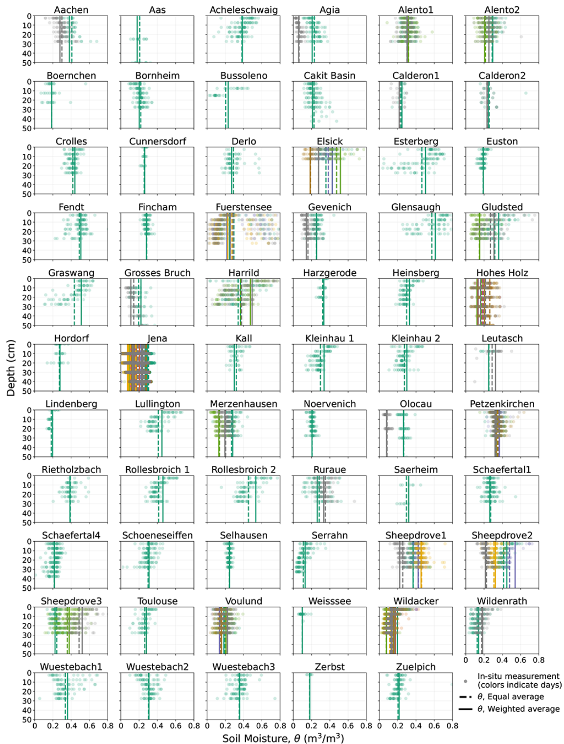
Figure A4. Soil profiles of the in situ calibration data for the COSMOS-Europe sites. The weighted average soil moisture values are also shown. The varying colors indicate the different sampling dates.
