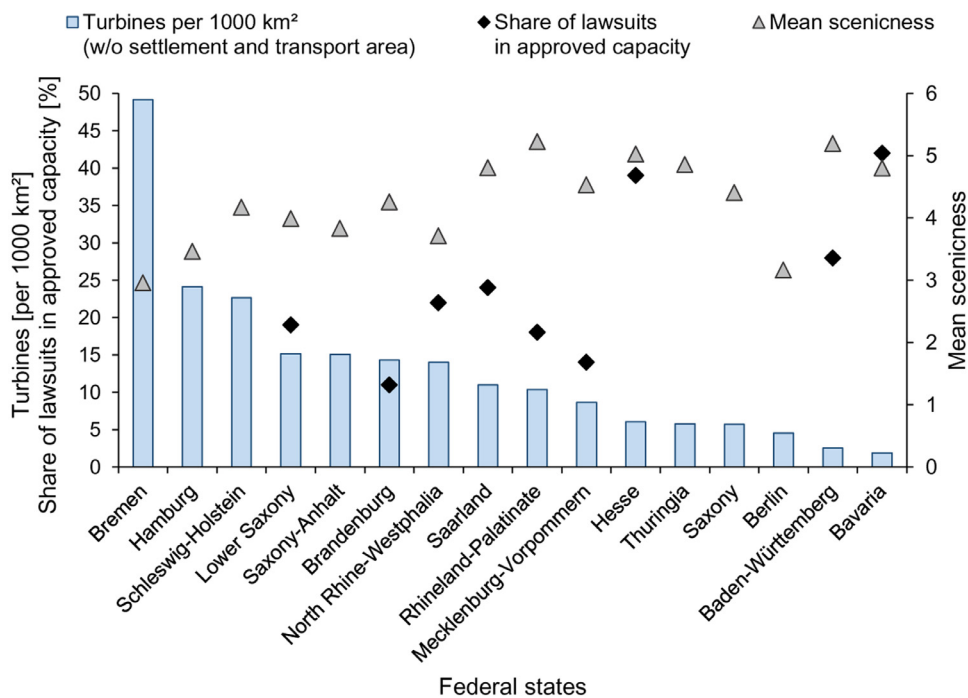
Fig. 3. Specific number of turbines, share of wind turbines in total licensed capacity subject to lawsuits, and mean scenicness of landscapes in the sixteen German federal states. The federal states are ordered from the highest specific number of turbines (Bremen) to the lowest (Bavaria). The share of wind turbines in total licensed capacity subject to lawsuits has been determined by a survey with 89 companies in 14 of the sixteen federal states [55]. However, lawsuits have not been reported for all federal states [55].
