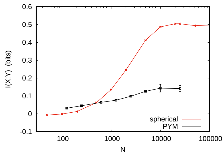
Figure 3. Estimated mutual information (in bits) of N -tuples of independent and identically distributed random subsamples from two distributions given in [22]. The data for “PYM”, originally due to [24], consist of 250,000 pairs (x, y) with binary y with p(y = 0) = p(y = 1) = 1/2 , and x being uniformly distributed over 4096 values. Thus each x -value is realized \approx 60 times, and we classify them into 5 classes depending on the associated y -values: (i) very heavily biased toward y = 1 , (ii) moderately biased toward y = 1 , (iii) y -neutral, (iv) moderately biased toward y = 0 , and (v) heavily biased toward y = 0 . When we estimated conditional entropies H(Y|X) for randomly drawn subsamples, we kept this classification and choose a_y accordingly: For class (iii) we used a_0 = a_1 = 1 , for class (ii) we used a_1 = 1, a_0 = 4 , for class (i) we used a_1 = 1, a_0 = 7 , for class (iv) we used a_1 = 4, a_0 = 1 , and finally for class (v) we used a_1 = 7, a_0 = 1 . The data for “spherical”, originally due to [21], consist of 50,000 (x, y) pairs. Here, Y is again binary with p(y = 0) = p(y = 1) = 1/2 , but X is highly non-uniformly distributed over \approx 4000 values. Again we classified these values as y -neutral or heavily/moderately biased toward or against y = 0 and used this classification to choose values of a_y accordingly.
