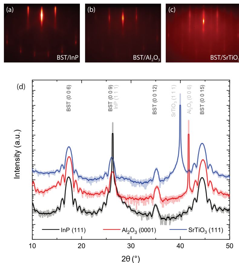
Figure 1. (a–c) RHEED patterns and (d) symmetric 2\theta - \omega diffractograms of 10 nm BST on InP (111), \text{Al}_2\text{O}_3 (001), and \text{SrTiO}_3 (111) substrates, respectively. The presented RHEED patterns are recorded along \langle 2\bar{1}10 \rangle and are representative for other BST films deposited on these substrates. The XRD data have been given an offset for clarity. The solid (semi-transparent) lines present the smoothed (real) data. The Miller indices of the different crystallographic planes ( hkl ) are indicated. The diffractograms and the sharp streaks observed in the RHEED patterns confirm the crystallinity of all three BST films in the out-of-plane direction.
