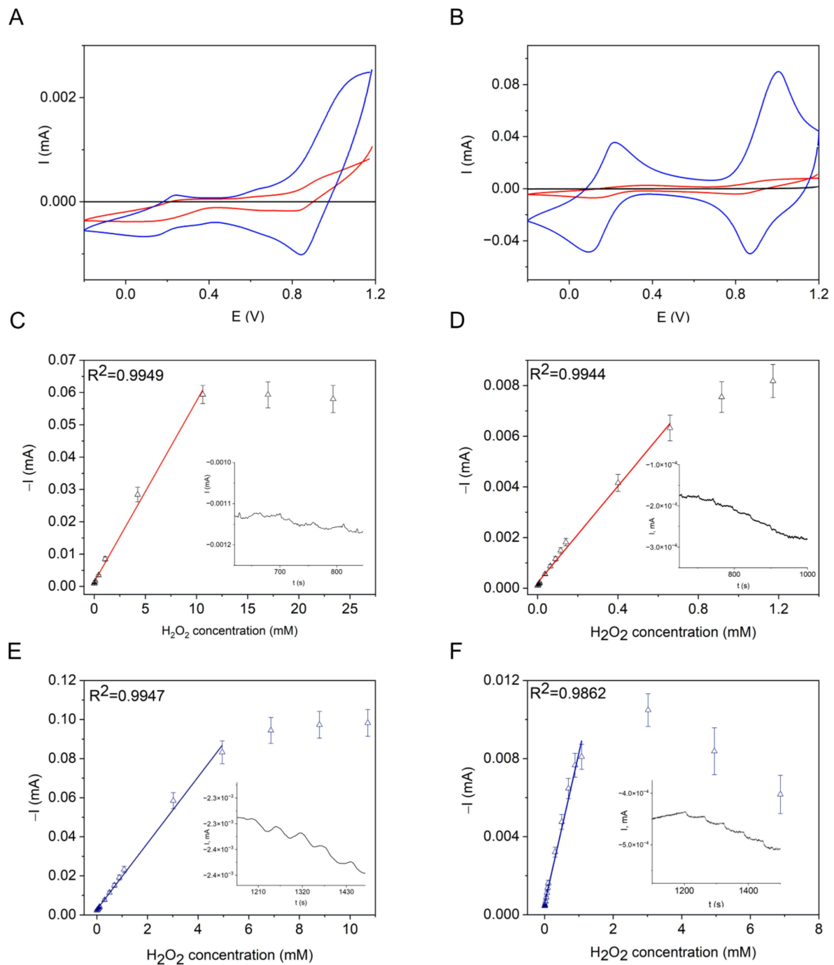
Figure 6. CVs of (A) GCE/Mn-PB NCPs/Nafion, (B) GCE/PB NCPs/Nafion in the deoxygenated solutions, at pH 3 (blue lines) and pH 7.4 (red lines), 25 mV s -1 , unmodified GCE at pH 3 (black lines). (C–F) Calibration curves of the electrodes modified with NCPs: (C,D) GCE/Mn-PB NCPs/Nafion, −0.05 V, and (E,F) GCE/PB NCPs/Nafion, 0 V, at pH 3 (C,E) and pH 7.4 (D,F), inserts show the amperometric response in the low concentration range.
