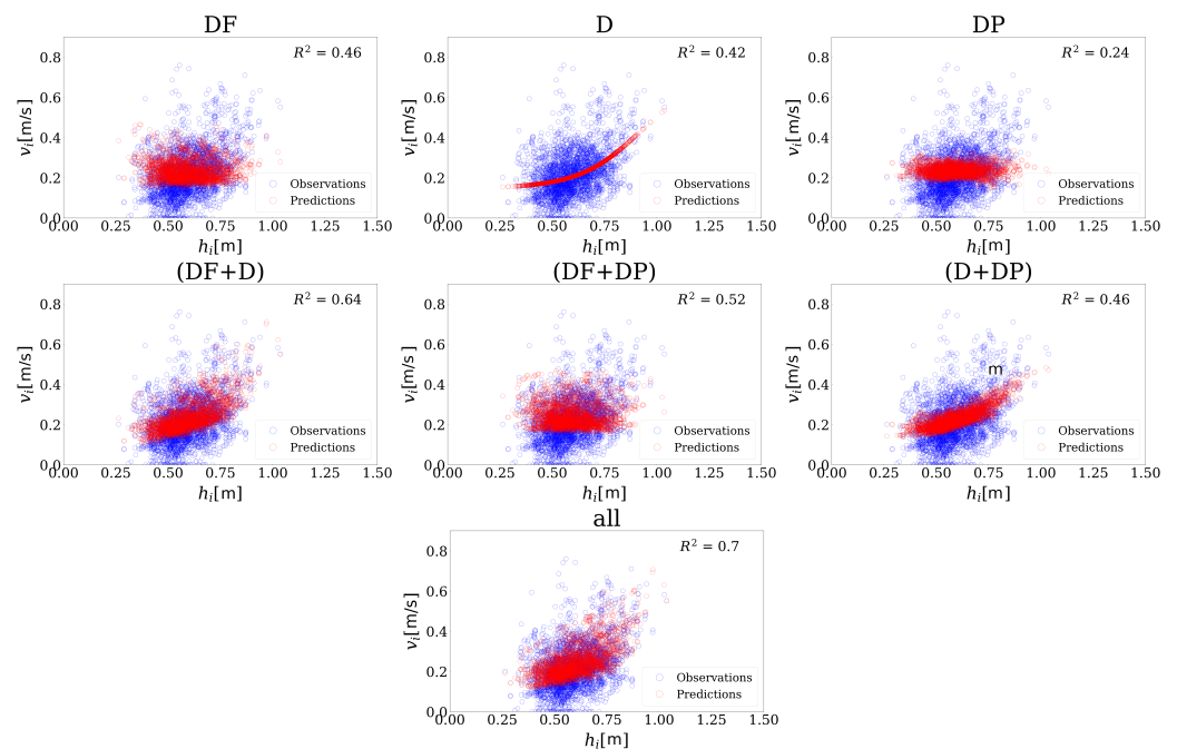
Figure 8. Examples of speed predictions from testing the neural networks ( D , DF , (DF + D) , (DF + DP) , (DP + D) , (all) ) using UX, N = 20, 24, 30 samples. As observed in the actual data (in blue), the speed values for given headway distances tend to be close to the observed values when we combine DF and D as inputs to the FFNN algorithm or when we have more input features ( all ). The R^2 values on the top-right of the figure are calculated to compare the variability of the estimated speed.
