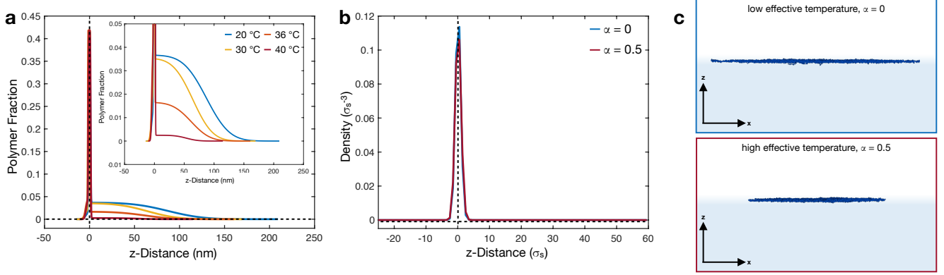
Figure 5: Structure of ULC microgels at liquid interfaces. a Results of the fits of the experimental data for the ULC D3 microgels. Inset: Zoom of polymer fraction profiles. b Density profiles of simulated ultra-low cross-linked microgels at different effective temperatures, corresponding to \alpha = 0, 0.5 . Horizontal and vertical dashed lines are guidelines for the eyes and represent zero polymer fraction and zero z-distance from the interface, respectively. Negative values of z represent the air phase and positive values represent the water phase. c Simulation snapshots showing the side perspective of an adsorbed ULC microgel for \alpha = 0, 0.5 . Solvent particles are not shown for visual clarity.
