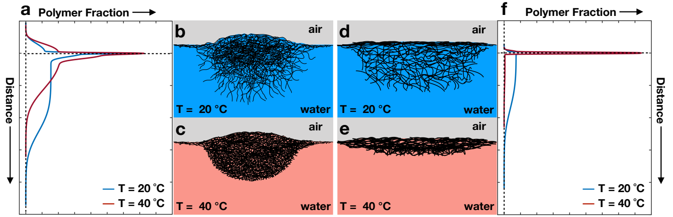
Figure 3: Sketch of the adsorbed microgels. Panel a shows the vertical profiles of standard microgels and f the vertical profiles of ULC microgels below and above the VPTT. Their corresponding shapes are outlined in b-e . The shapes are based on the combination of our polymer fraction profiles, simulations and AFM measurements at the liquid-solid interface from the literature. 25
