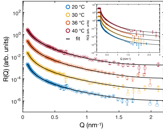
Figure 4: Reflectivity curves of ULC D3 microgels at different temperatures. Reflectivity, R(Q) , versus momentum transfer, Q , at the air-ACMW interface. The fits are shown by continuous lines. Inset: Reflectivity curves at air-D 2 O interfaces. The curves are shifted in y-direction for clarity. The unshifted curves are shown in Supplementary Figs. 6c. The error bars represent the statistical errors on R(Q) .
