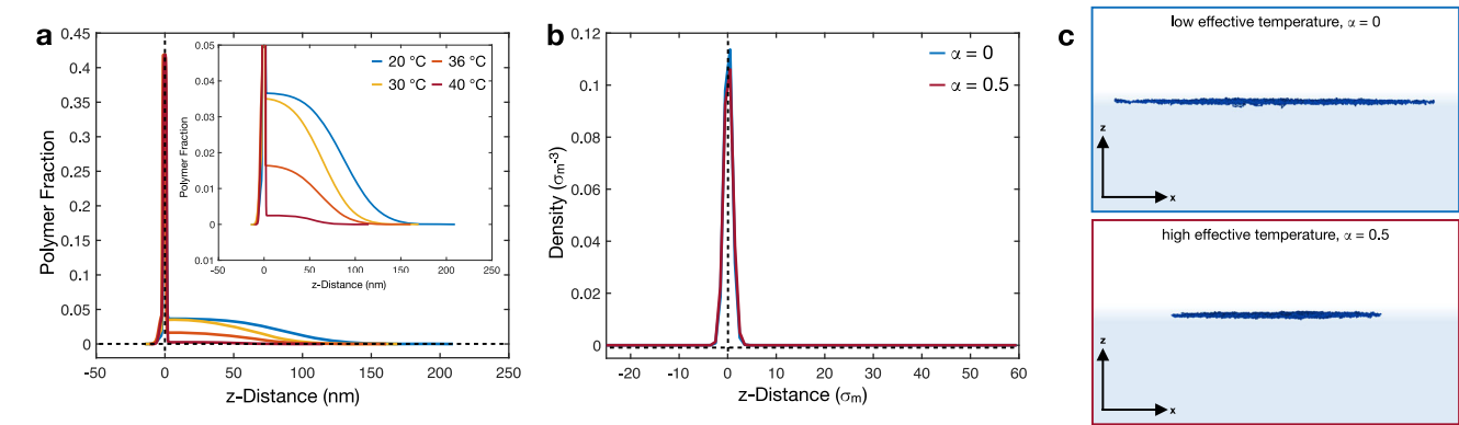
Fig. 5 Structure of ULC microgels at liquid interfaces. a Results of the fits of the experimental data for the ULC D3 microgels. Inset: Zoom of the polymer fraction profiles. b Density profiles of simulated ultra-low cross-linked microgels at different effective temperatures, corresponding to \alpha = 0 , and 0.5. Horizontal and vertical dashed lines are guides to the eyes and represent zero polymer fraction and zero z -distance from the interface, respectively. Negative values of z represent the air phase and positive values represent the water phase. c Simulation snapshots showing the side perspective of an adsorbed ULC microgel for \alpha = 0, 0.5 . Solvent particles are not shown for visual clarity.
