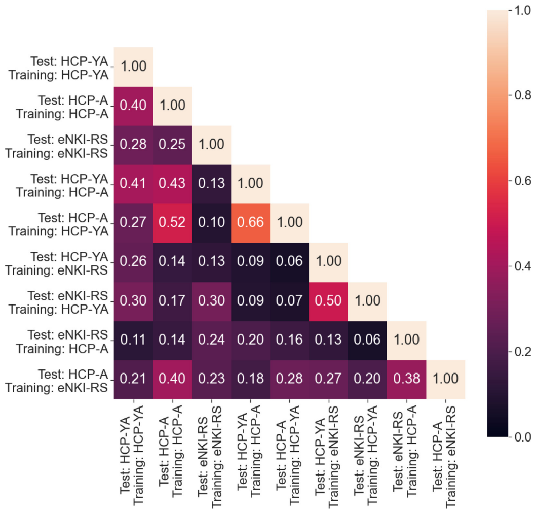
Fig. 10. Correlation between within-dataset and cross-dataset prediction patterns of HCP-YA fluid cognition, HCP-A fluid cognition, and eNKI-RS WASI-II intelligence. Each box shows the Pearson's correlation between one pair of prediction patterns, average across all 5 atlas options.
