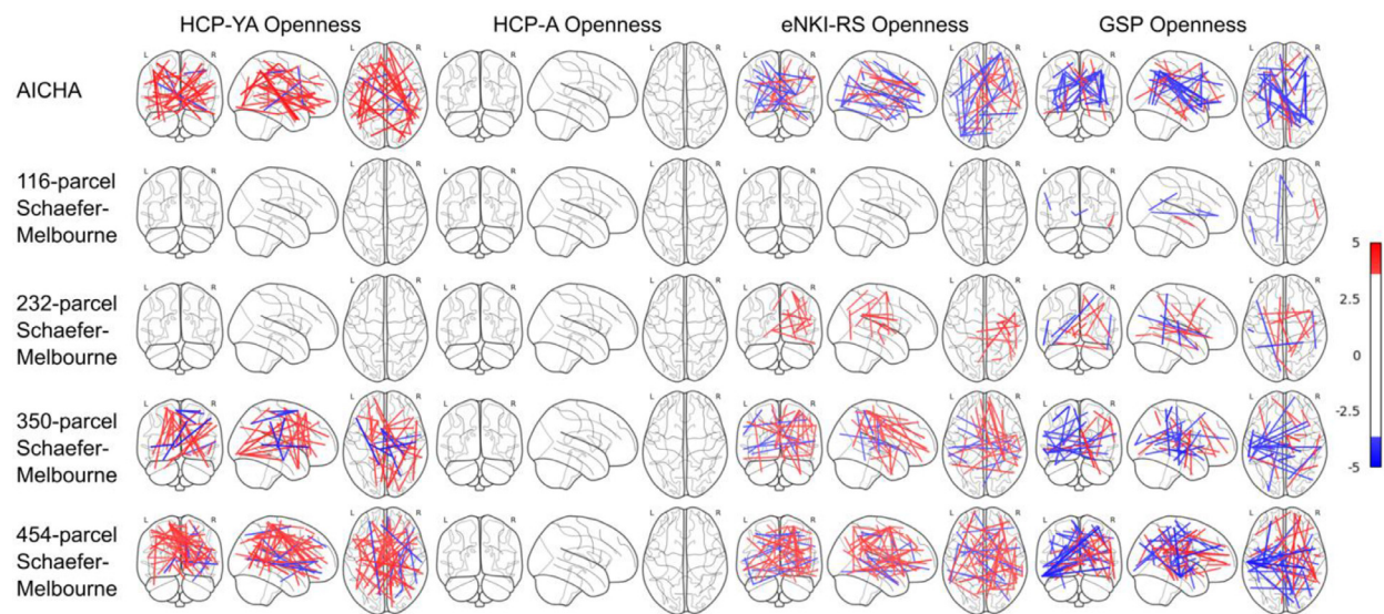
Fig. 7. Haufe transformed patterns of HCP-YA, HCP-A, eNKI-RS and GSP openness measures, respectively. Each row shows the patterns for predictions using one specific parcellation. In each plot, only significant edges with the top 0.05% z-score normalized absolute values were shown, with positive edges shown in red and negative edges in blue.
