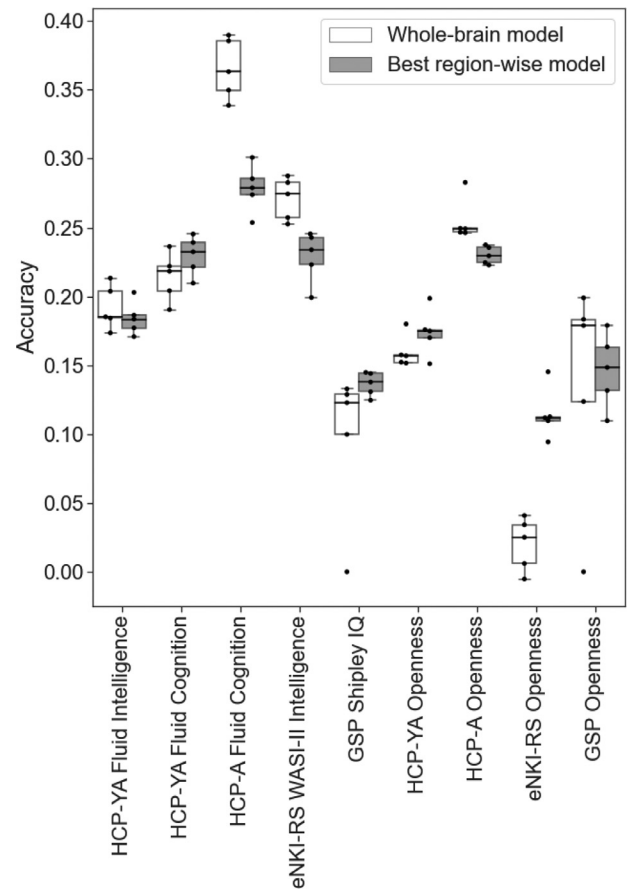
Fig. 2. Prediction accuracies (Pearson's correlation between predicted and observed values) for each psychometric variable using the whole-brain model (white boxes) and best region-wise model (black boxes) with different atlases. For each psychometric variable and each atlas, only the region-wise model with the highest prediction accuracy (i.e., the best region-wise model) was included. Black bars inside the boxes represent the median accuracy value across different parcellations.
