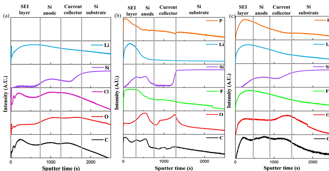
Figure 3. Sputter-etched TOF-SIMS spectra of Si electrodes after GITT measurements in \text{LiClO}_4 -based electrolytes (a), \text{LiPF}_6 in PC solvents (b), and \text{LiPF}_6 in EC/EDC/DMC solvents (c).
