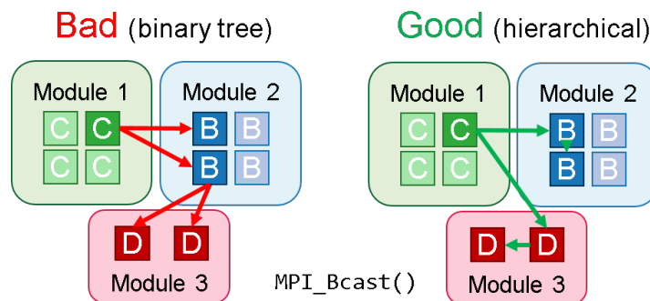
Figure 4 - Principle behind the MSA-aware optimisation of MPI collectives
