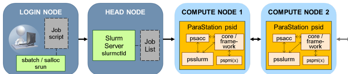
Figure 5 - Control flow for submitting a job to the Slurm scheduler when using ParaStation Management. The ParaStation Daemons ( psid ) completely replace the node-local Slurm daemons and directly interact with the Slurm control daemon.
