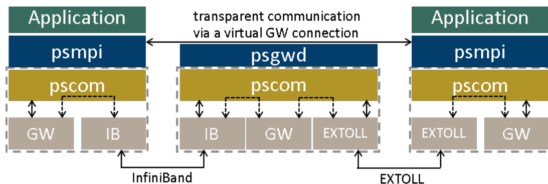
Figure 3 - Overview of the network bridging within ParaStation MPI. This relies on a gateway-base approach and is implemented as part of the pscom library
