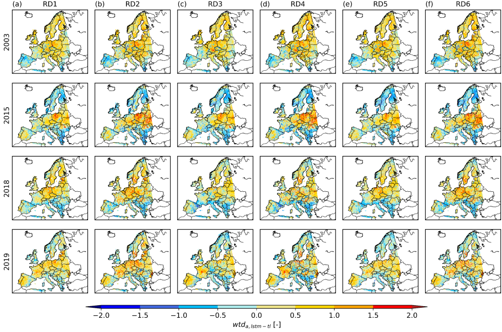
Figure 4.4: Spatial distribution of yearly averaged wtd_{a,ism-tl} over the European continent for the recent drought years 2003, 2015, 2018 and 2019. The anomalies were calculated from (a) RD1; (b) RD2; (c) RD3; (d) RD4; (e) RD5; and (f) RD6.
