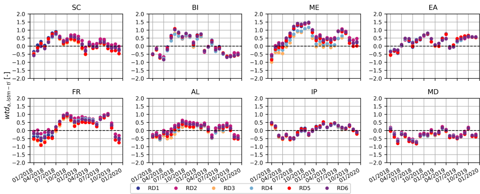
Figure 4.5: Regionally averaged wtd_{a,ism-tl} from RD1-6 over eight PRUDENCE regions for the 2018-2019 period. The black dashed lines indicate wtd_a = 0 . A long time period with wtd_a > 0 corresponds to a dry event while a long time period with wtd_a < 0 corresponds to a wet event.
