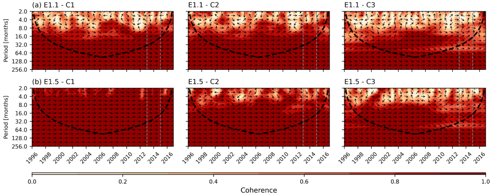
Figure B.3: Results of wavelet coherence analysis on the regionally averaged wtd_a time series for the wtd categories C1 to C3 in SC, which were derived from the TSMP-G2A data set and the results of the LSTM networks of: (a) E1.1: pr_a ; and (b) E1.5: pr_a and \theta_a .
