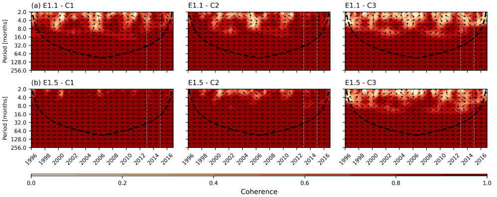
Figure 3.8: Results of wavelet coherence analysis on the regionally averaged wtd_a time series for the wtd categories C1 to C3 in ME, which were derived from the TSMP-G2A data set and the results of the LSTM networks of: (a) E1.1: pr_a ; and (b) E1.5: pr_a and \theta_a . The training, validation and testing periods are separated by gray dashed lines.
