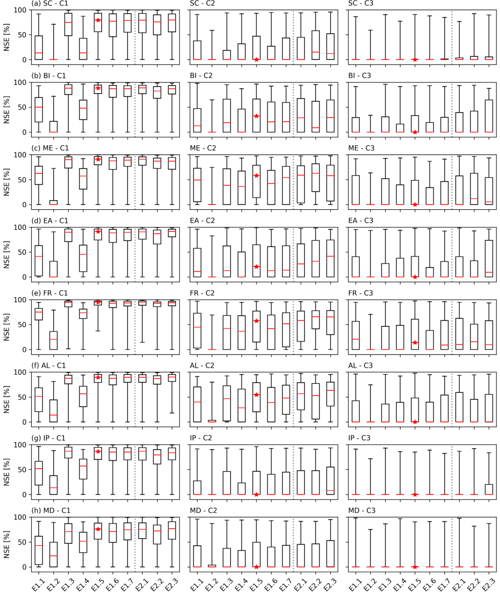
Figure 3.4: Box plots of test NSE scores achieved by the LSTM networks of E1 and E2: E1.1: pr_a ; E1.2: ET_a ; E1.3: \theta_a ; E1.4: pr_a and ET_a ; E1.5: pr_a and \theta_a ; E1.6: ET_a and \theta_a ; E1.7: pr_a , ET_a and \theta_a ; E2.1: pr_a , \theta_a and SWE_{scaled} ; E2.2: pr_a , \theta_a at the selected pixels and adjacent pixels; and E2.3: pr_a , \theta_a at the selected pixels close to rivers and rs_a at the adjacent pixels. (a) – (h) show the comparison of the box plots at the selected pixels belonging to the wtd categories C1 to C3 in each PRUDENCE region. The box plots show the ranges of the NSE scores from the first quartile to the third quartile; the red lines indicate the medians of the NSE scores; and the upper and lower ends represent the maximum and minimum values of the NSE scores, respectively. The medians of the NSE scores obtained by the LSTM networks of E1.5 are marked with red stars. The box plots for E1 and E2 are separated by gray dotted lines.
