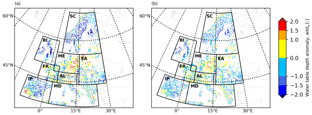
Figure B.2: European wtd_a maps for August 2015 (i.e., in the testing period) derived from (a) the TSMP-G2A data set and (b) the results from the LSTM networks of E1.1 ( pr_a ).
