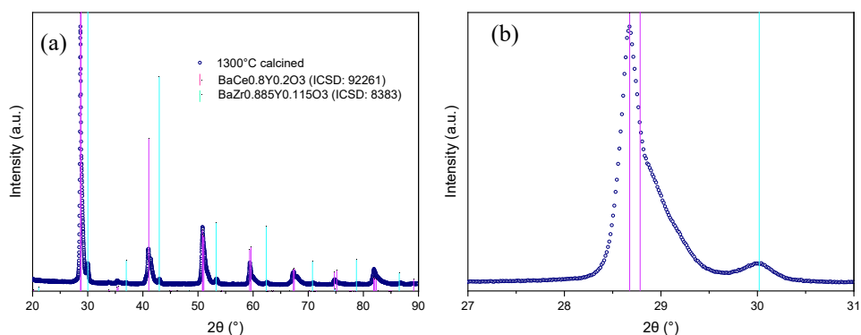
Figure 2.1 XRD patterns of the mixed powders after 1300 °C / 5 h calcination. (b) represents the magnified 2θ angle range in (a) covering the peak with the highest intensity. The legends in (a) also apply to (b).
