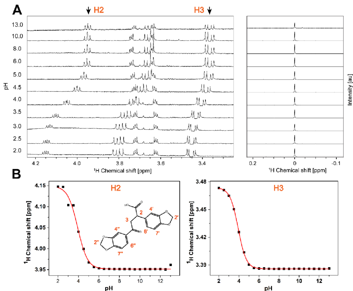
Figure 6. Determination of the pKa value for 7.44 by 1 H NMR. (A) 1 H NMR spectra of 200 μM of 7.44 measured from pH 2 to 13 at 298 K at 600 MHz. Sodium 2,2-dimethyl-2-silapentane-5-sulfonate (DSS) was used for chemical shift referencing and calibrated to a zero ppm value. (B) Titration curves obtained from the 1 H chemical shifts of the protons H2 and H3 as a function of pH. The pKa values were calculated using the Henderson-Hasselbalch equation 25 , yielding a pKa value of 3.99 \pm 0.01 and 3.93 \pm 0.01 of the carboxylic group as indicated by proton H2 and H3, respectively.
