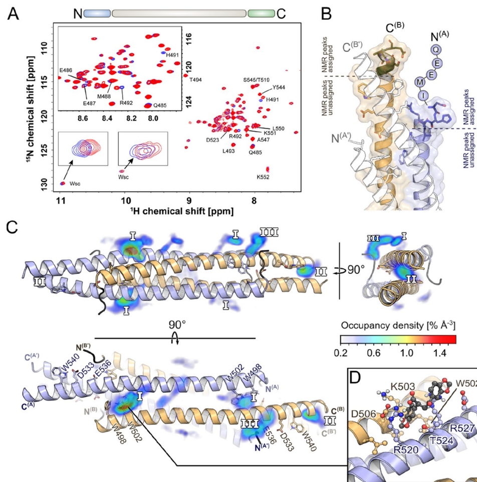
Figure 5. TROSY-HSQC NMR experiments of ^2\text{H} , ^{15}\text{N} , ^{13}\text{C} -labeled NHR2 in the absence and presence of 7.44. (A) 2D ^1\text{H} - ^{15}\text{N} TROSY-HSQC spectra of 47 \mu\text{M} of apo NHR2 (blue) and in complex with 2 mM of 7.44 (red). Both spectra were recorded at 60 ^\circ\text{C} on a 750 MHz spectrometer for about 19 h each and illustrate the changes in amide proton and nitrogen chemical shifts induced in NHR2 upon binding of 7.44. 32% of amide signals from the N- (light blue; residues Q485 to D495, T519) and C- (light green; residues Y544 to K552) terminus were unambiguously assigned (depicted above the spectra); these residues are labeled with a single-letter code (see also panel B for the location). Note that the first five (QEEMI) and last four (DLKK) amino acids were also assigned but are not shown in the crystal structure. (B) Chemical shift perturbations (CSPs) of residues Q485 to L493 (blue) upon addition of 7.44 mapped onto the NHR2 crystal structure (PDB ID 1WQ6). Residue R492, which shows the highest CSP, is associated with three hot spot residues (see text). (C) Occurrence propensities of 7.44 interacting with the NHR2 tetramer from MD simulations; the densities are mapped around the NHR2 crystal structure (PDB ID 1WQ6). Assigned residues at the termini showing CSP are colored in black. The side chains of the previously identified hot spots are shown as sticks in the figure. The preferred binding epitopes with the highest densities are labeled as I, II, and III. Identical binding epitopes due to the internal symmetry of the NHR2 tetramer are labeled identically. Here, ligands binding to epitope I and II form interactions with the hot spots W502 and W540, respectively. (D) Representative binding pose of 7.44 in epitope I. The 1,3-benzodioxole moiety inserts in between the helices, close to the hot spot residue W502. Identical binding poses are observed for all epitopes I.
