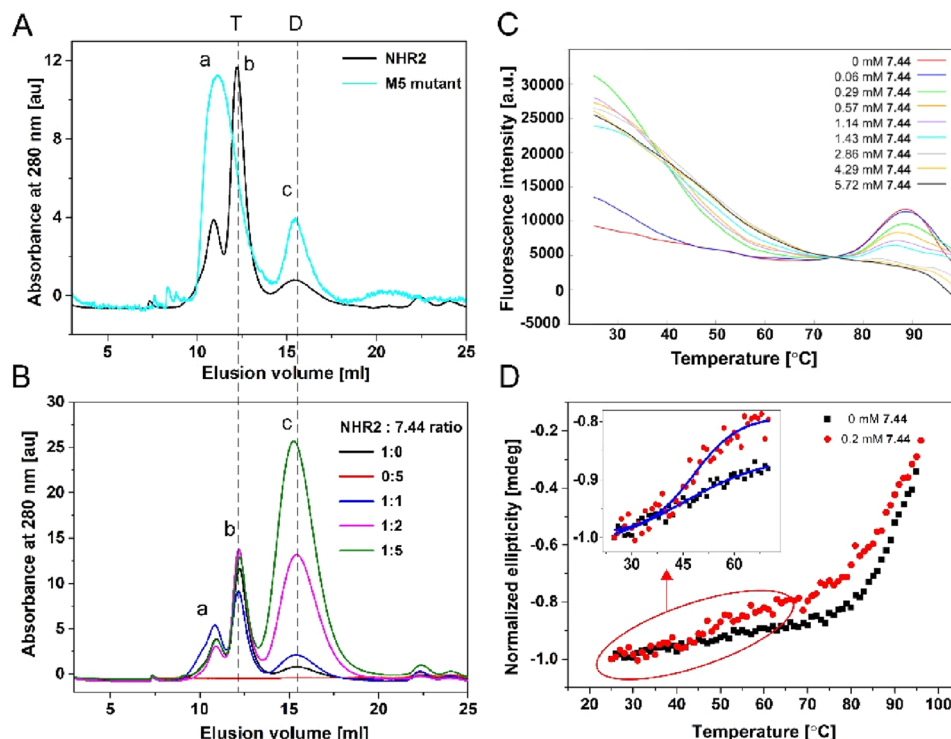
Figure 2. Stability of the NHR2 tetramer with and without 7.44 studied by size exclusion chromatography, DSE, and CD spectroscopy. (A) Elution profiles of purified proteins of the NHR2 domain (black) and M5 variant (cyan) from size exclusion chromatography (SEC) obtained at 280 nm absorbance: higher-order oligomers (a), tetramer (b), and dimer (c). The integration of peaks (b) and (c) of the NHR2 domain yields 92% of the tetramer and 8% of the dimer. (B) Elution profiles of 30 \mu M of apo NHR2 (black), 150 \mu M of 7.44, and NHR2:7.44 with molar ratios of 1:1 (blue), 1:2 (magenta), and 1:5 (green) obtained from SEC at 280 nm. Samples were incubated at 37 ^{\circ} C for 2 h and then incubated overnight at room temperature prior to the experiment. (C) Fluorescence intensity in the presence of 7.44 at different concentrations; for better visualization, the curves were shifted along the y-axis to match them at the point between the two melting points of dimer and tetramer. (D) Thermal denaturation of apo NHR2 (black) and NHR2 in the presence of 7.44 (red) monitored by CD spectroscopy at 222 nm wavelength. The CD data was normalized with respect to the highest ellipticity for better comparison.
