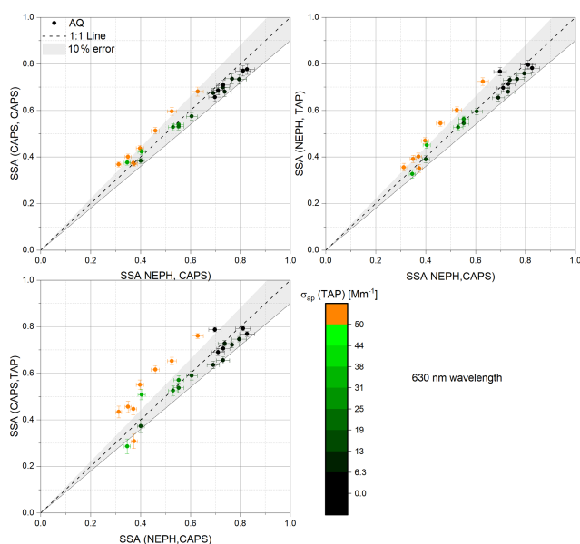
Figure 7. Scatter plots of derived SSA values from various combinations of measurements at 630 nm wavelength obtained for AQ–AS mixtures ( y axis) versus \text{SSA}(\text{NEPH, CAPS}) as the reference on the x axis. The colour code indicates \sigma_{\text{ap}}(\text{TAP}) values shown in inverse megametres ( \text{Mm}^{-1} ).
