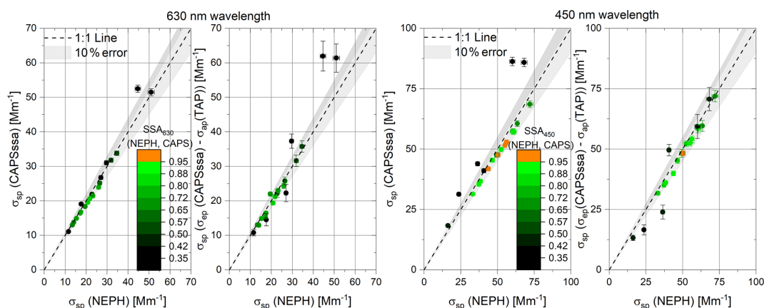
Figure 4. Comparisons of measured light-scattering coefficients at 450 and 630 nm wavelengths for mixtures of AQ and AS aerosols. The y axes show the CAPS PM SSA (integrating sphere) or the differential method (CAPS extinction minus TAP absorption) scattering versus NEPH scattering measurements at 450 and 630 nm wavelengths. The colour code represents the SSA value of the measured aerosol mixture. An error band of \pm 10\% was applied to the 1 : 1 line. Error bars shown represent instrument precisions ( 1\sigma ).
