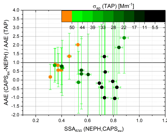
Figure 14. The absorbing Ångström exponent ratio, \text{AAE}(\text{CAPS, NEPH})/\text{AAE}(\text{TAP}) , as a function of 630 nm wavelength \text{SSA}(\text{NEPH, CAPS}) values for AQ–AS mixtures. The 630 nm wavelength light-absorption coefficient, \sigma_{\text{ap}} (TAP), is used as the colour code. Measured precision error bars are shown for individual measurements.
