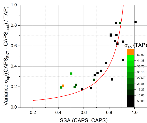
Figure 6. Variance of the measured absorption coefficients ( \sigma_{\text{ap}} (CAPS, CAPS)/ \sigma_{\text{ap}} (TAP)) for differential method calculations relative to TAP measurements for AQ and AS external mixtures. The ratios are plotted against the aerosol measured SSA values (SSA(CAPS, CAPS)). The red line represents the calculated relative errors using Gaussian error propagation of the uncertainties in the DM with 1 as 100 %.
