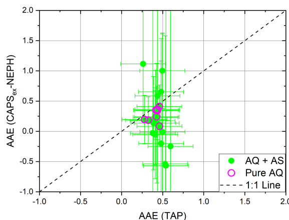
Figure 13. Scatter plot of AAE(CAPS, NEPH) measurements compared to AAE(TAP) measurements for pure AQ and AQ–AS external mixtures. Measured precision error bars are shown for individual externally mixed AQ–AS measurements.
