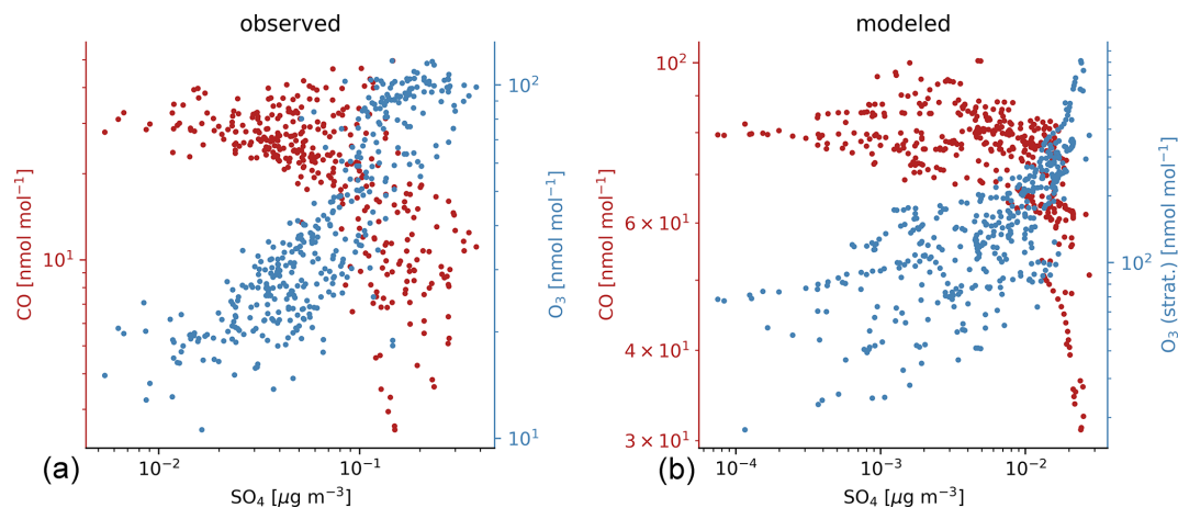
Figure 4. Scatter plot of co-located \text{SO}_4 , CO (red), and \text{O}_3 (blue) abundance between 350 and 150 hPa from observations (a) and the RED simulation (b).
