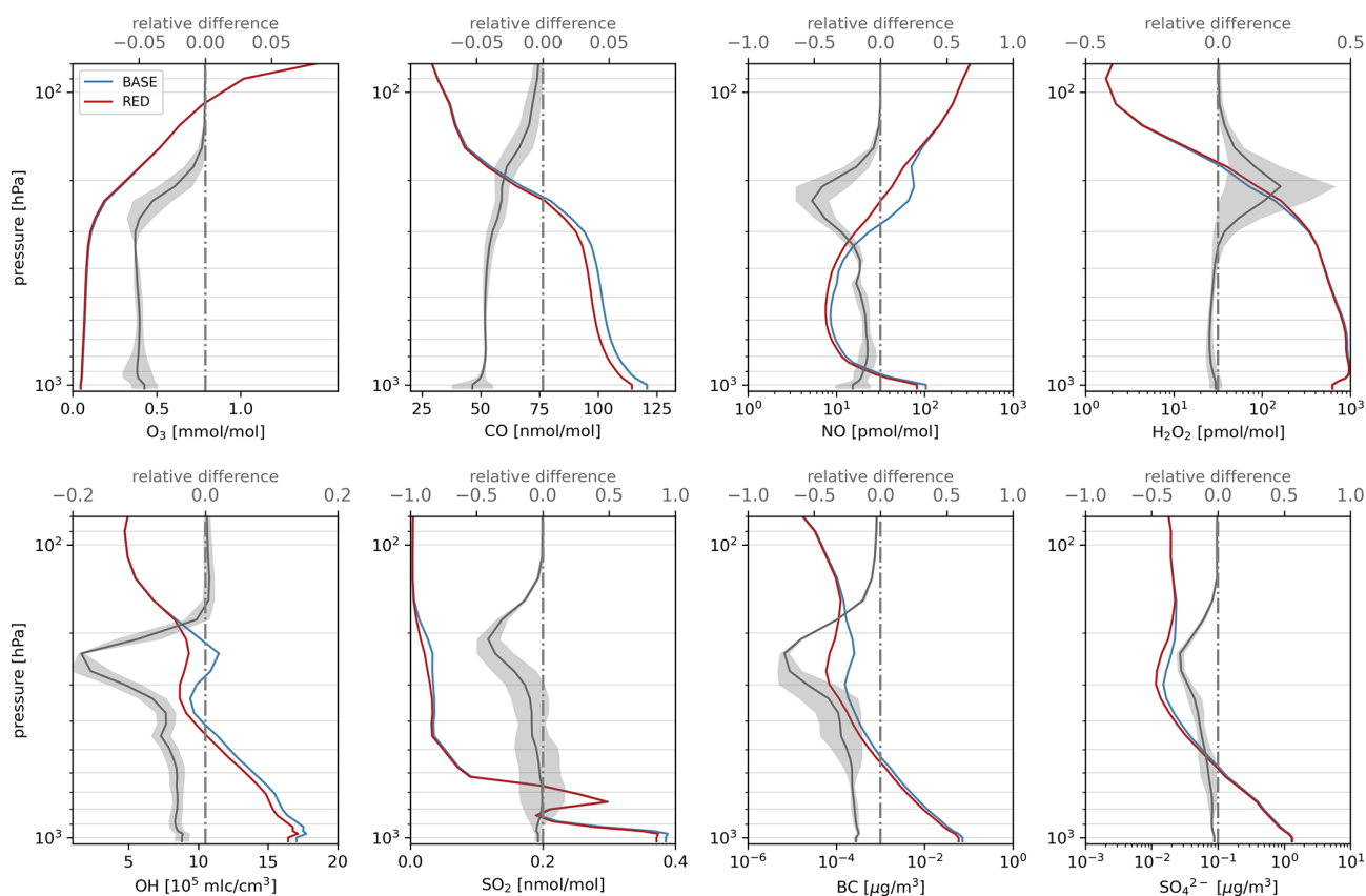
Figure 5. Vertical profiles from BASE and RED simulations and their relative difference ((\text{RED} - \text{BASE})/\text{BASE}) . The grey area represents 1 standard deviation of the spatial-temporal mean (grey line). Please note the different scales for the relative differences.
