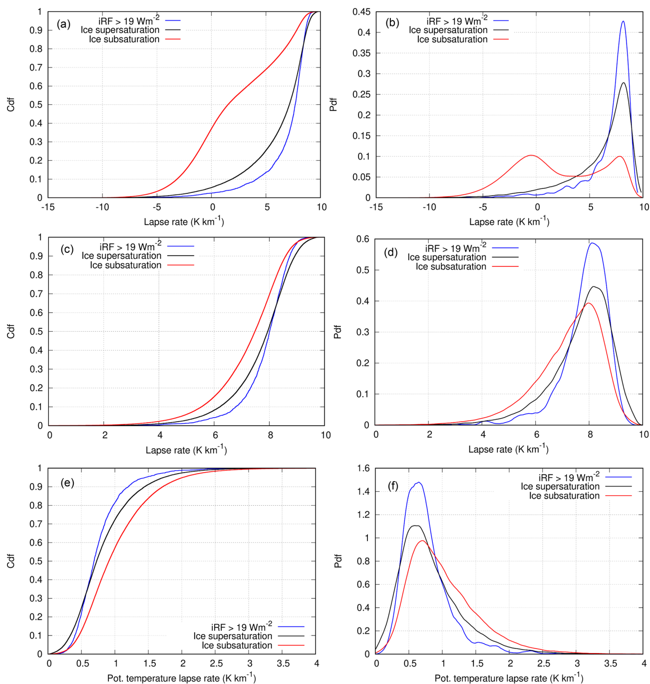
Figure 1. (a) Cumulative distribution function of lapse rates, -dT/dh , for ice-subsaturated (red) and ice-supersaturated air masses. (b) Probability densities for the same lapse rate distributions. The middle panels show the lapse rate distributions (c) and probability densities (d) excluding stratospheric cases; that is, the upper pressure level of each event has PV \leq 2 PVU. Please note the different \gamma ranges plotted in the upper and middle panels. Panels (e) and (f) show the corresponding troposphere-only distributions (e) and probability densities (f) for potential temperature gradients.
