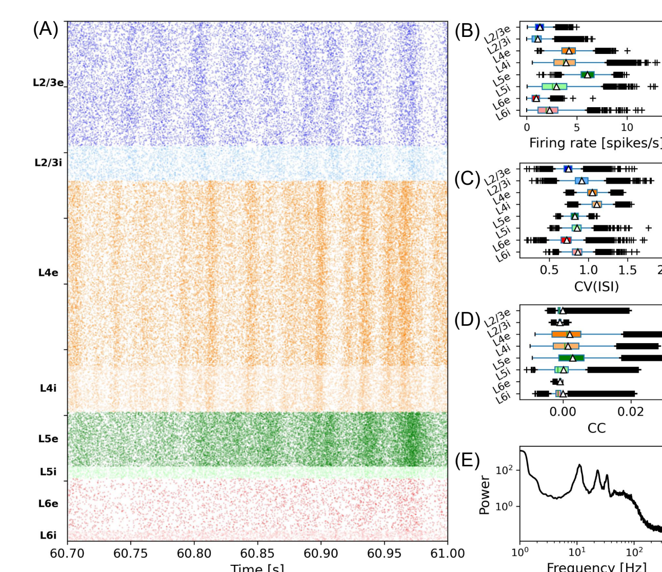
Figure 5. Network activity of the thalamocortical network. Thalamocortical and corticothalamic delays were set to 30 and 50 ms respectively. A) raster plot; B) firing rates; C) coefficient of variation of the interspike intervals; D) correlation coefficient; and E) power spectrum calculated from network activity. Each color represents a different population.
