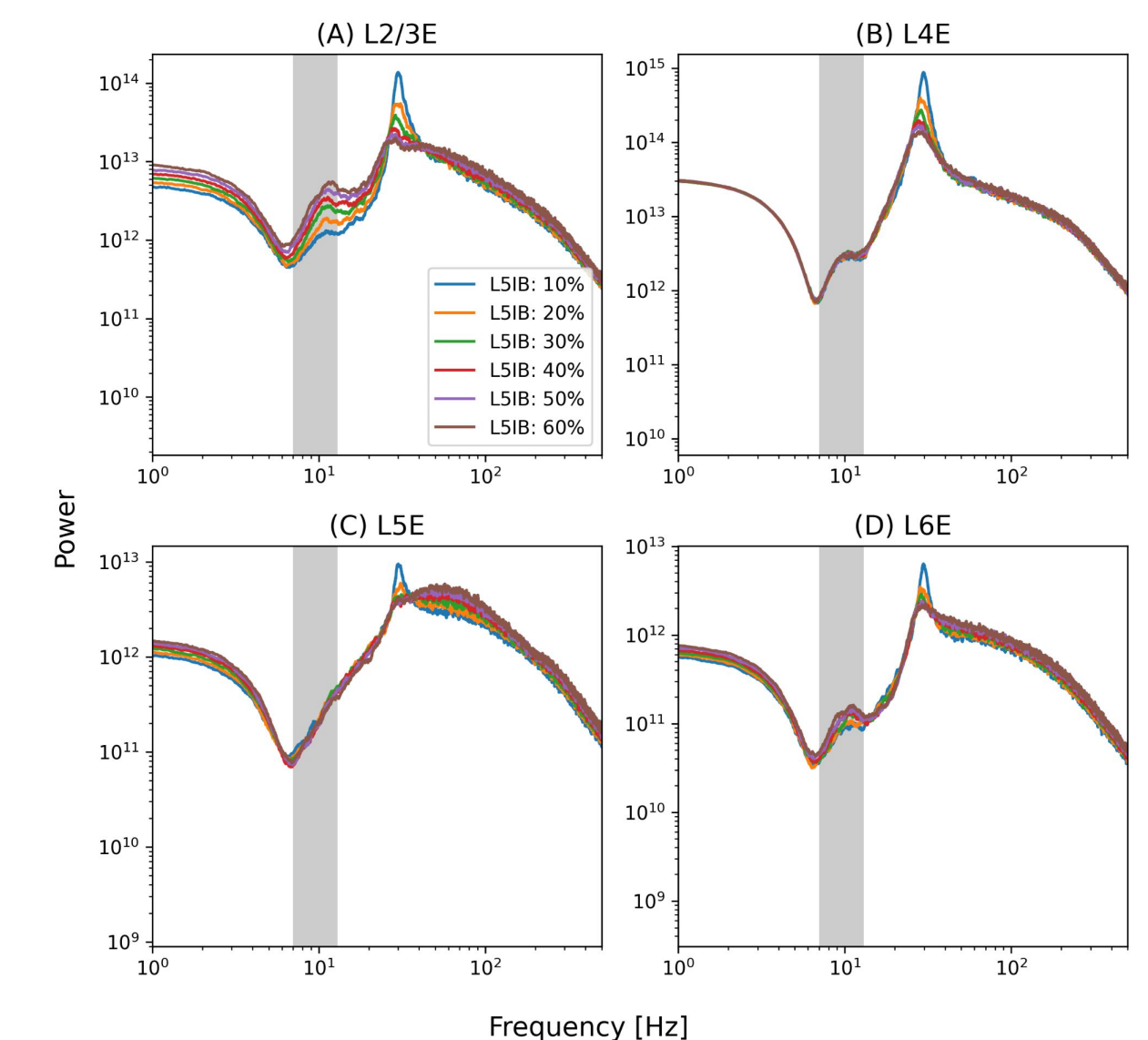
Figure 4. Power spectra estimated using CSD proxy from network activity by layer for different proportions of IB to RS neurons at L5 (10 to 60 of the total L5 excitatory neurons). The shaded area represents the alpha range.
