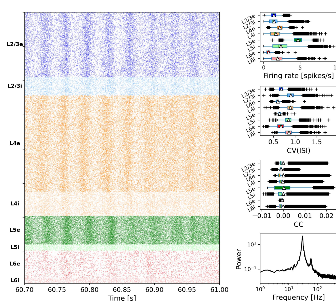
Figure 2. Network activity of the isolated V1 microcircuit. A) raster plot; B) firing rates; C) coefficient of variation of the interspike intervals; D) correlation coefficient; and E) power spectrum calculated from network activity. Each color represents a different population.
