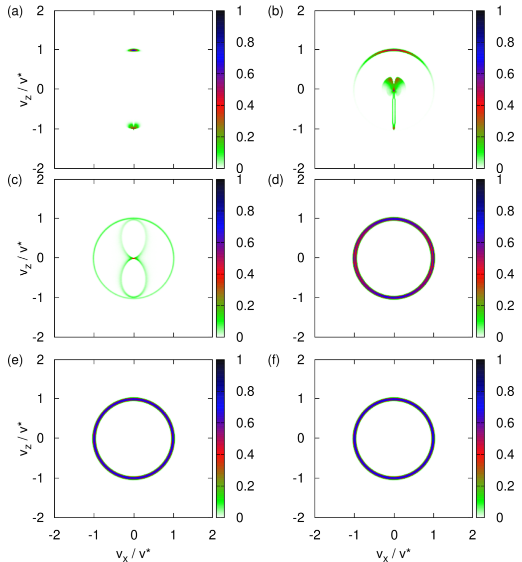
Figure 11. Histograms of the transverse velocity distribution obtained by event-by-event simulation. The classical equations of motion (Equation (3)) are modified to include a one-time projection of the spin vector \mathbf{S} along the direction of the magnetic field using the procedure described in the text. The initial magnetic moments of the particles are distributed randomly. The variance of the transverse velocity \sigma_v = 0.014v^* . (a) B_0 = 1 T; (b) B_0 = 0.1 T; (c) B_0 = 0.01 T; (d) B_0 = 0.001 T; (e) B_0 = 0.0001 T; (f) B_0 = 0.00001 T.
