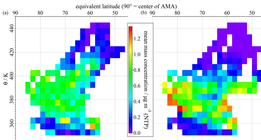
Figure 4. Curtain plot of (a) organic and (b) nitrate mass concentration as a function of \theta and equivalent latitude (AMA-centered). The values for organics are based on the data from the Flights 1, and 4 through 8.
